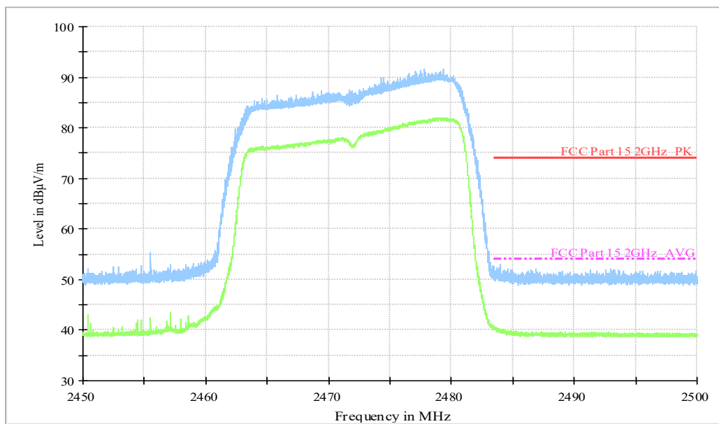
Fig.A.6.2.15 Transmitter Spurious Emission - Radiated (Power): 802.11n-HT20, ch13, 2.45 GHz - 2.50GHz
