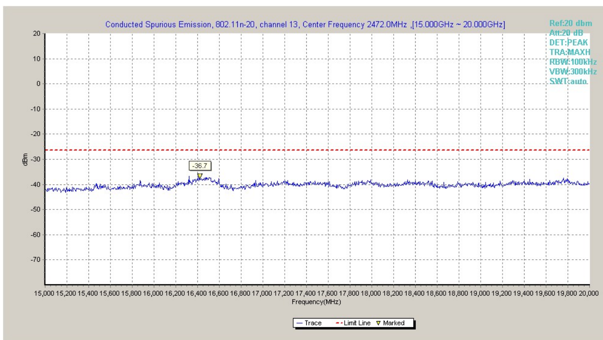
Fig.A.6.1.119 Transmitter Spurious Emission - Conducted (802.11n-HT20, Ch13, 15 GHz-20 GHz)
