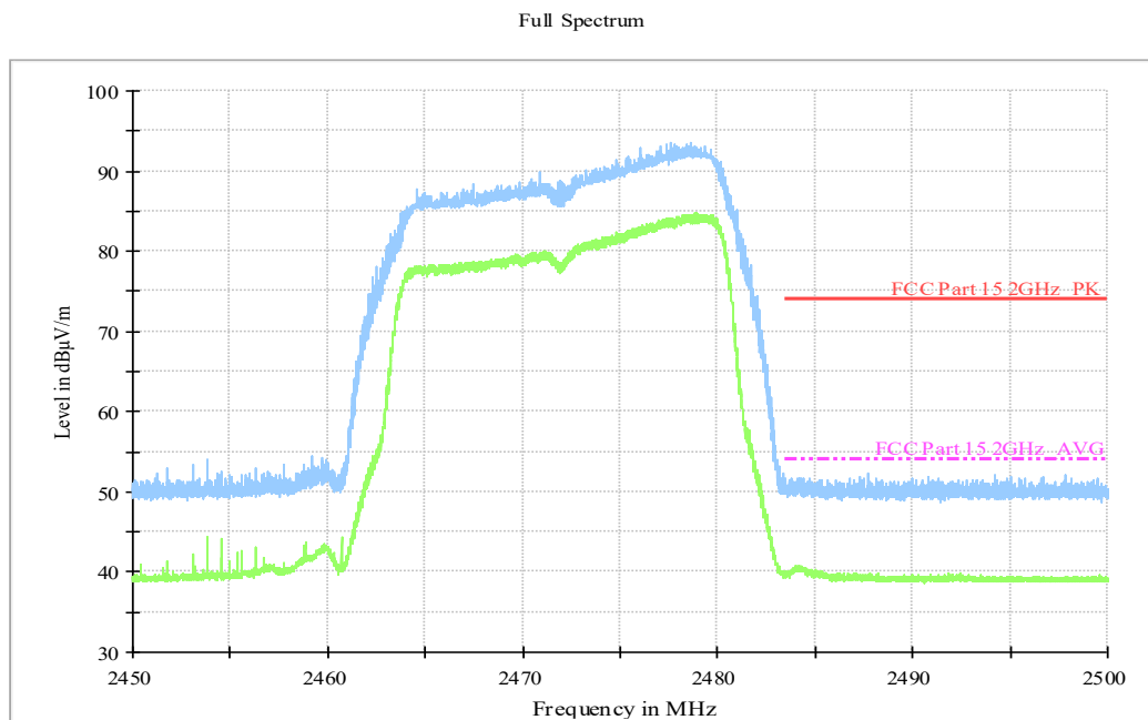
Fig.A.6.2.10 Transmitter Spurious Emission - Radiated (Power): 802.11g, ch13, 2.45 GHz - 2.50GHz
