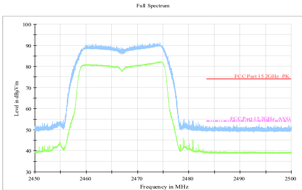
Fig.A.6.2.9 Transmitter Spurious Emission - Radiated (Power): 802.11g, ch12, 2.45 GHz - 2.50GHz
