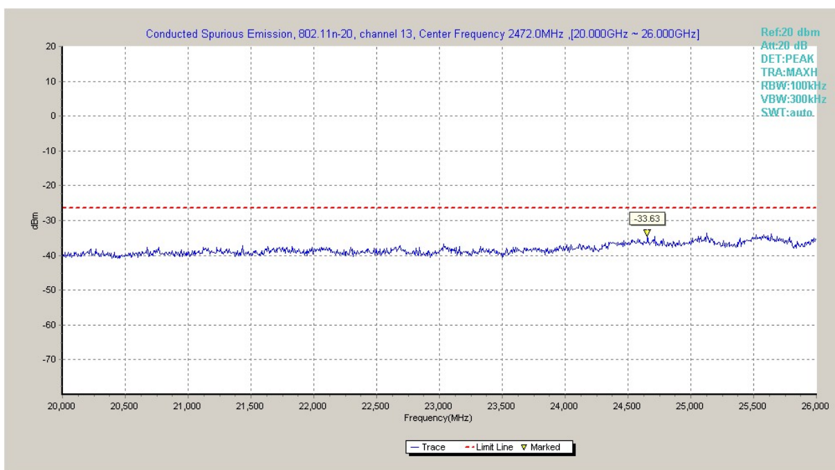
Fig.A.6.1.120 Transmitter Spurious Emission - Conducted (802.11n-HT20, Ch13, 20 GHz-26 GHz)
