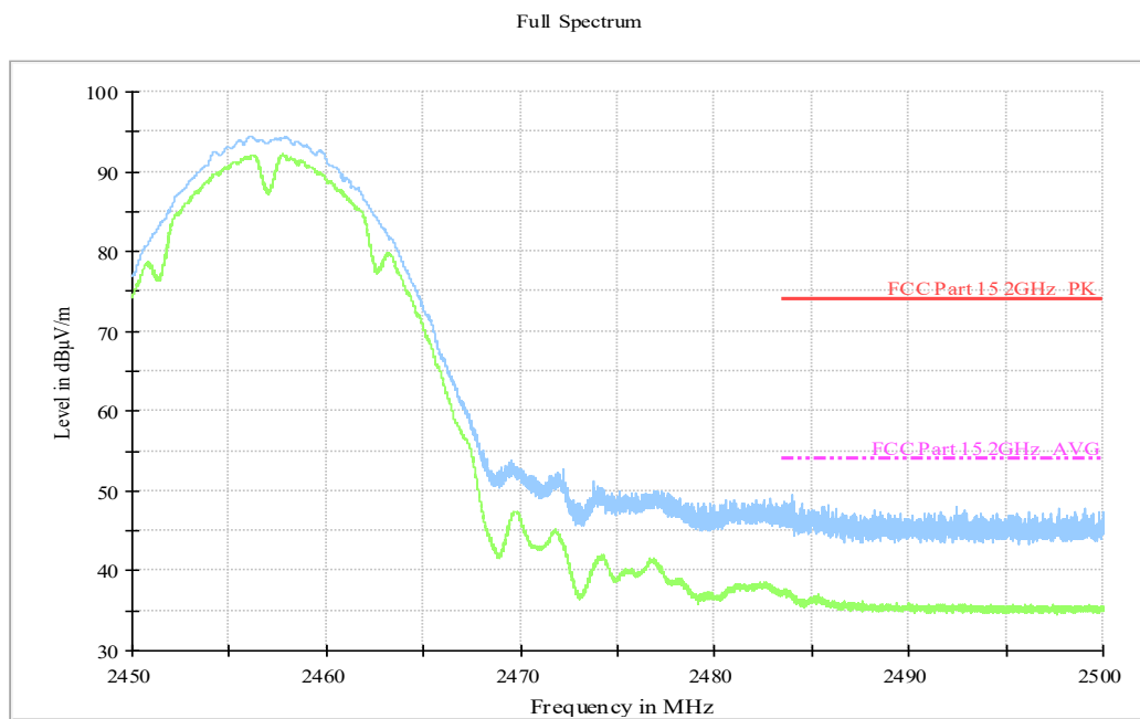
Fig.A.6.2.3 Transmitter Spurious Emission - Radiated (Power): 802.11b, ch10, 2.45 GHz - 2.50GHz
