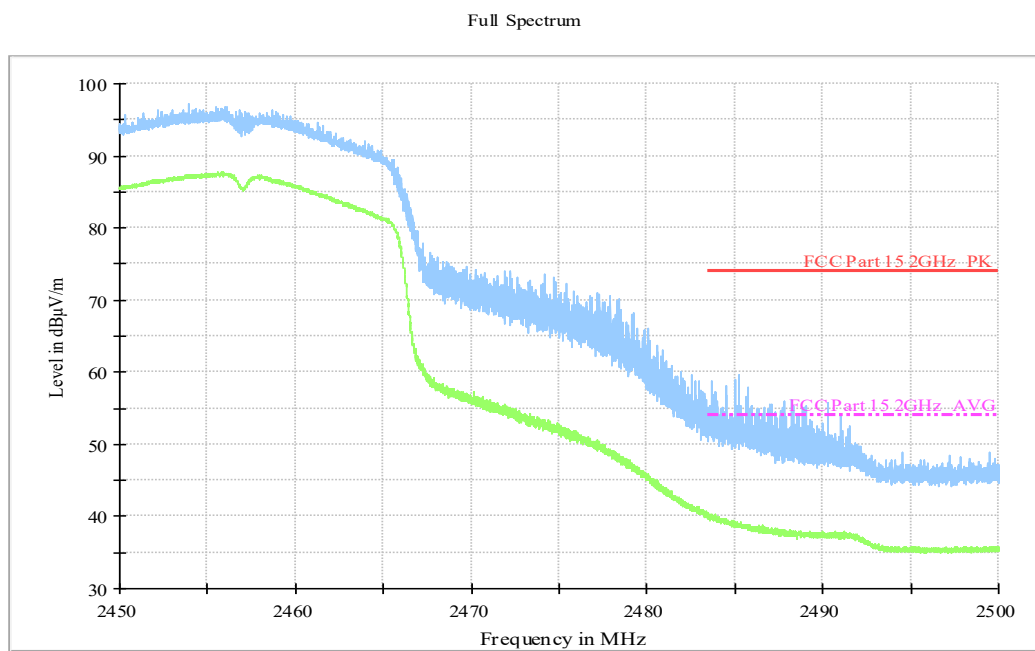
Fig.A.6.2.13 Transmitter Spurious Emission - Radiated (Power): 802.11n-HT20, ch10, 2.45 GHz - 2.50GHz
