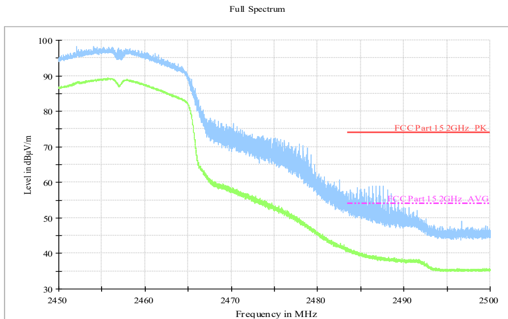
Fig.A.6.2.8 Transmitter Spurious Emission - Radiated (Power): 802.11g, ch10, 2.45 GHz - 2.50GHz
