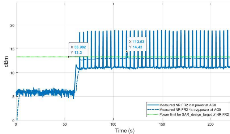
Figure 12.4-1 Radiated EIRP of FR2 n261 in TC22
