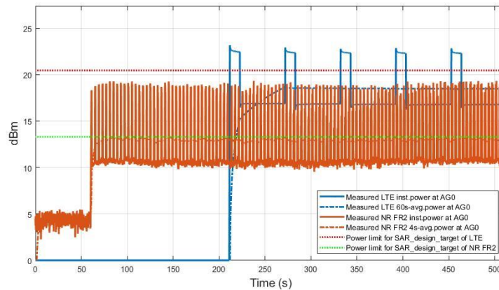
Figure 12.2-6-1 Conducted power of LTE B2 and radiated EIRP of FR2 n261 in TC18 EN-DC
