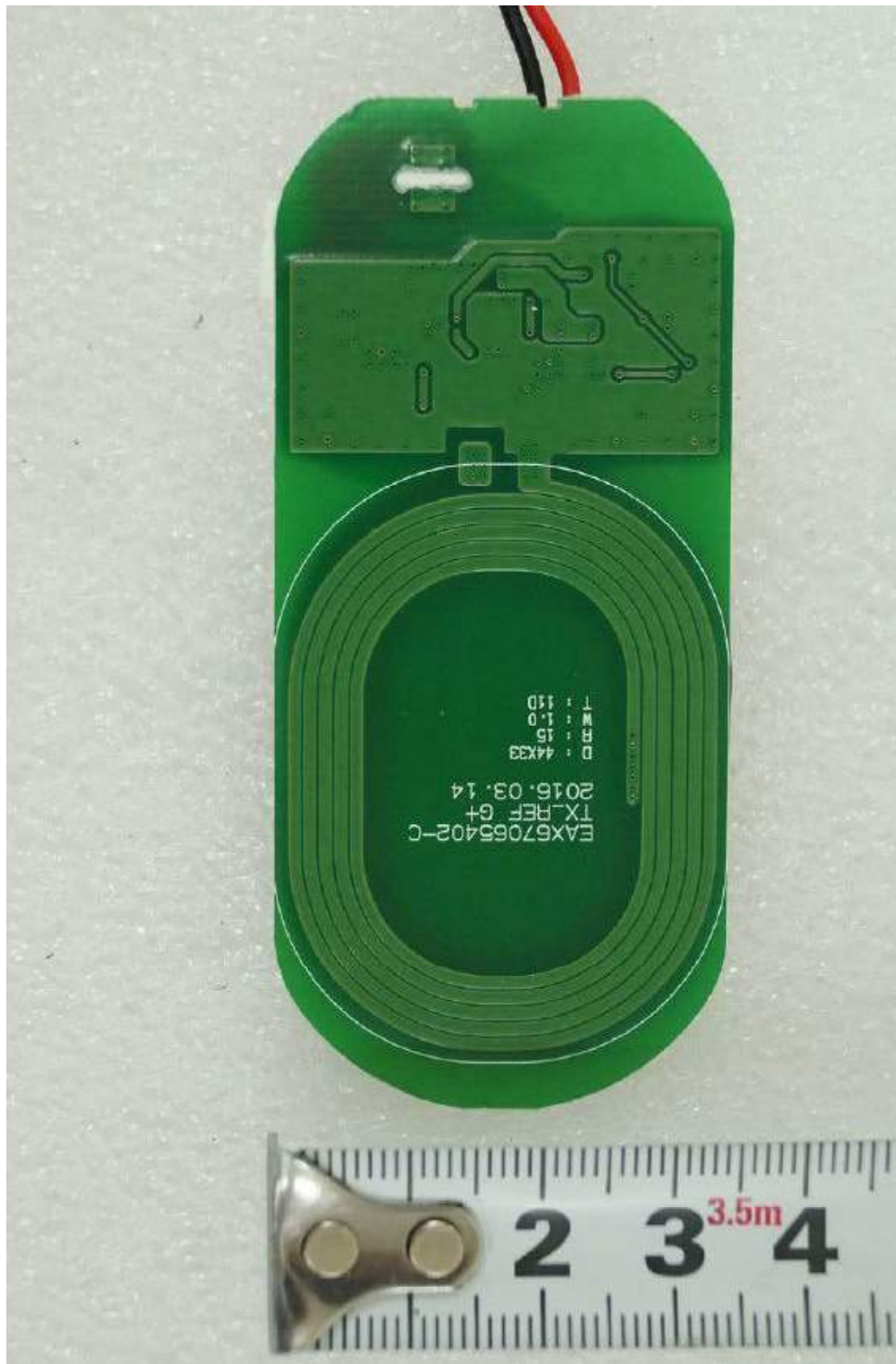
<OLD Wireless shelf module -3>
