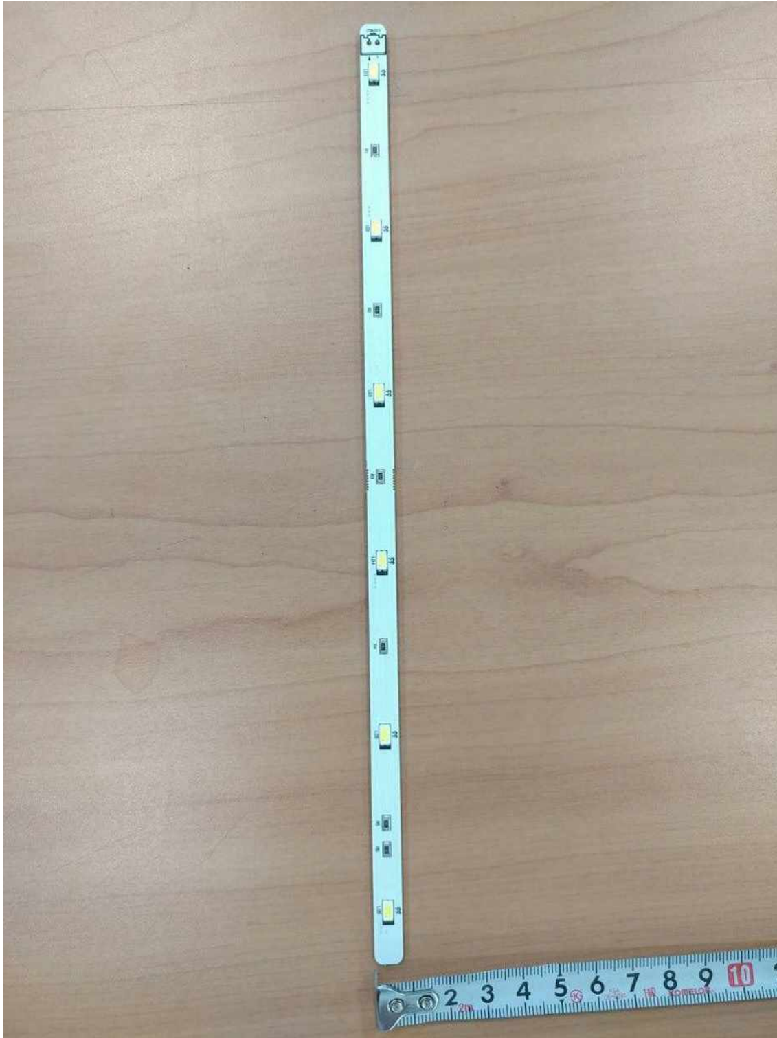
<Top LED -2>
