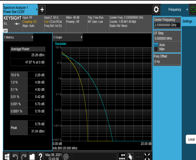
Band7-20MHz-QPSK-21100-100RB#0
