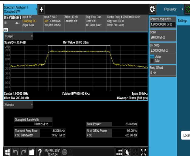
Band2-10MHz-16QAM-19150-50RB#0
