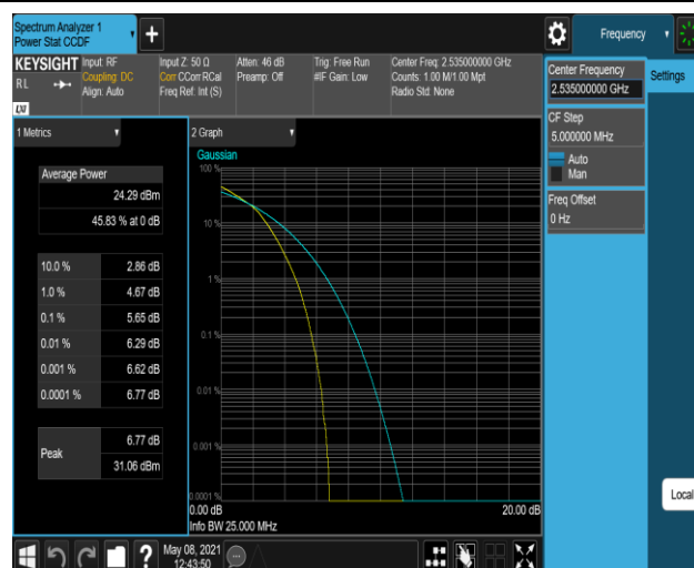
Band7-20MHz-16QAM-21100-100RB#0
