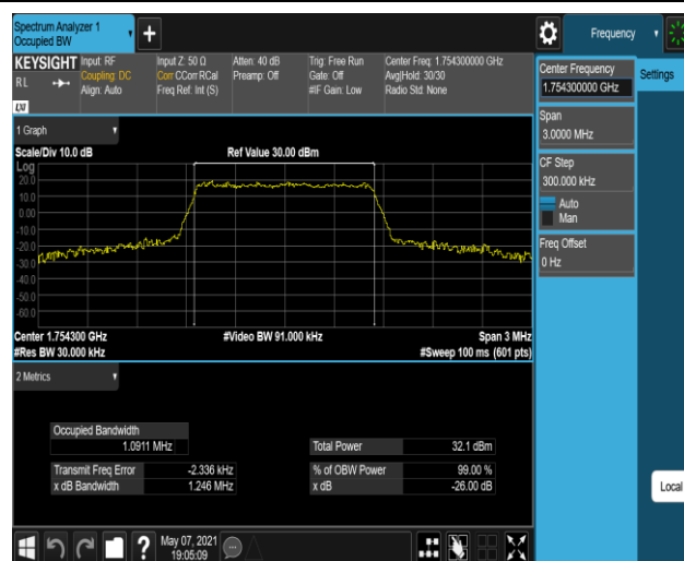
Band4-1.4MHz-16QAM-20393-6RB#0
