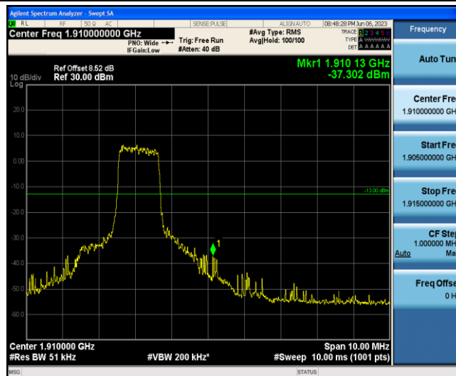
Band2-20MHz-16QAM-19100-6-0-High--37.30-PASS
