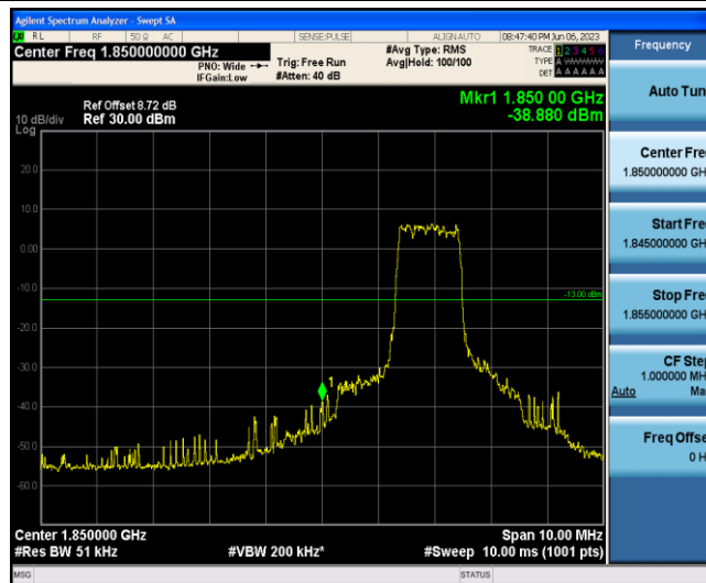
Band2-20MHz-16QAM-18700-6-0-Low--38.88-PASS
