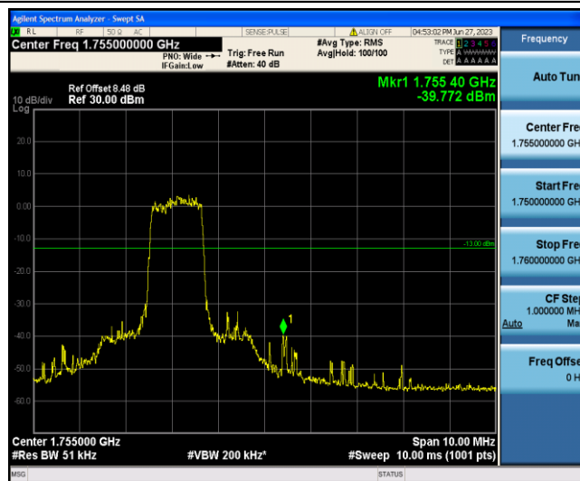
Band4-20MHz-QPSK-20300-6-0-High--39.77-PASS
