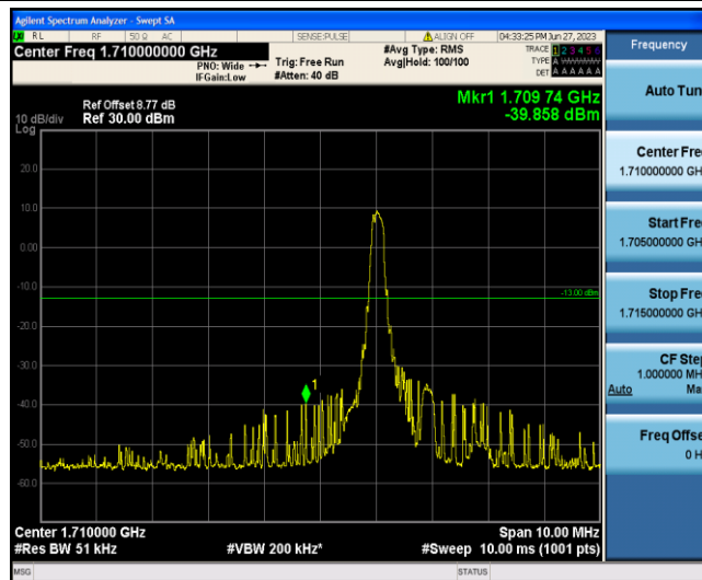
Band4-15MHz-16QAM-20025-1-0-Low--39.86-PASS
