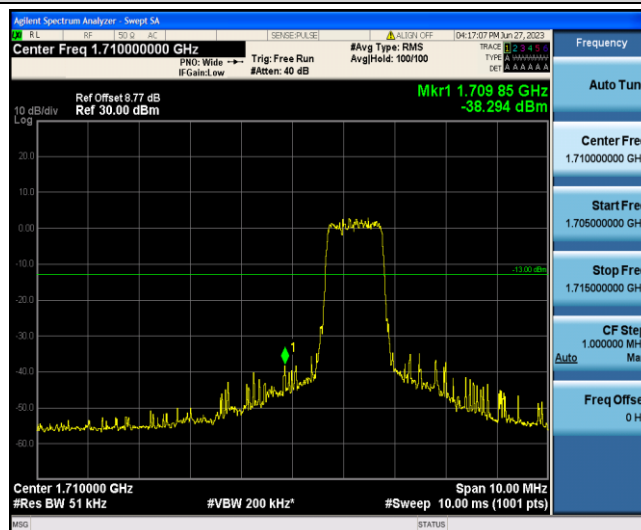
Band4-10MHz-16QAM-20000-6-0-Low--38.29-PASS
