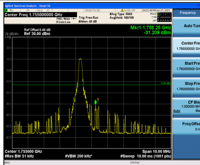
Band4-5MHz-QPSK-20375-1-5-High--31.21-PASS
