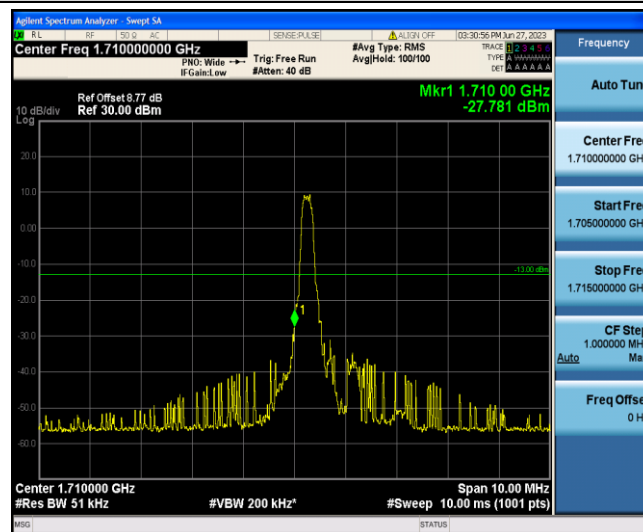
Band4-1.4MHz-16QAM-19957-1-0-Low--27.78-PASS
