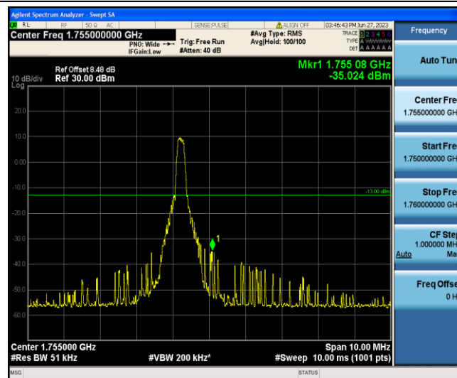
Band4-3MHz-QPSK-20385-1-5-High--35.02-PASS
