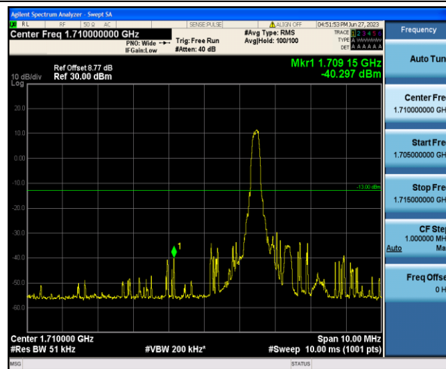
Band4-20MHz-QPSK-20050-1-0-Low--40.30-PASS
