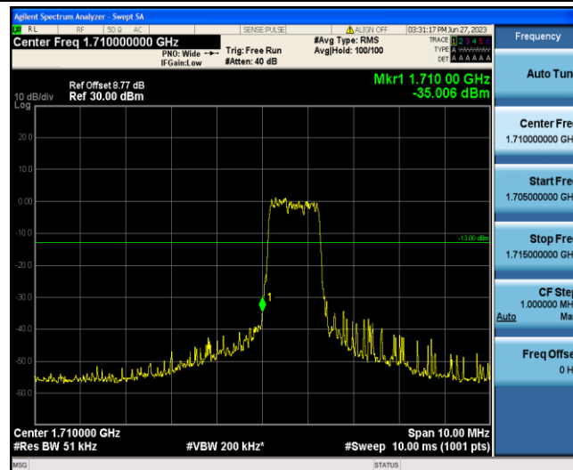
Band4-1.4MHz-16QAM-19957-6-0-Low--35.01-PASS
