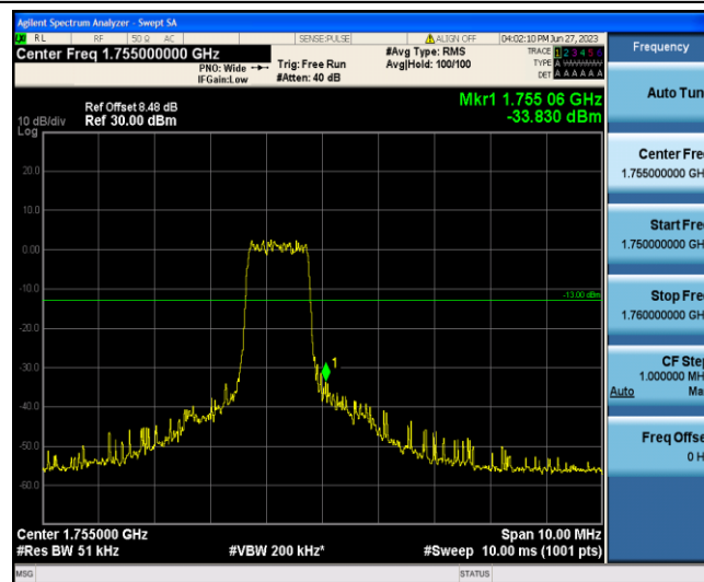
Band4-5MHz-QPSK-20375-6-0-High--33.83-PASS
