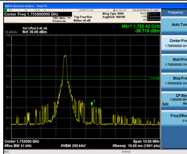
Band4-15MHz-QPSK-20325-1-5-High--38.72-PASS
