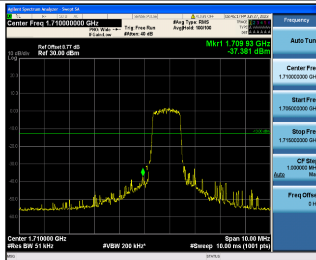
Band4-3MHz-QPSK-19965-6-0-Low--37.38-PASS
