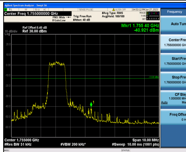
Band4-20MHz-16QAM-20300-6-0-High--40.92-PASS
