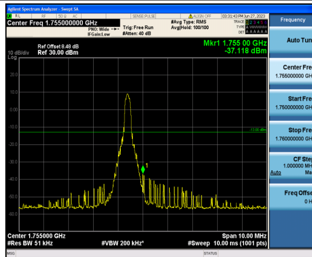
Band4-1.4MHz-16QAM-20393-1-5-High--37.12-PASS
