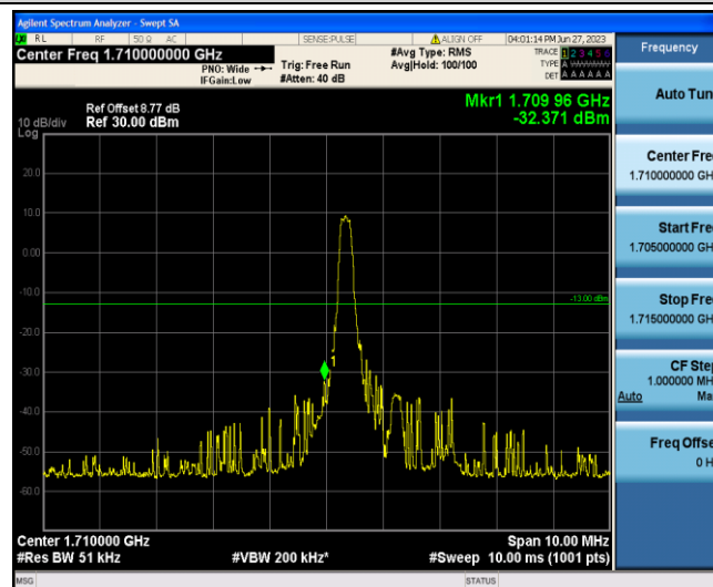
Band4-5MHz-16QAM-19975-1-0-Low--32.37-PASS
