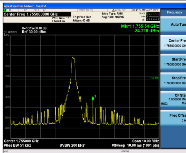
Band4-3MHz-16QAM-20385-1-5-High--34.22-PASS
