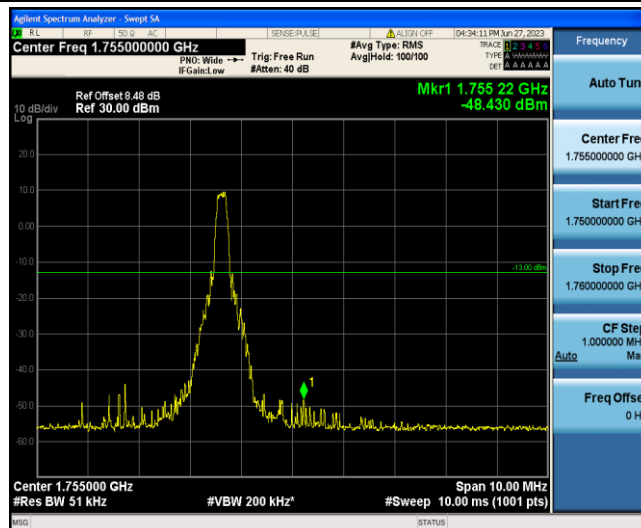
Band4-15MHz-16QAM-20325-1-5-High--48.43-PASS
