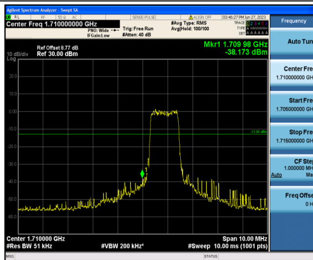
Band4-3MHz-16QAM-19965-6-0-Low--38.17-PASS
