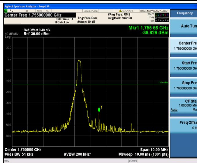
Band4-5MHz-16QAM-20375-1-5-High--38.93-PASS
