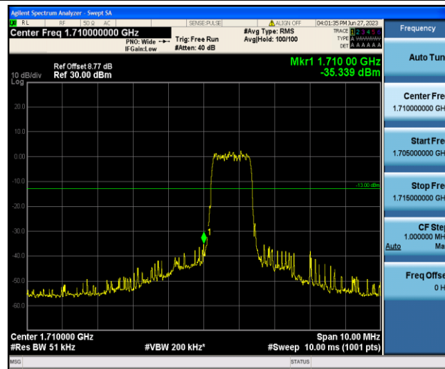
Band4-5MHz-16QAM-19975-6-0-Low--35.34-PASS
