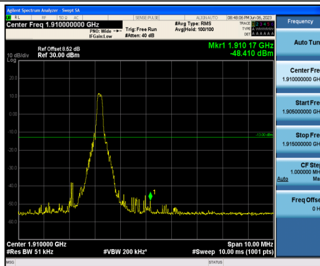
Band2-20MHz-16QAM-19100-1-5-High--48.41-PASS
