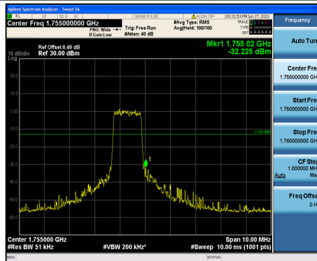
Band4-1.4MHz-QPSK-20393-6-0-High--32.23-PASS
