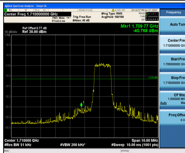
Band4-10MHz-QPSK-20000-6-0-Low--40.77-PASS
