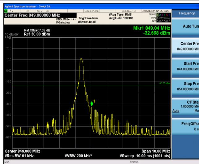
Band5-1.4MHz-QPSK-20643-1-5-High--32.57-PASS
