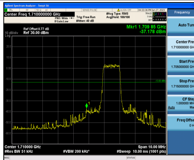
Band4-15MHz-QPSK-20025-6-0-Low--37.18-PASS
