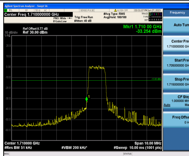
Band4-1.4MHz-QPSK-19957-6-0-Low--33.25-PASS
