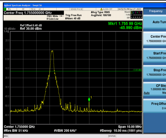
Band4-20MHz-16QAM-20300-1-5-High--45.99-PASS
