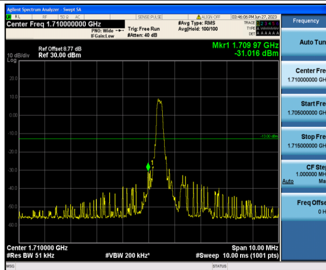
Band4-3MHz-16QAM-19965-1-0-Low--31.02-PASS
