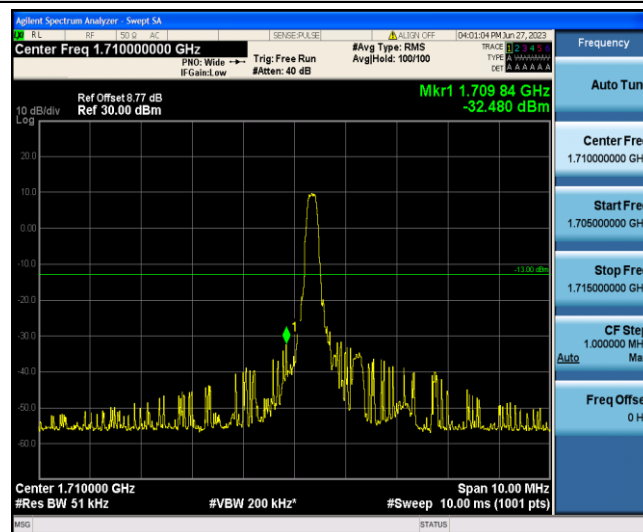
Band4-5MHz-QPSK-19975-1-0-Low--32.48-PASS
