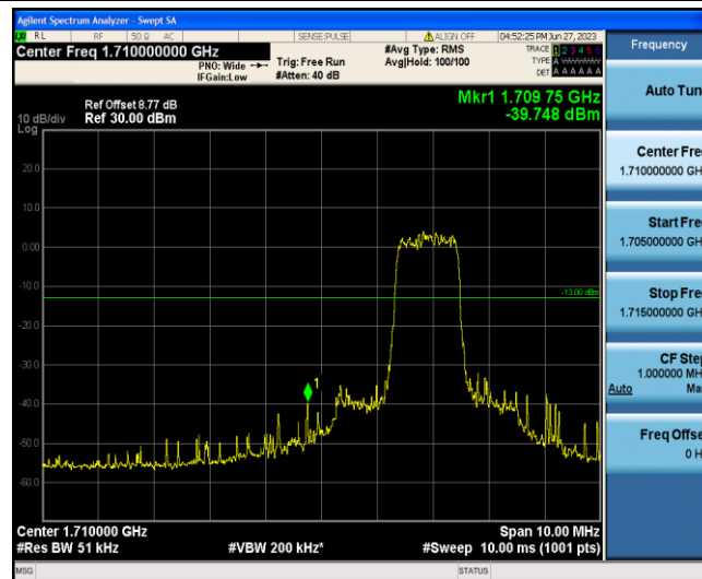
Band4-20MHz-16QAM-20050-6-0-Low--39.75-PASS
