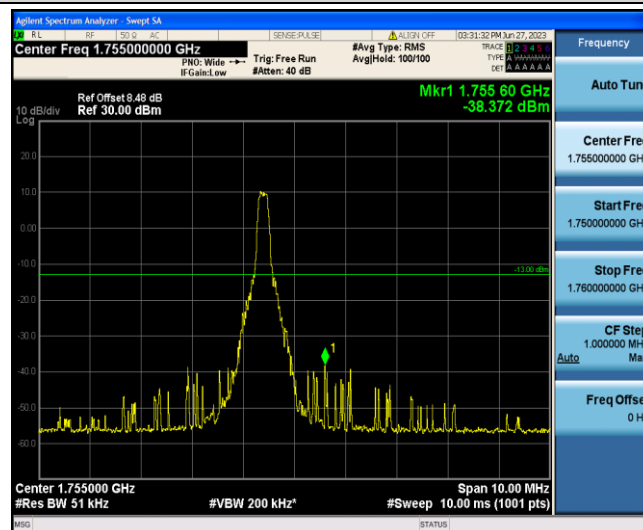
Band4-1.4MHz-QPSK-20393-1-5-High--38.37-PASS
