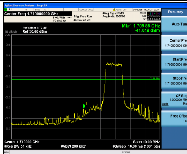
Band4-20MHz-QPSK-20050-6-0-Low--41.05-PASS
