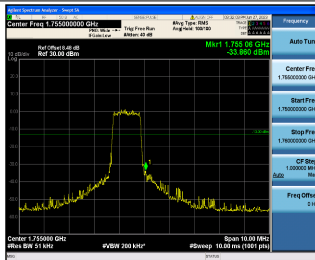
Band4-1.4MHz-16QAM-20393-6-0-High--33.86-PASS
