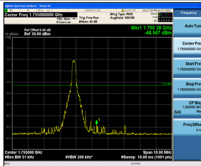
Band4-10MHz-16QAM-20350-1-5-High--48.57-PASS
