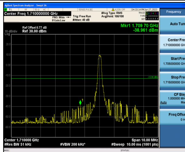
Band4-15MHz-QPSK-20025-1-0-Low--38.96-PASS
