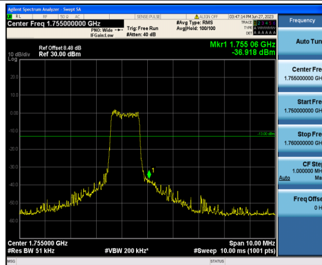
Band4-3MHz-16QAM-20385-6-0-High--36.92-PASS
