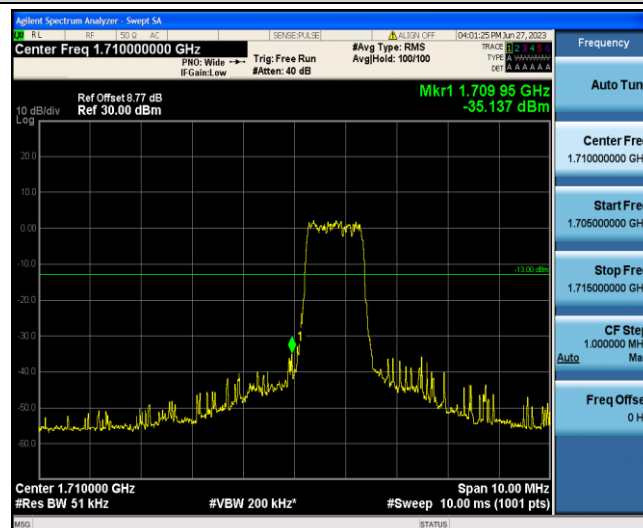
Band4-5MHz-QPSK-19975-6-0-Low--35.14-PASS
