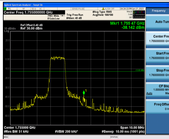
Band4-15MHz-16QAM-20325-6-0-High--38.14-PASS
