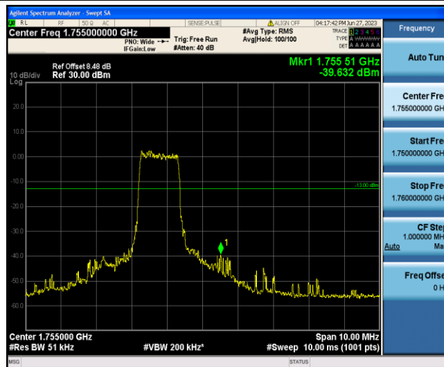
Band4-10MHz-QPSK-20350-6-0-High--39.63-PASS
