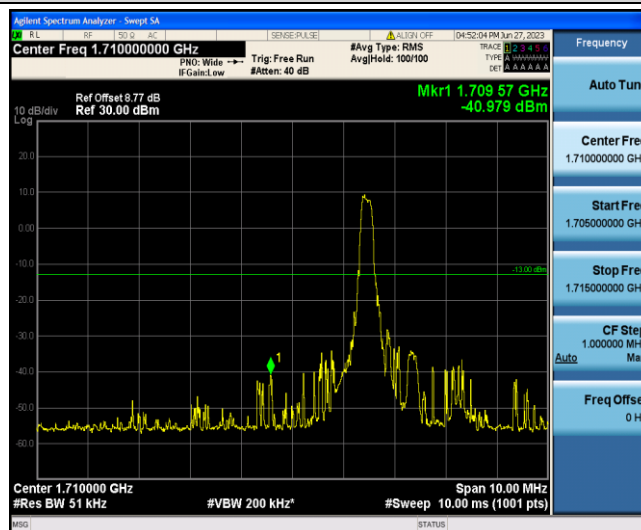
Band4-20MHz-16QAM-20050-1-0-Low--40.98-PASS
