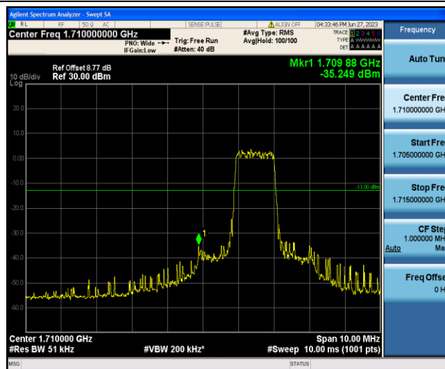
Band4-15MHz-16QAM-20025-6-0-Low--35.25-PASS
