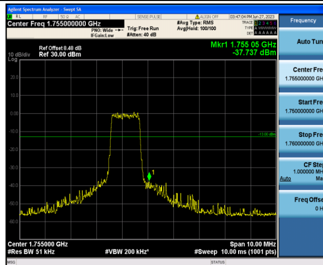
Band4-3MHz-QPSK-20385-6-0-High--37.74-PASS
