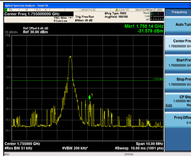
Band4-10MHz-QPSK-20350-1-5-High--31.58-PASS
