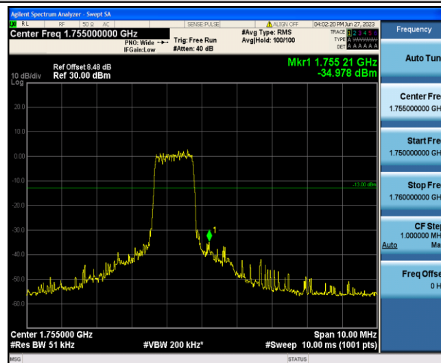
Band4-5MHz-16QAM-20375-6-0-High--34.98-PASS
