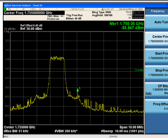
Band4-15MHz-QPSK-20325-6-0-High--35.95-PASS
