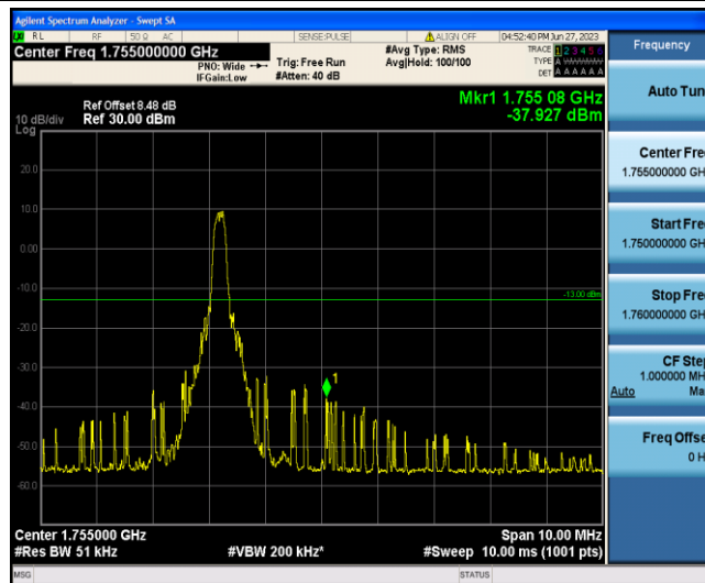
Band4-20MHz-QPSK-20300-1-5-High--37.93-PASS
