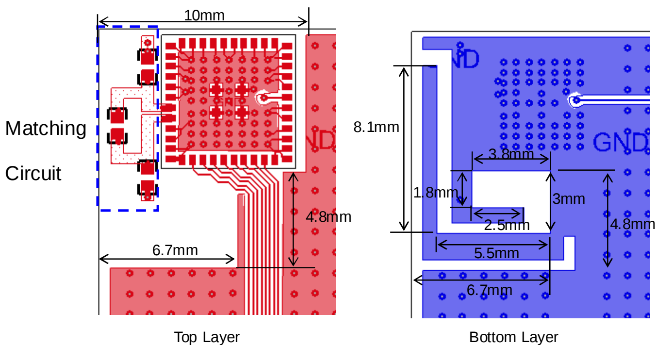
Figure 10-1. Layout Guide
