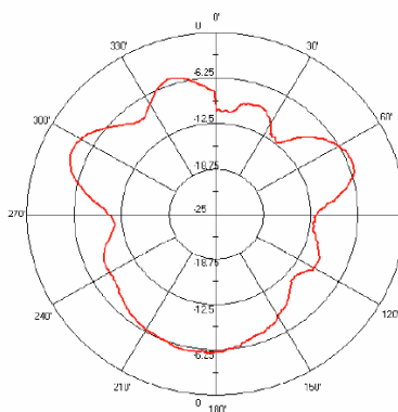
2.4 GHz E-Plane Vertical
