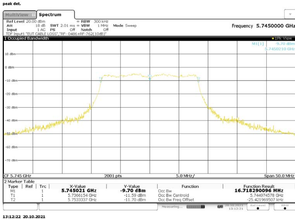
Figure 50: 99% Bandwidth, 802.11a, CDD, RF0, 5745MHz
