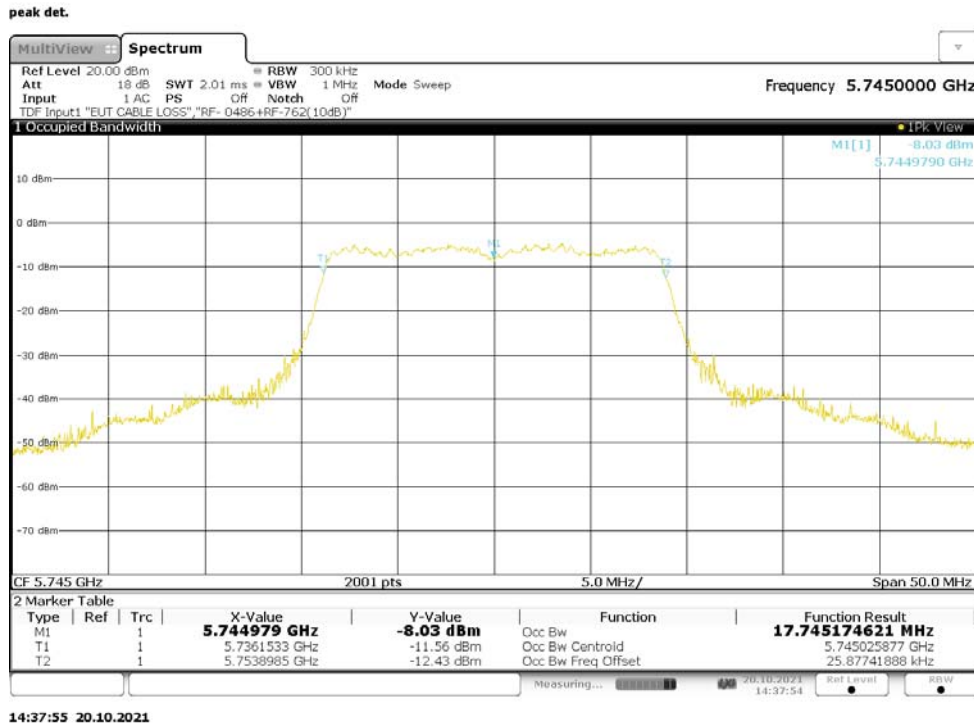
Figure 56: 99% Bandwidth, 802.11n-20, SISO, RF0, 5745MHz
