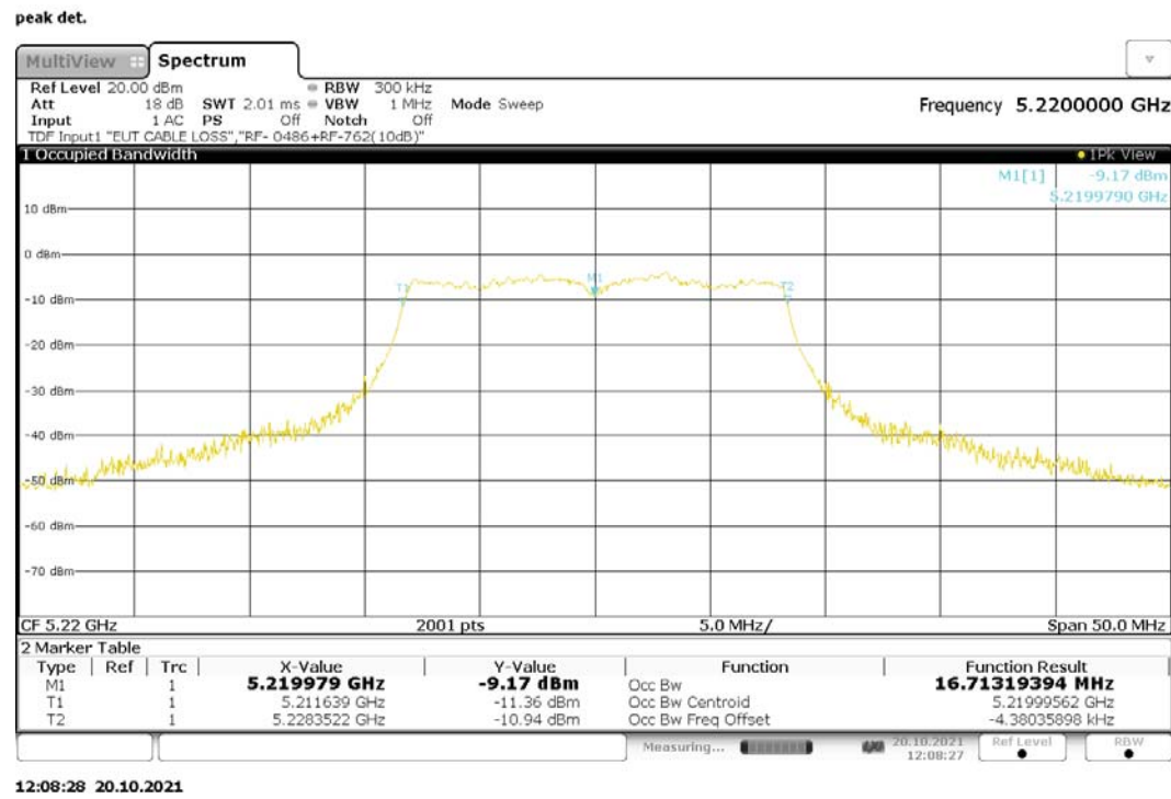
Figure 42: 99% Bandwidth, 802.11a, SISO, RF0, 5220MHz
