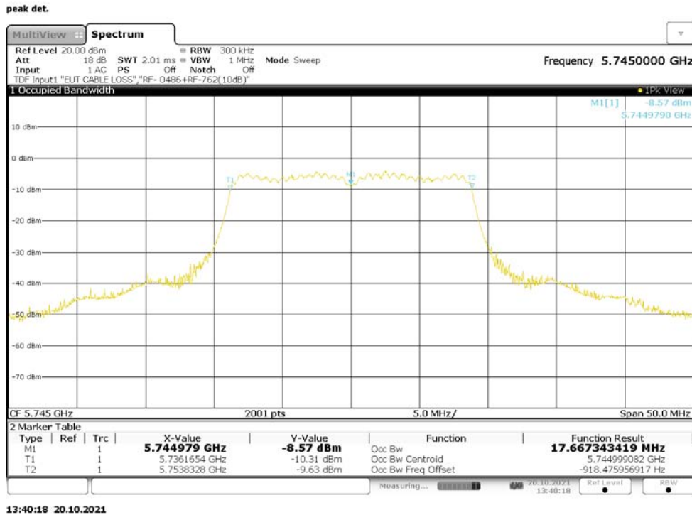
Figure 68: 99% Bandwidth, 802.11n-20, MIMO, RF0, 5745MHz
