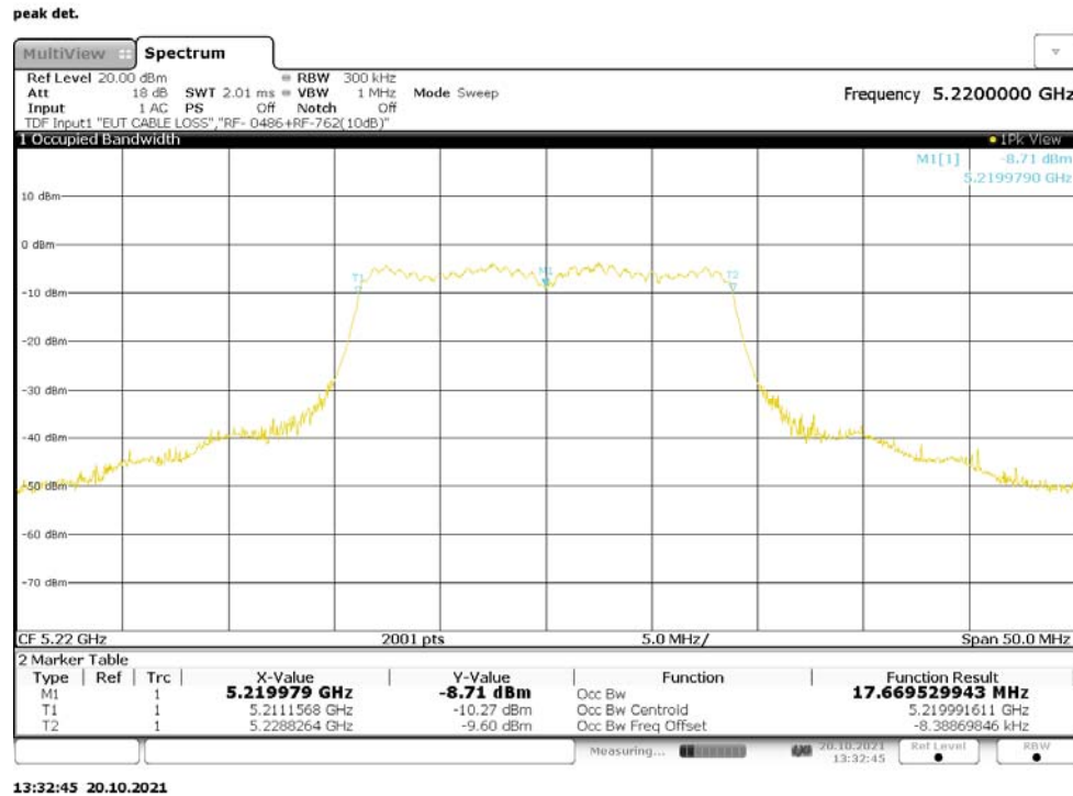
Figure 60: 99% Bandwidth, 802.11n-20, CDD, RF0, 5220MHz
