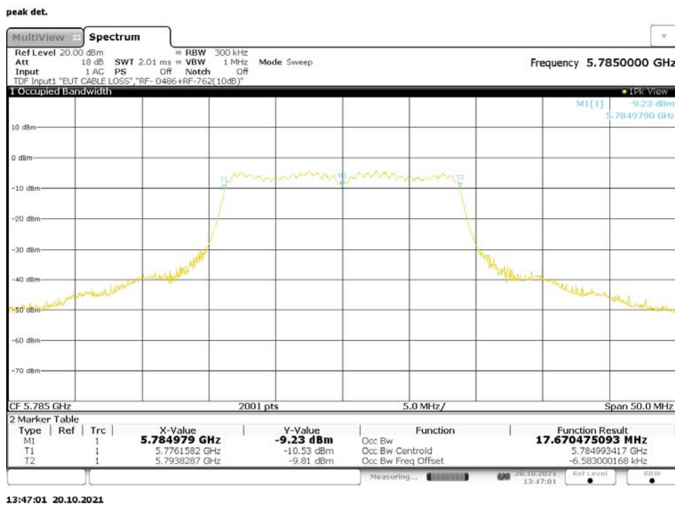
Figure 69: 99% Bandwidth, 802.11n-20, MIMO, RF0, 5785MHz
