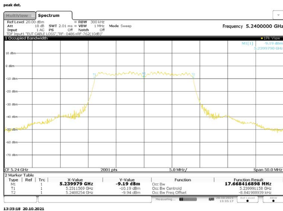
Figure 61: 99% Bandwidth, 802.11n-20, CDD, RF0, 5240MHz
