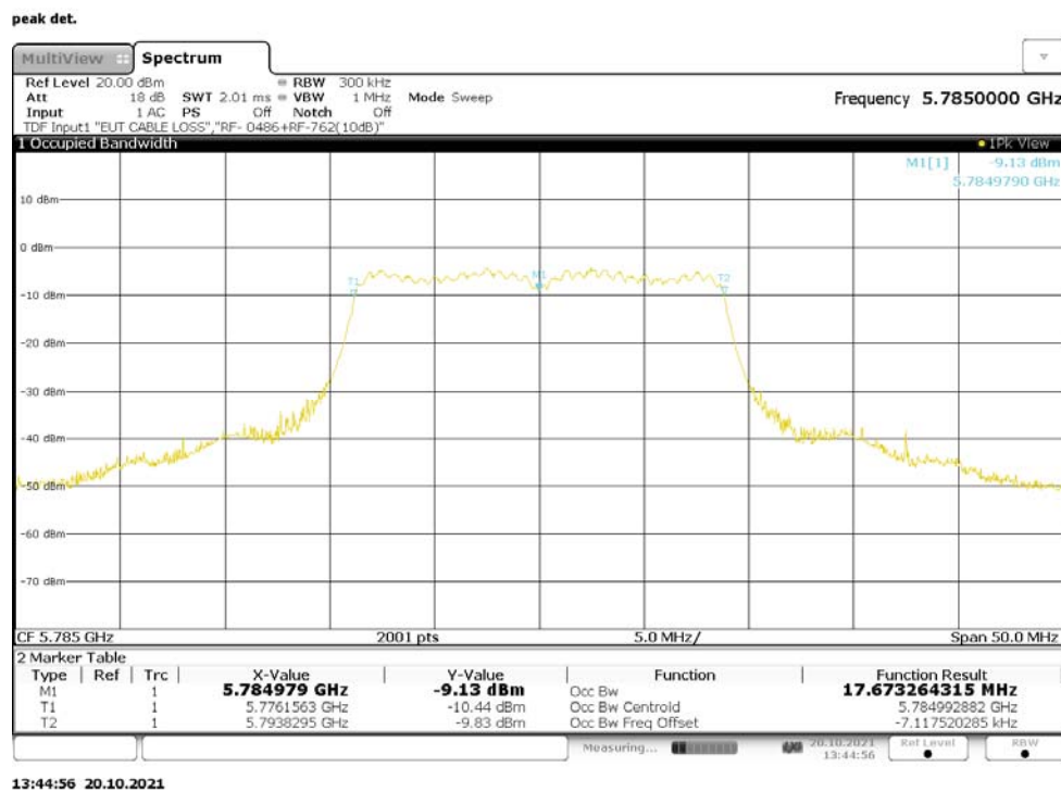
Figure 63: 99% Bandwidth, 802.11n-20, CDD, RF0, 5785MHz
