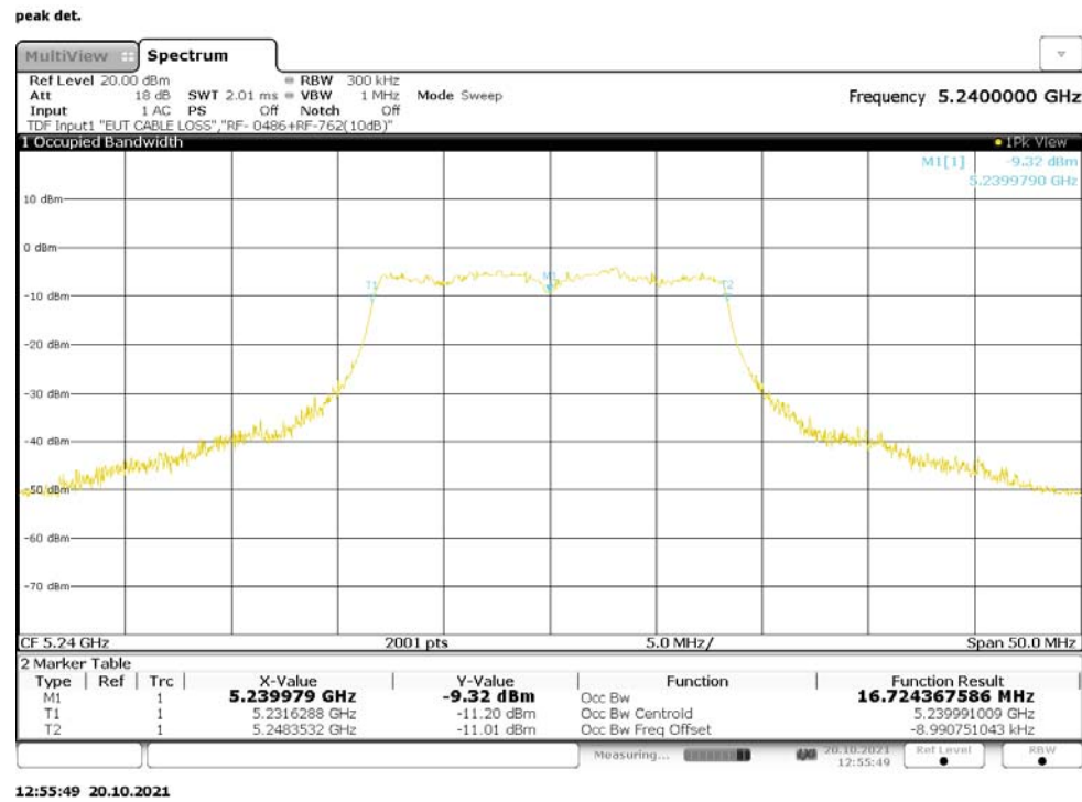
Figure 43: 99% Bandwidth, 802.11a, SISO, RF0, 5240MHz
