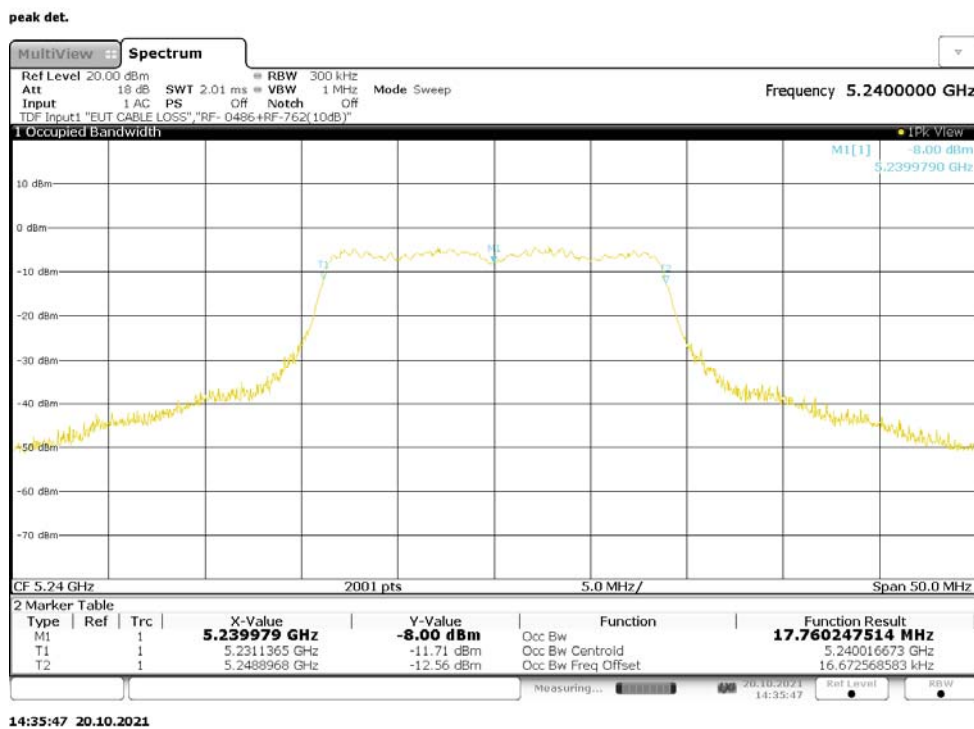
Figure 55: 99% Bandwidth, 802.11n-20, SISO, RF0, 5240MHz
