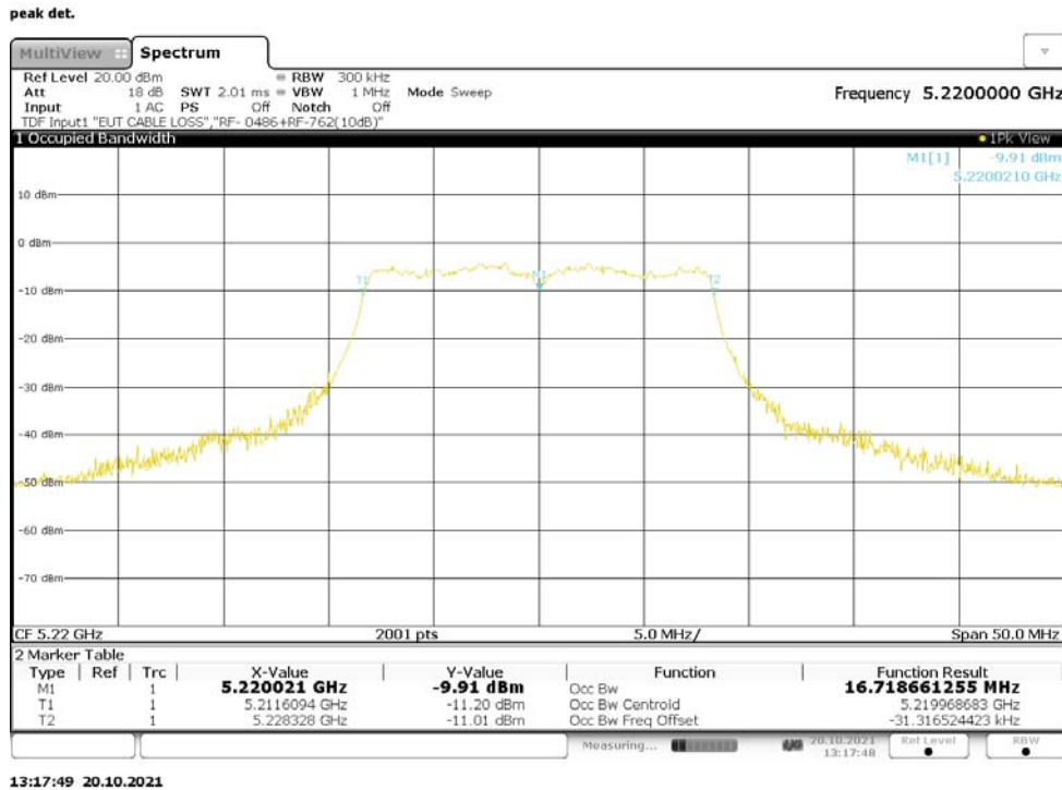
Figure 48: 99% Bandwidth, 802.11a, CDD, RF0, 5220MHz
