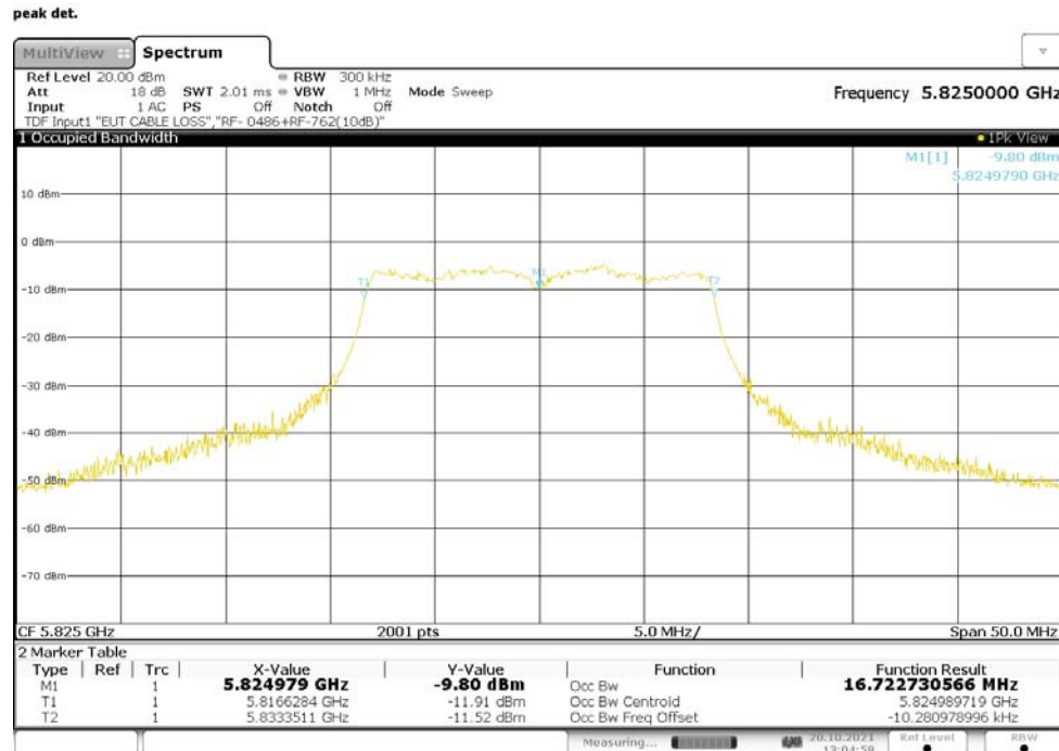
Figure 46: 99% Bandwidth, 802.11a, SISO, RF0, 5825MHz
