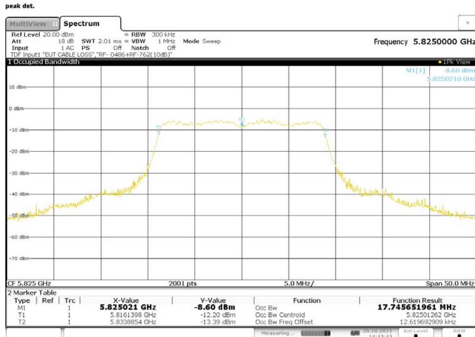
Figure 58: 99% Bandwidth, 802.11n-20, SISO, RF0, 5825MHz
