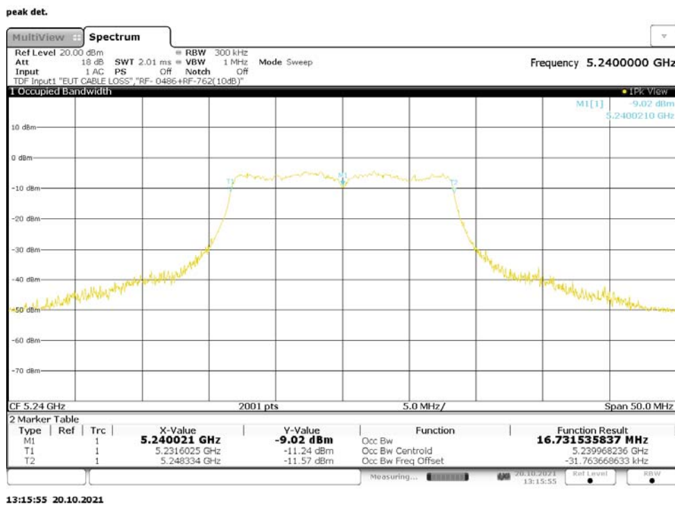
Figure 49: 99% Bandwidth, 802.11a, CDD, RF0, 5240MHz
