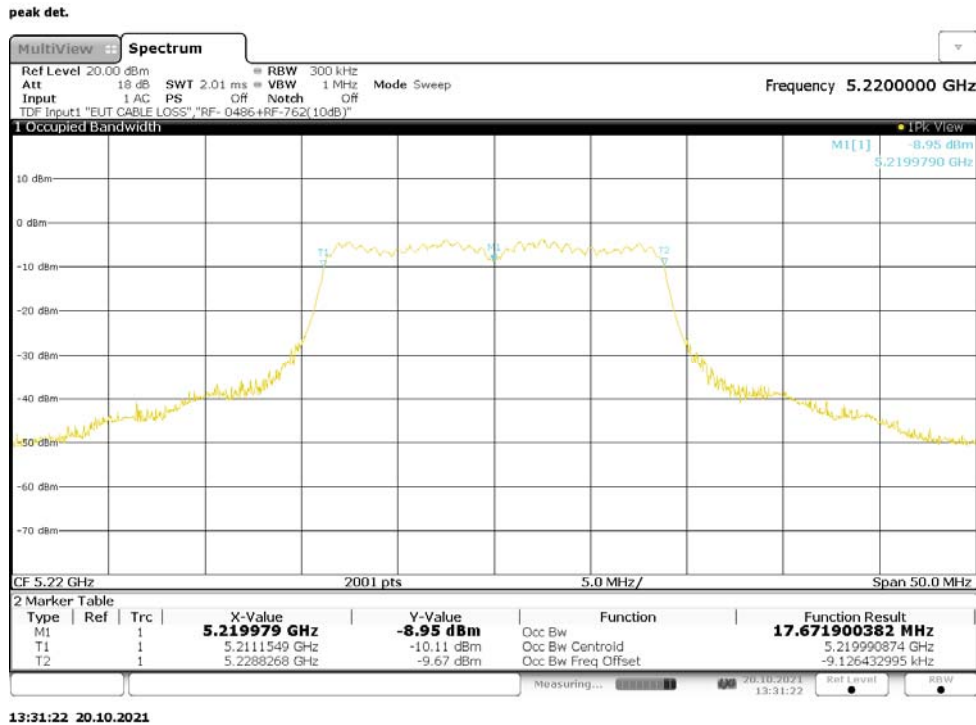
Figure 66: 99% Bandwidth, 802.11n-20, MIMO, RF0, 5220MHz
