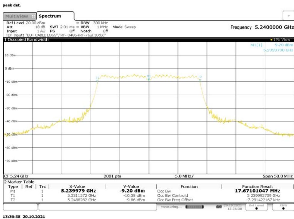
Figure 67: 99% Bandwidth, 802.11n-20, MIMO, RF0, 5240MHz
