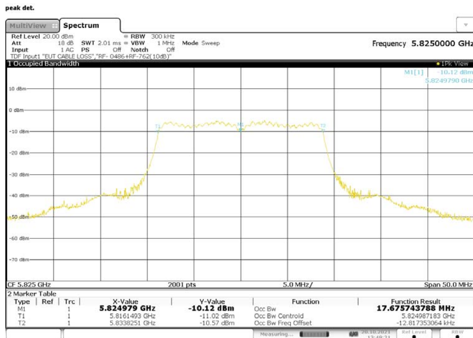
Figure 70: 99% Bandwidth, 802.11n-20, MIMO, RF0, 5825MHz
