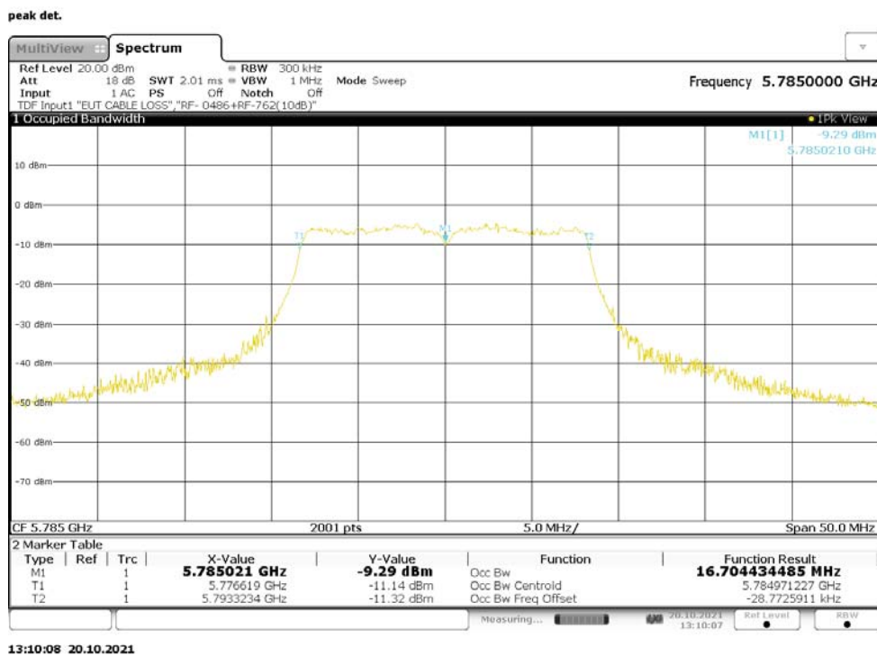
Figure 51: 99% Bandwidth, 802.11a, CDD, RF0, 5785MHz
