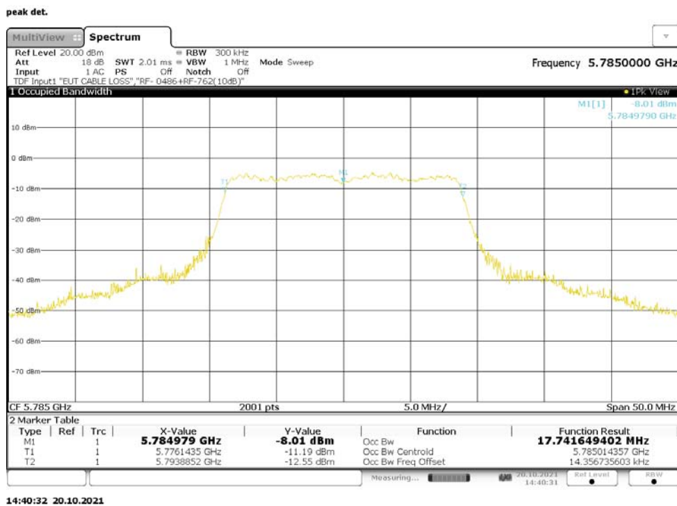
Figure 57: 99% Bandwidth, 802.11n-20, SISO, RF0, 5785MHz
