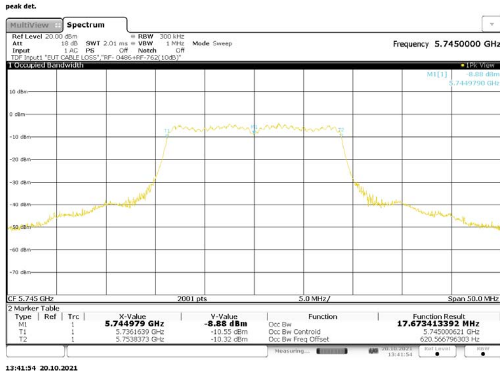
Figure 62: 99% Bandwidth, 802.11n-20, CDD, RF0, 5745MHz
