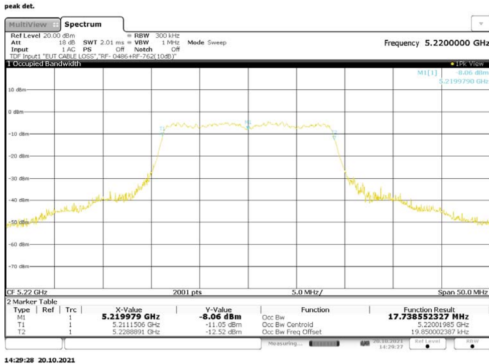
Figure 54: 99% Bandwidth, 802.11n-20, SISO, RF0, 5220MHz
