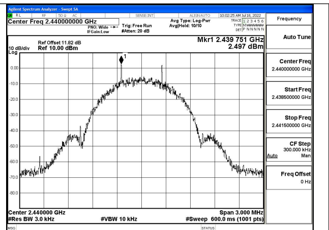
Test Mode:Coded 125K
