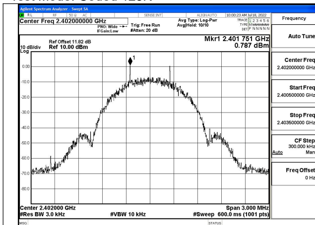
Test Mode:Coded 125K
