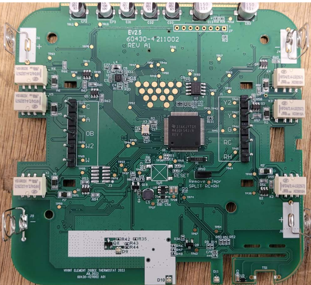
Bottom View of the PCB - View #4
