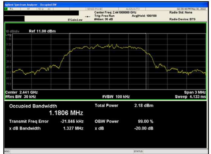
Middle Channel
