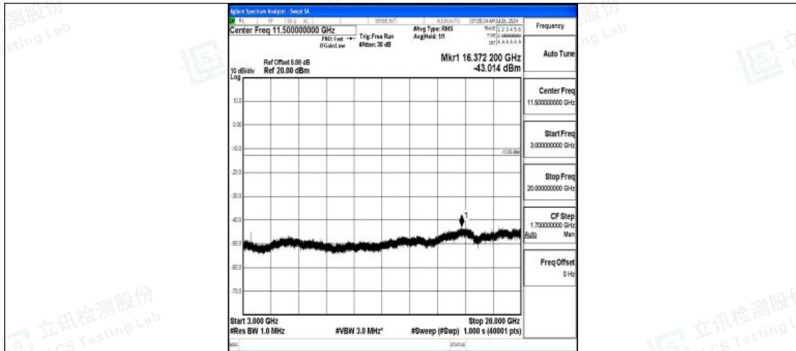
Band4-15MHz-QPSK-20325-1RB#0-3000~20000-PASS
