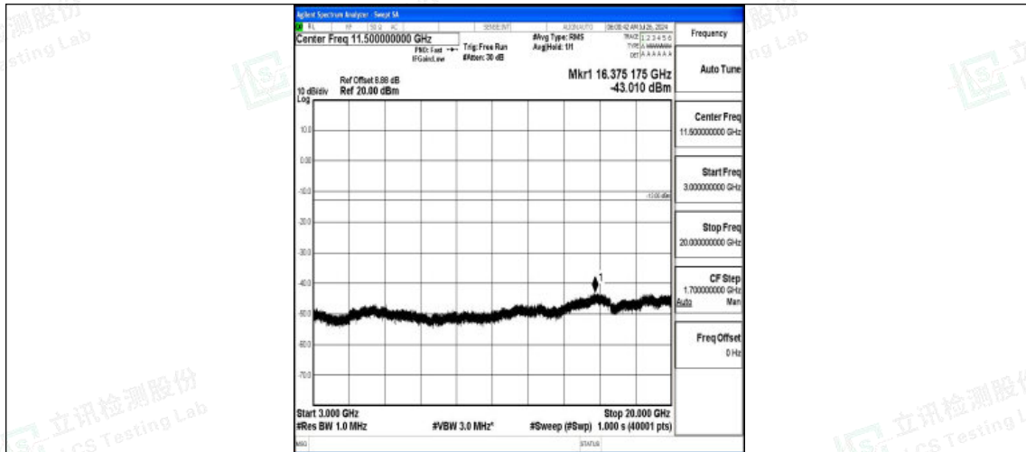
Band4-3MHz-QPSK-20385-1RB#0-3000~20000-PASS
