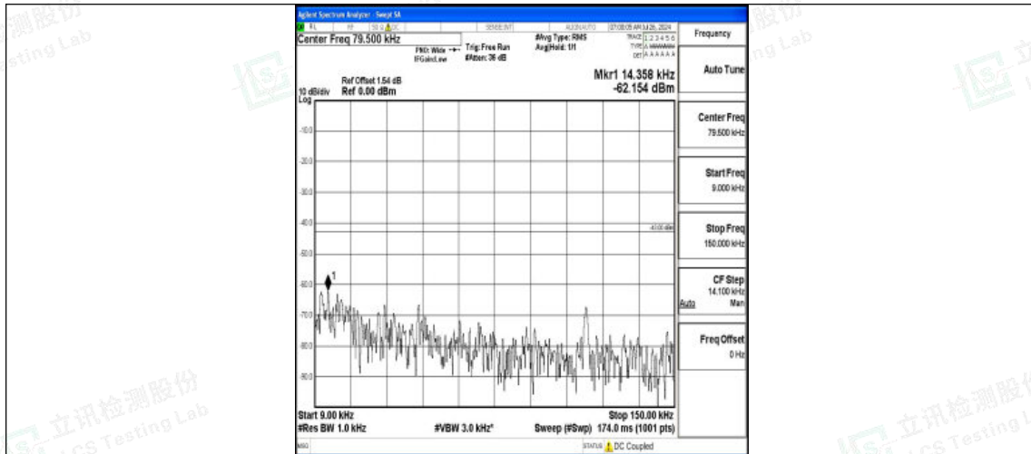
Band4-15MHz-QPSK-20025-1RB#0-0.009~0.15-PASS
