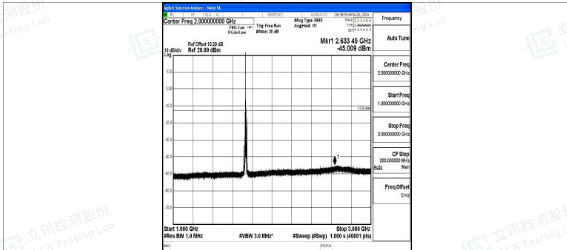
Band4-10MHz-16QAM-20175-1RB#0-1000~3000-PASS
