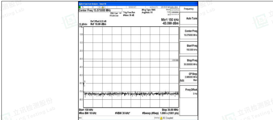
Band4-20MHz-QPSK-20300-1RB#0-0.15~30-PASS
