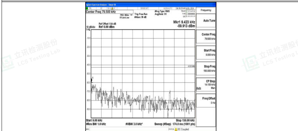
Band4-10MHz-QPSK-20350-1RB#0-0.009~0.15-PASS
