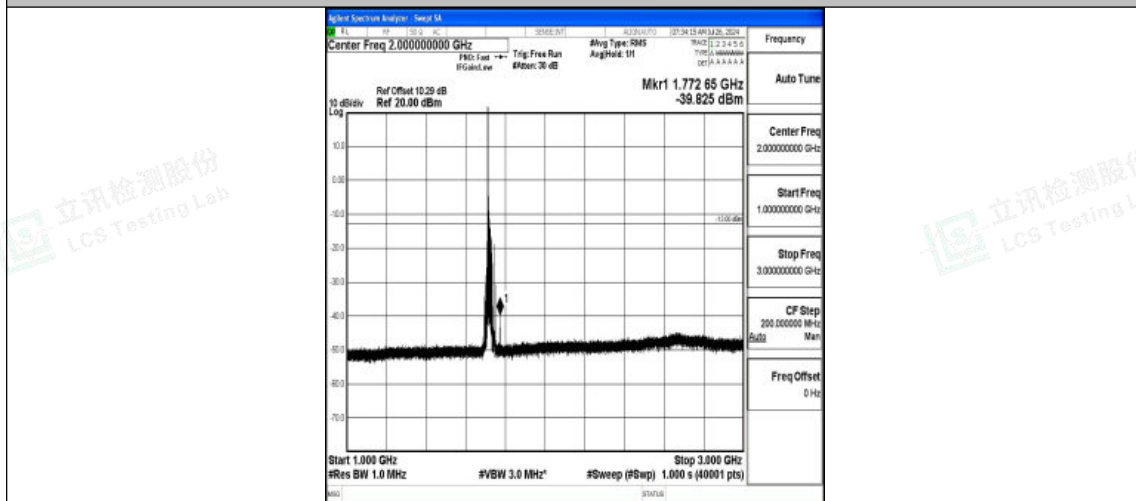
Band4-20MHz-16QAM-20050-1RB#0-1000~3000-PASS
