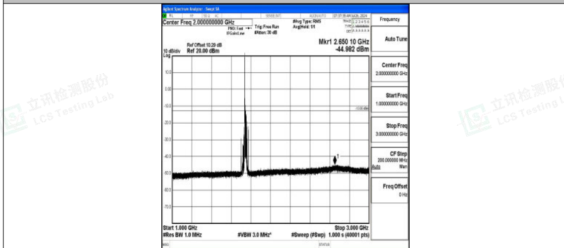
Band4-20MHz-QPSK-20300-1RB#0-1000~3000-PASS
