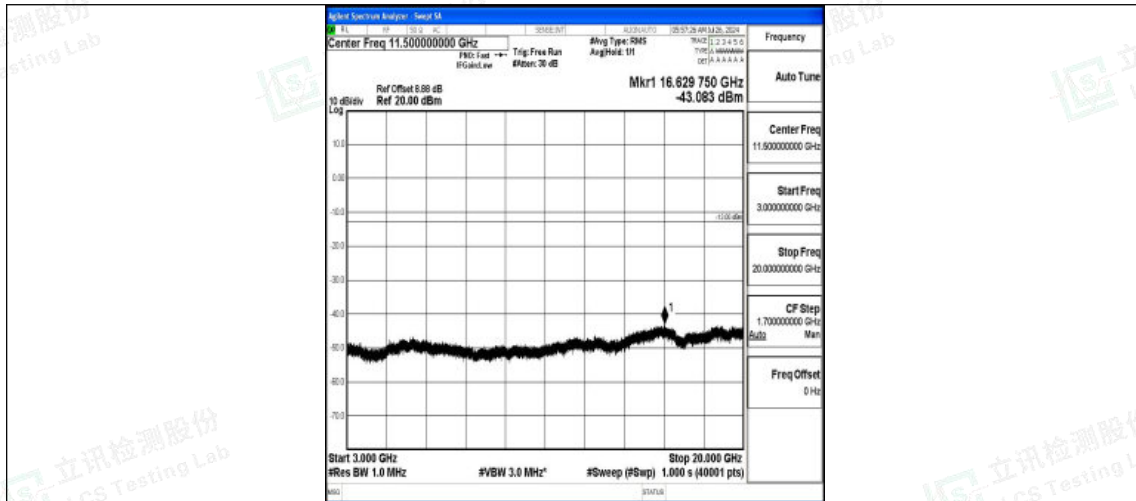
Band4-3MHz-16QAM-19965-1RB#0-3000~20000-PASS
