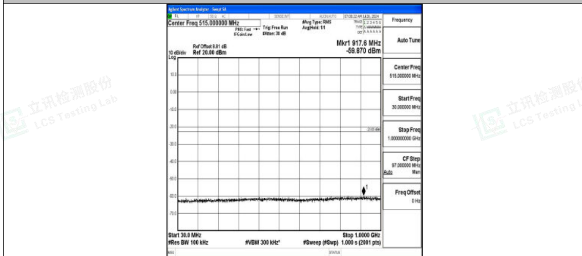
Band4-15MHz-QPSK-20025-1RB#0-30~1000-PASS
