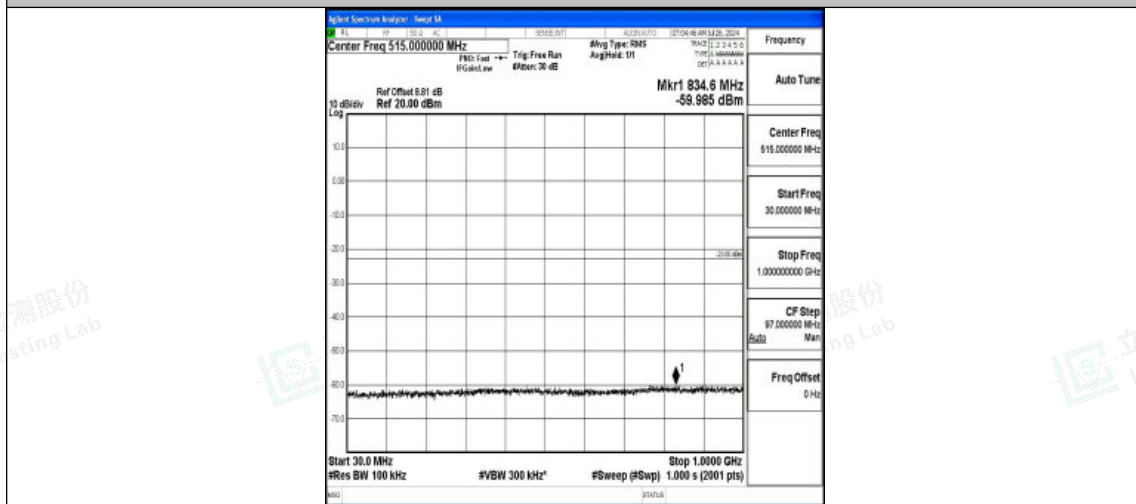
Band4-15MHz-QPSK-20325-1RB#0-0-30~1000-PASS
