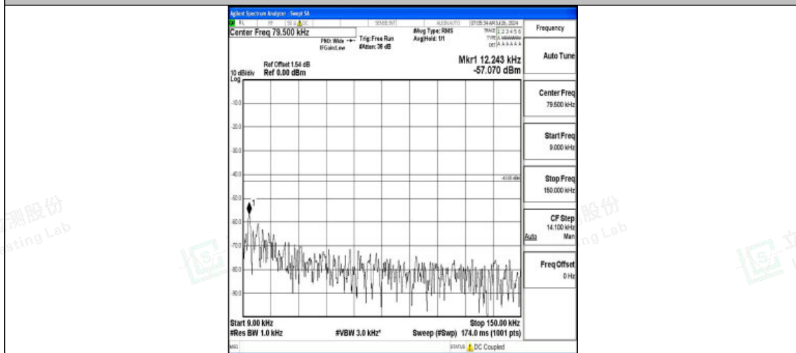
Band4-15MHz-16QAM-20325-1RB#0-0.009~0.15-PASS
