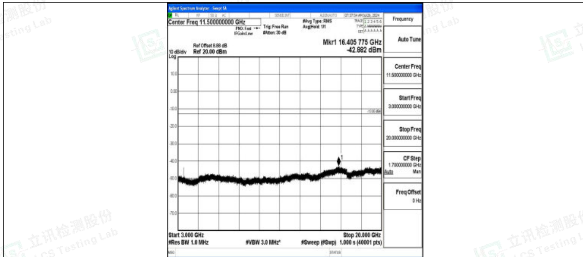
Band4-20MHz-QPSK-20300-1RB#0-3000~20000-PASS
