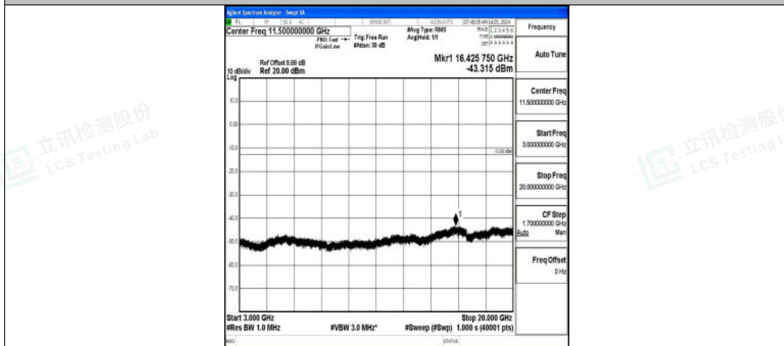
Band4-1.4MHz-16QAM-20393-1RB#0-3000~20000-PASS
