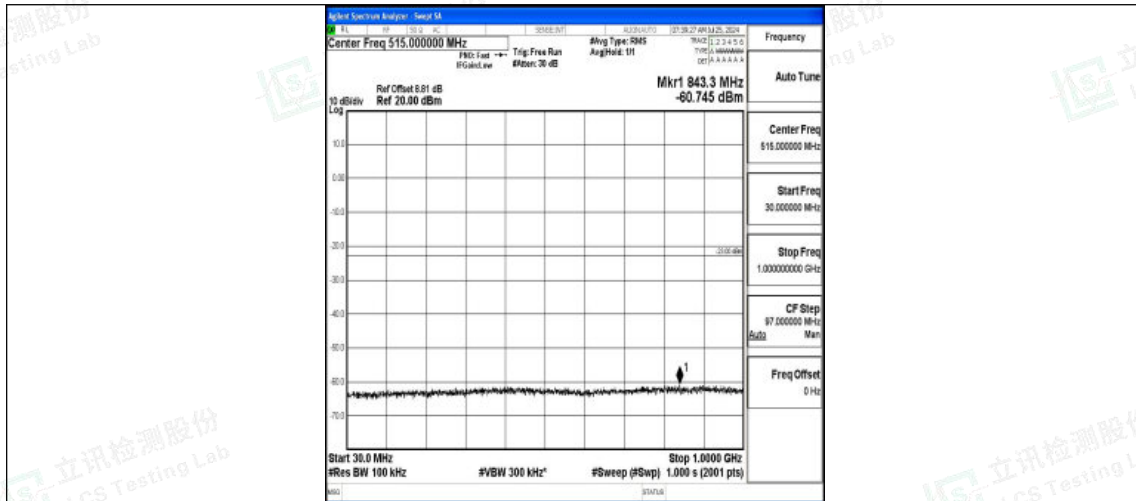
Band4-1.4MHz-16QAM-20393-1RB#0-30~1000-PASS
