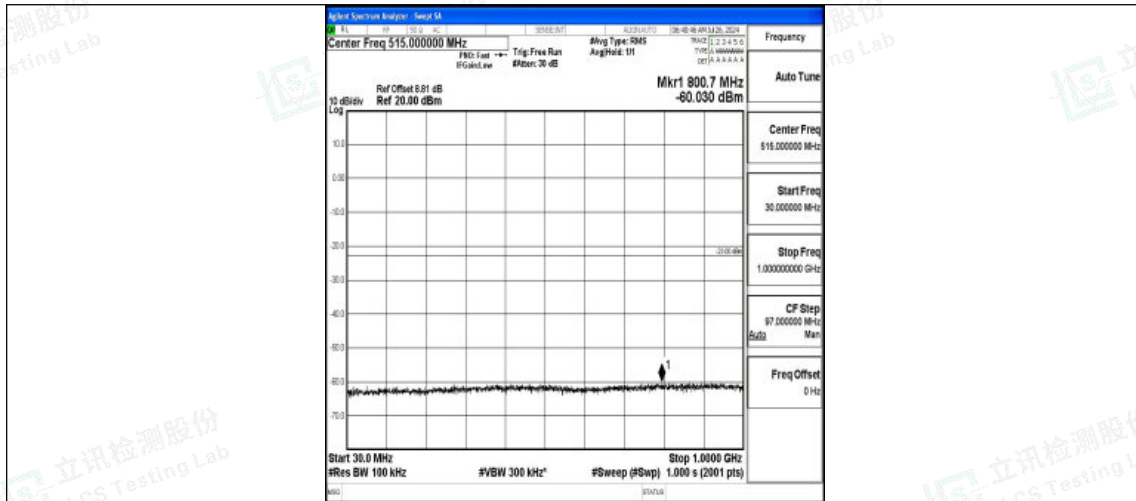
Band4-10MHz-16QAM-20350-1RB#0-30~1000-PASS
