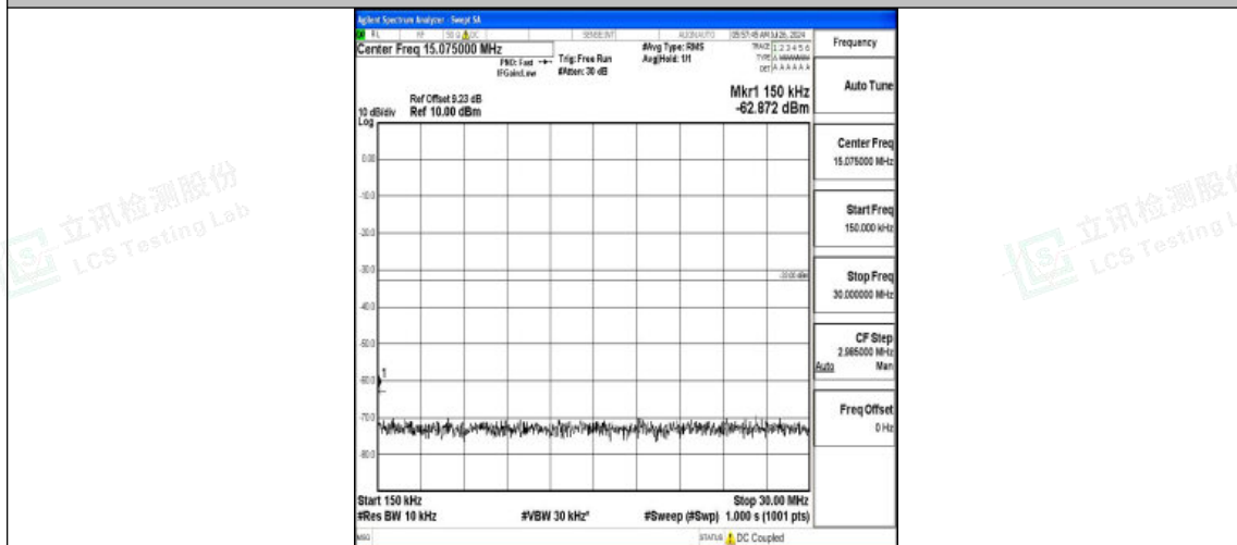
Band4-3MHz-QPSK-20175-1RB#0-0.15~30-PASS
