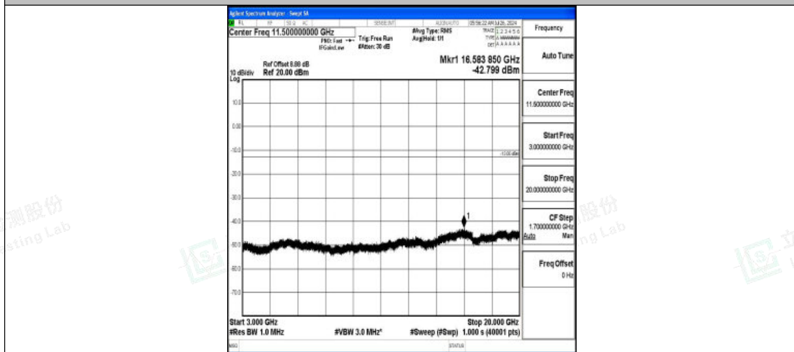
Band4-3MHz-QPSK-19965-1RB#0-3000~20000-PASS
