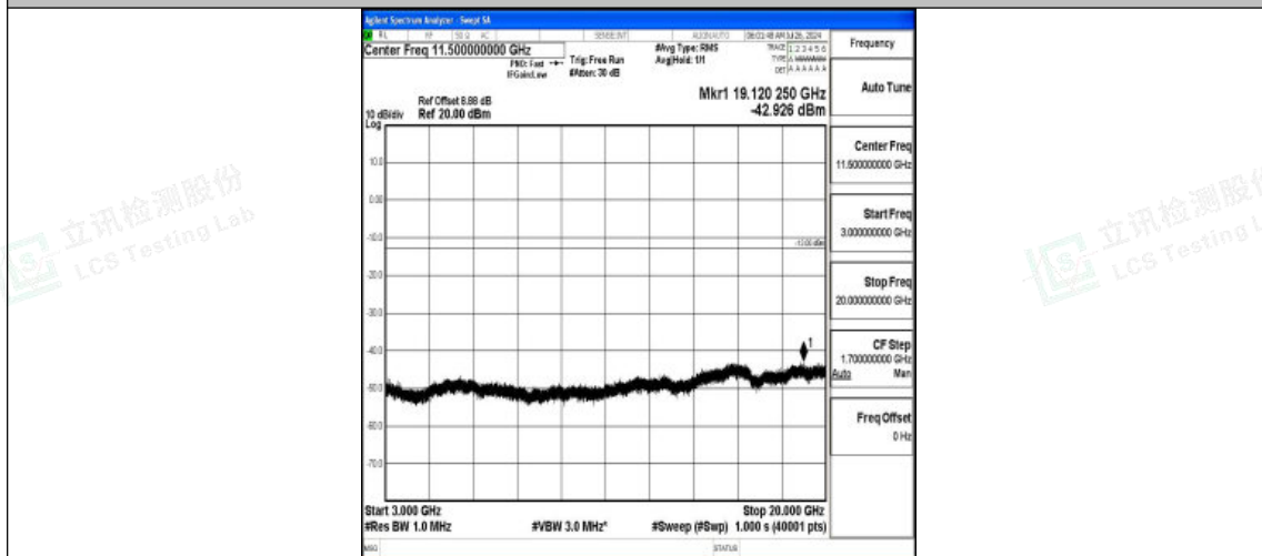
Band4-3MHz-16QAM-20385-1RB#0-3000~20000-PASS
