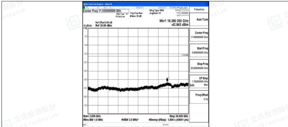
Band4-1.4MHz-QPSK-20393-1RB#0-3000~20000-PASS
