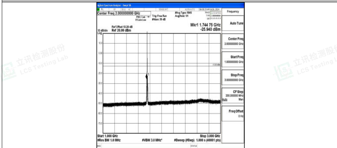
Band4-3MHz-QPSK-20385-1RB#0-1000~3000-PASS
