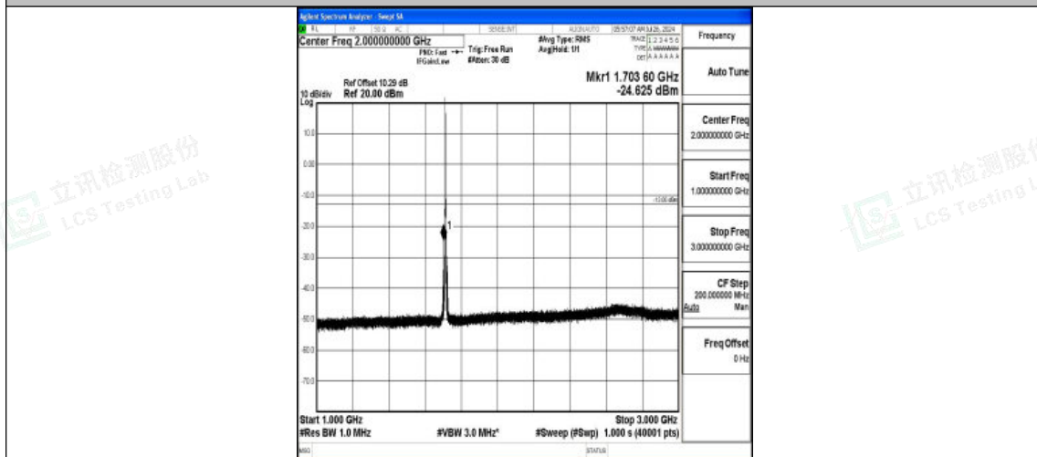
Band4-3MHz-16QAM-19965-1RB#0-1000~3000-PASS
