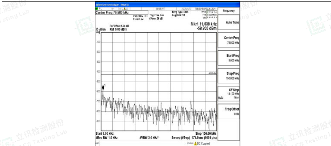
Band4-5MHz-QPSK-19975-1RB#0-0.009~0.15-PASS
