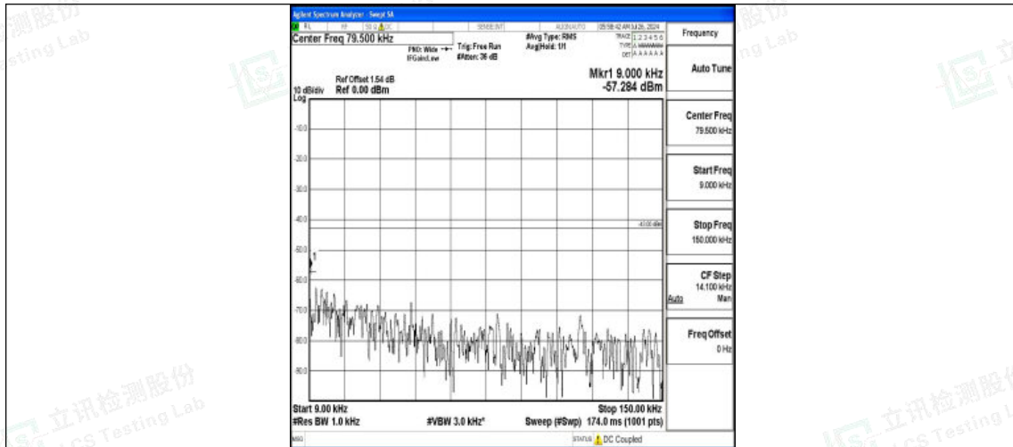
Band4-3MHz-16QAM-20175-1RB#0-0.009~0.15-PASS
