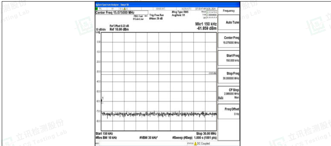
Band4-20MHz-16QAM-20050-1RB#0-0.15~30-PASS
