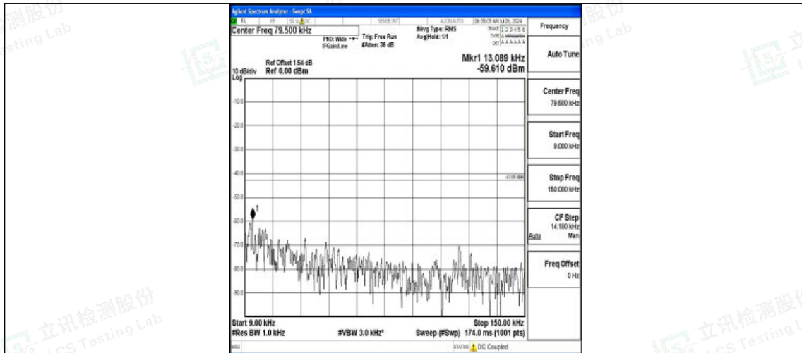
Band4-10MHz-QPSK-20000-1RB#0-0.009~0.15-PASS
