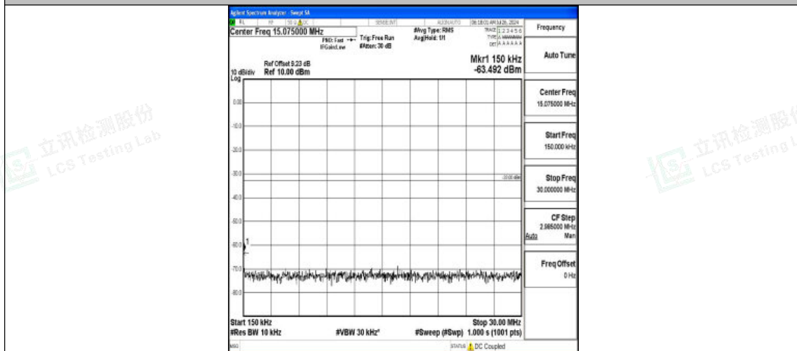
Band4-5MHz-QPSK-20175-1RB#0-0.15~30-PASS
