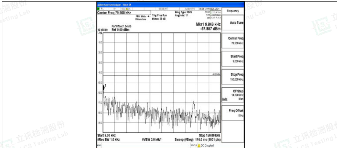
Band4-10MHz-16QAM-20175-1RB#0-0.009~0.15-PASS
