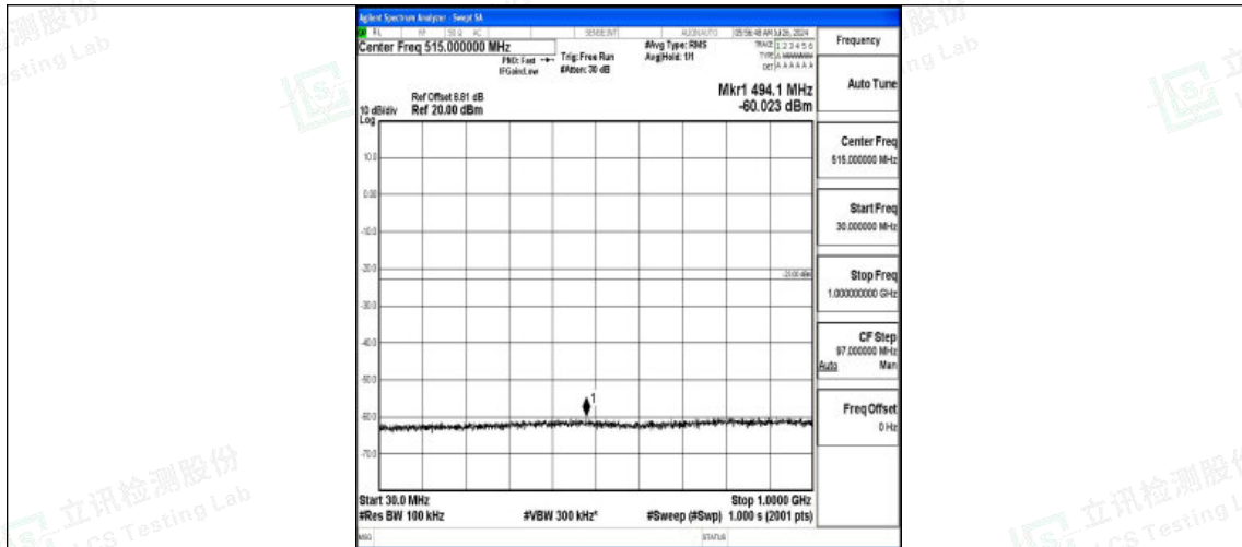
Band4-3MHz-16QAM-19965-1RB#0-30~1000-PASS
