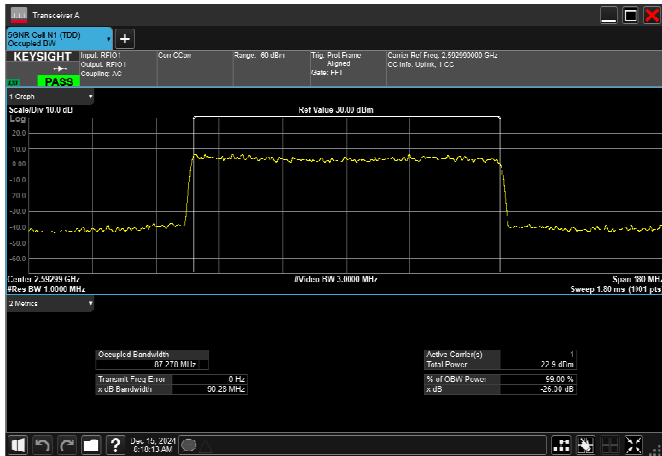
n41_90MHz_30kHz_2592.99MHz_CP-OFDM 256 QAM_RB245@0
