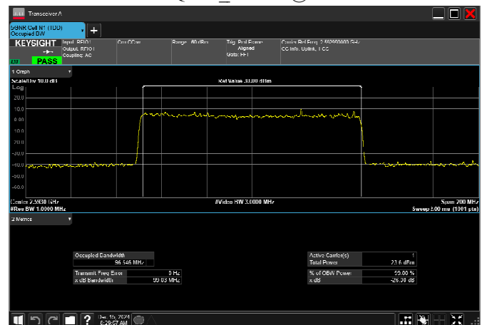
n41_100MHz_30kHz_2592.99MHz_DFT-s-OFDM 64 QAM_RB270@0
