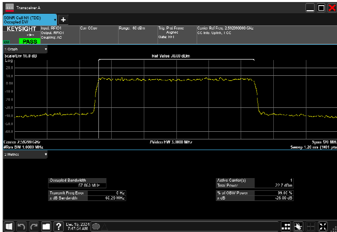
n41_60MHz_30kHz_2592.99MHz_CP-OFDM 256 QAM_RB162@0
