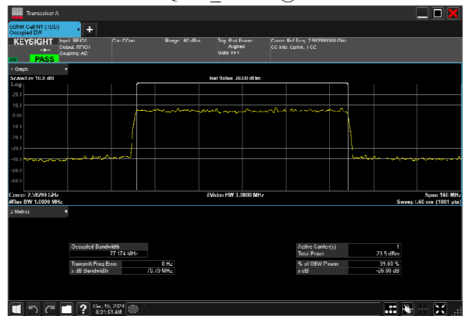
n41_80MHz_30kHz_2592.99MHz_DFT-s-OFDM 16 QAM_RB216@0
