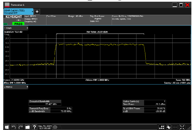
n41_80MHz_30kHz_2592.99MHz_DFT-s-OFDM 16 QAM_RB216@0
