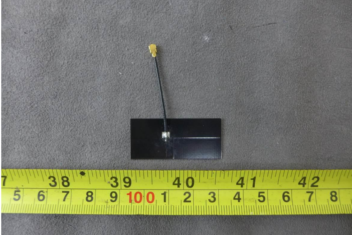
PCB Antenna
