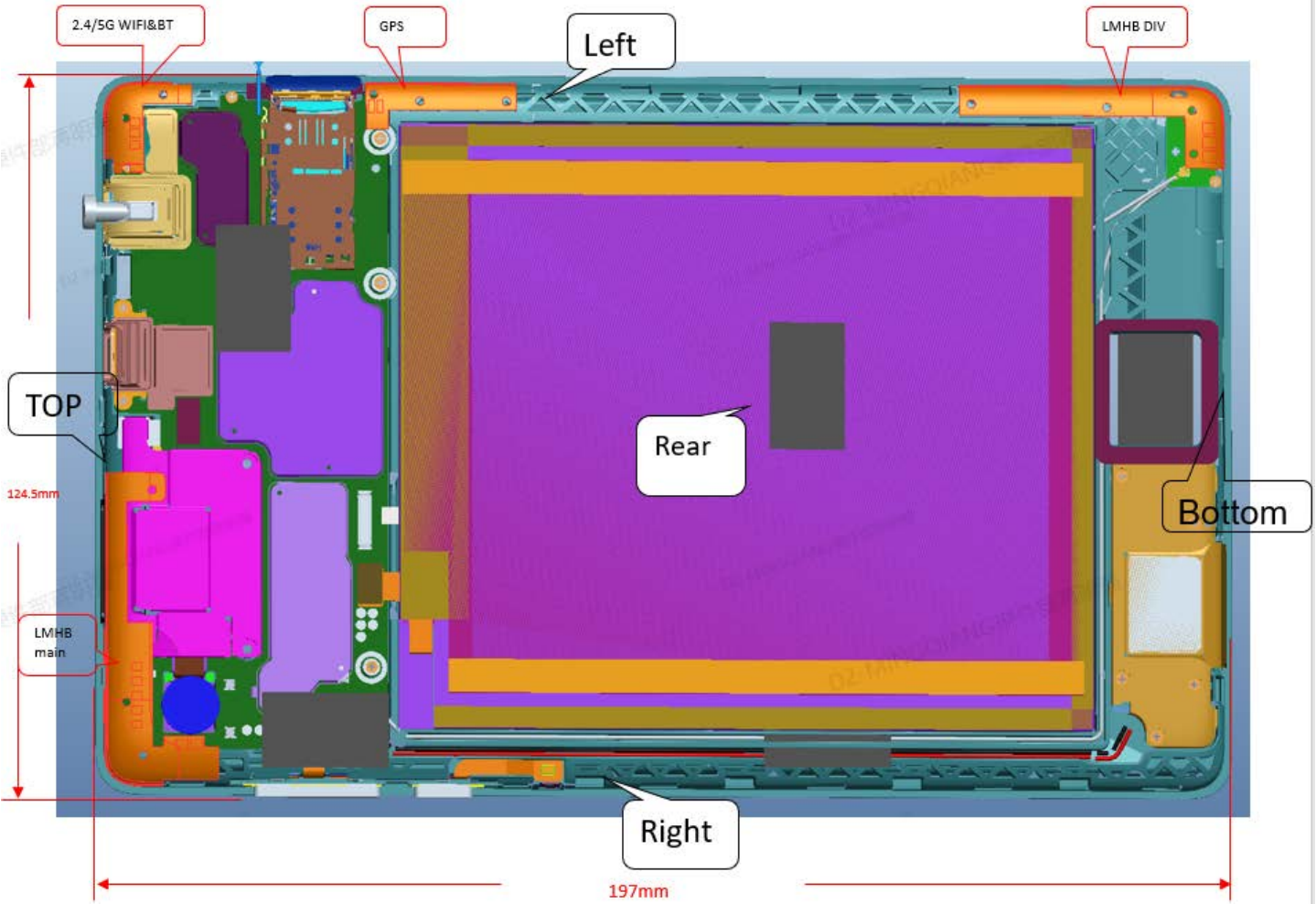
Antenna area diagram
