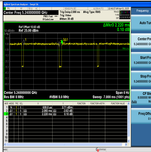
NTNV-11A-Ant2-5240
