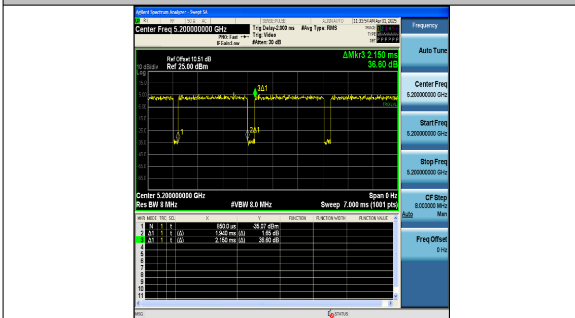
NTNV-11AC20MIMO-Ant2-5200
