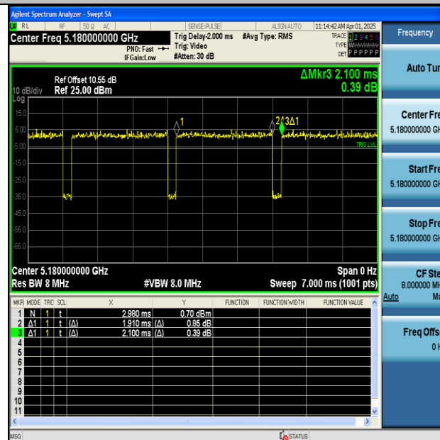
NTNV-11N20MIMO-Ant1-5180
