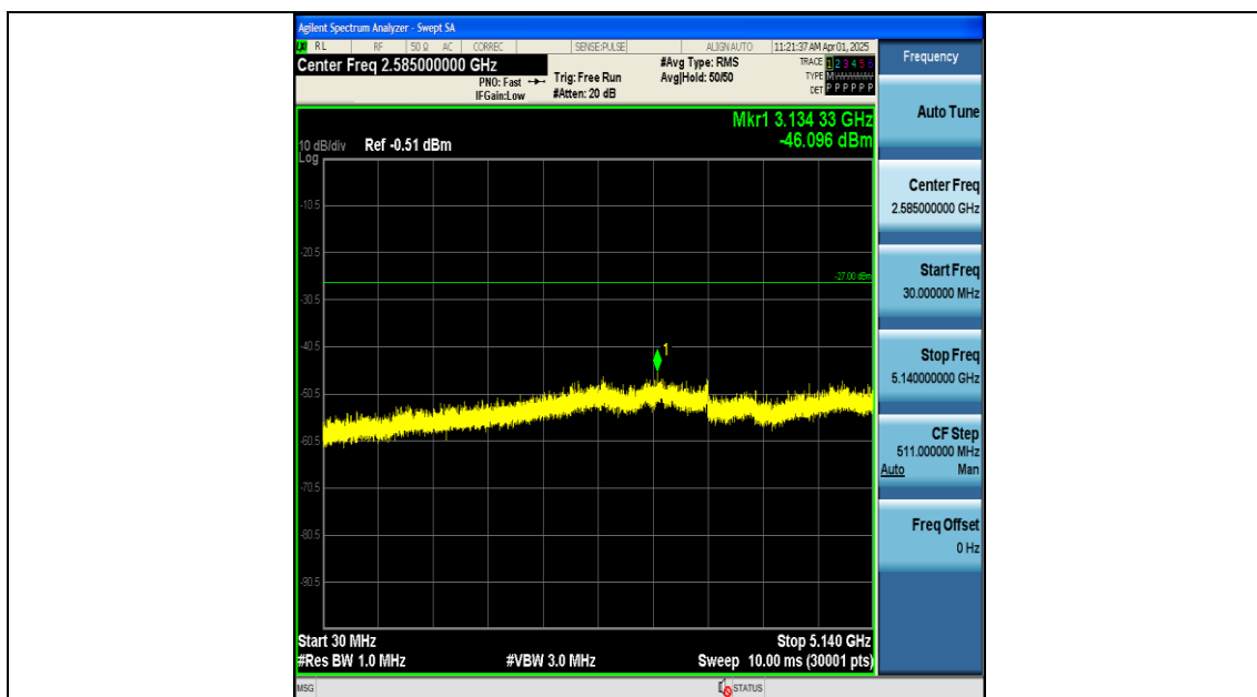
11N20MIMO-Ant2-5200-30~5140-PASS
