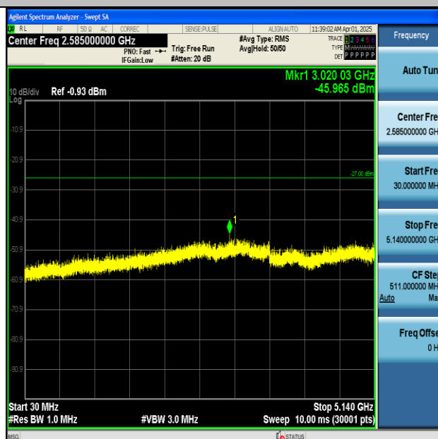
11AC20MIMO-Ant2-5240-30~5140-PASS
