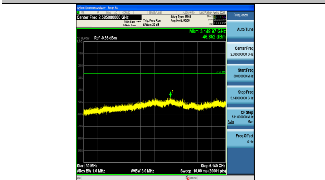
11A-Ant1-5200-30~5140-PASS
