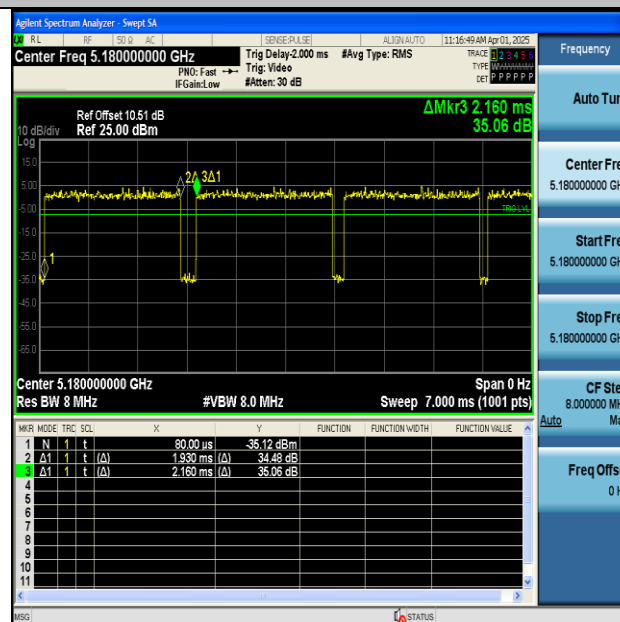
NTNV-11N20MIMO-Ant2-5180
