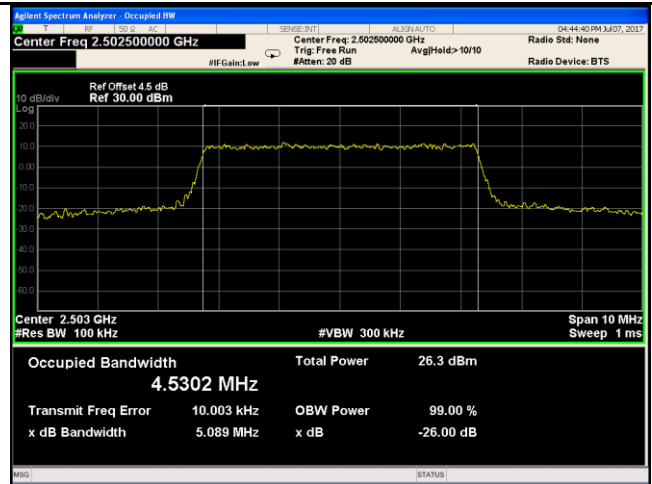
LTE Band VII - Low CH 16QAM-5
