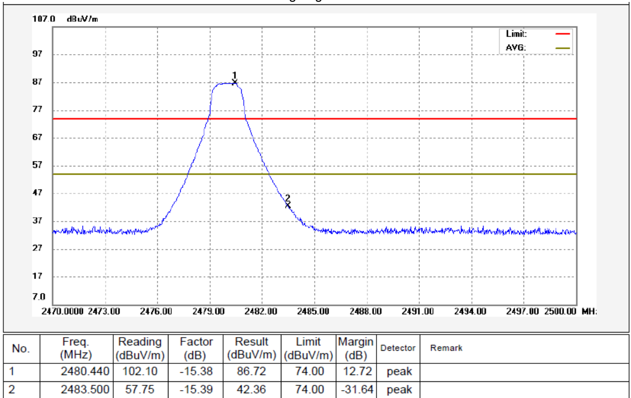
BLE: Band edge-right side Vertical
