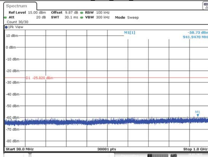
11N20SISO_Ant1_2437_30~1000
