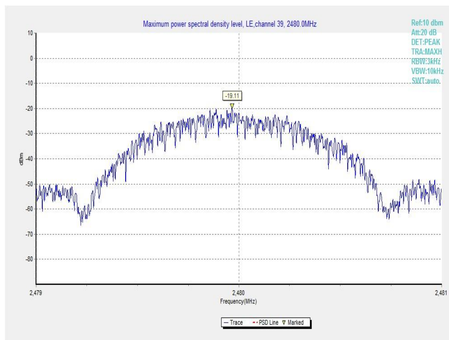
Fig.6 Power Spectral Density (Ch 39)
