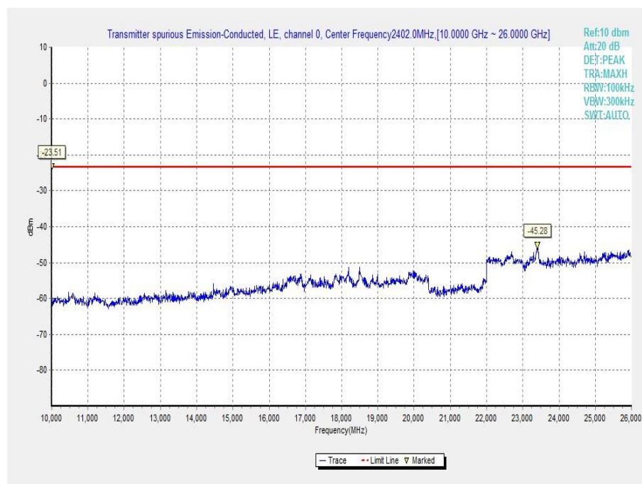
Fig.16 Conducted Spurious Emission (Ch0, 10 GHz-26 GHz)
