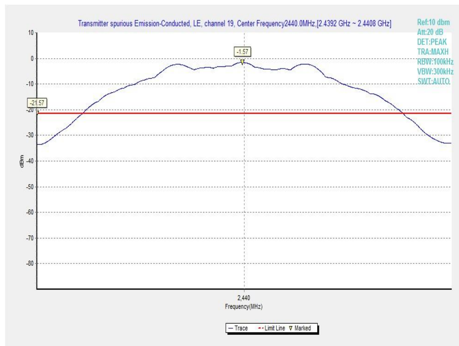
Fig.17 Conducted Spurious Emission (Ch19, Center Frequency)
