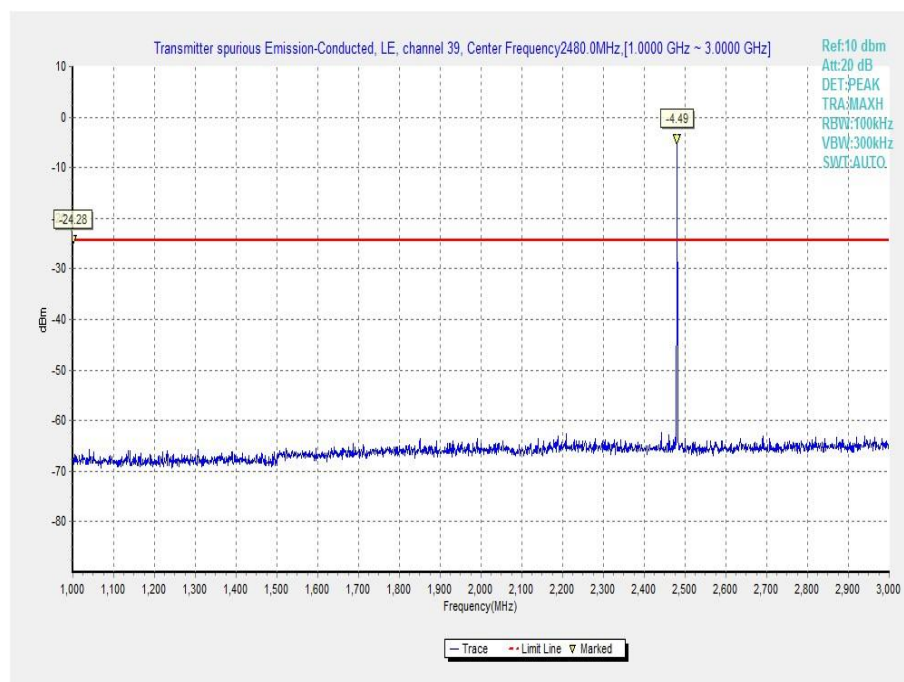
Fig.24 Conducted Spurious Emission (Ch39, 1 GHz-3 GHz)
