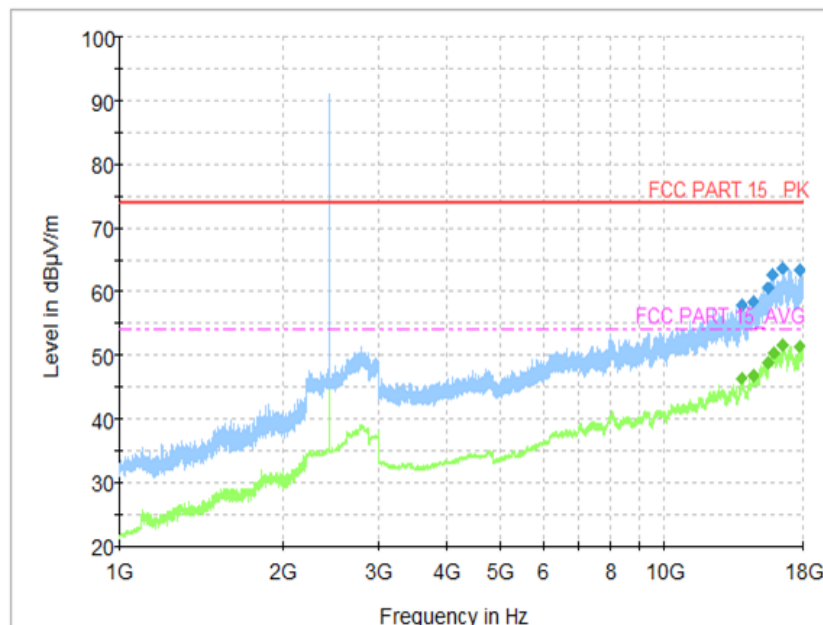
Fig.30 Radiated Spurious Emission (Ch19, 1 GHz- 18 GHz)
