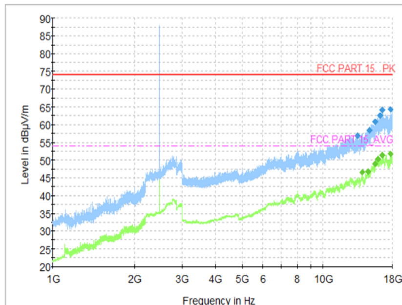
Fig.32 Radiated Spurious Emission (Ch39, 1 GHz-18 GHz)
