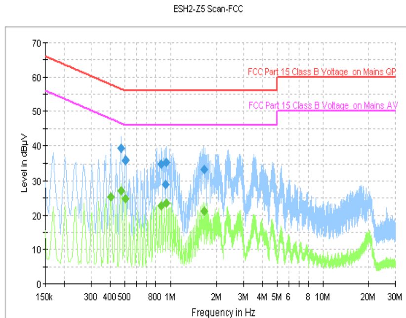
Fig.38 AC Power line Conducted Emission (Idle, AE1, 240V)
