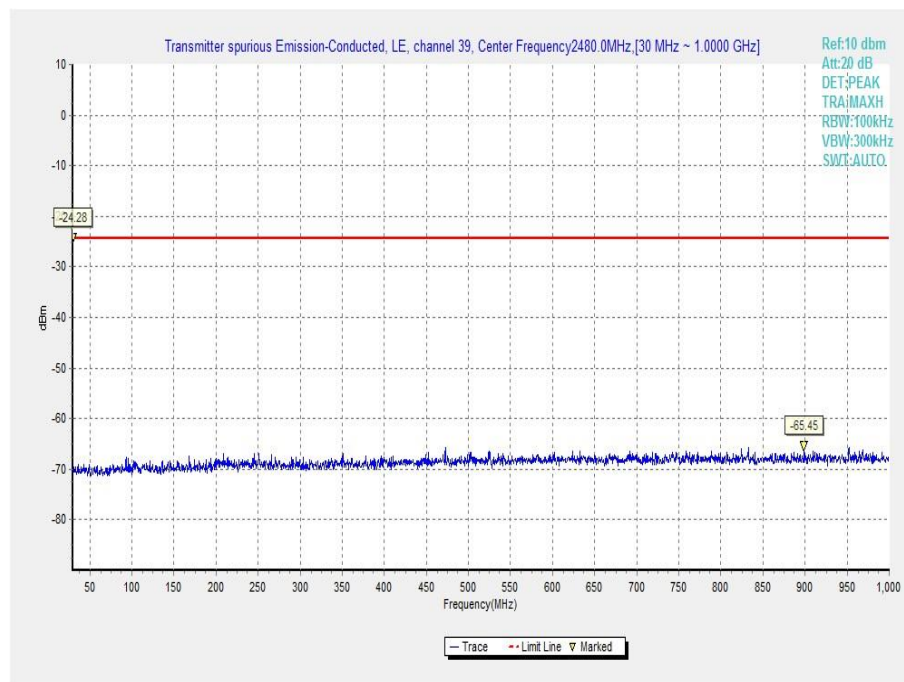
Fig.23 Conducted Spurious Emission (Ch39, 30 MHz-1 GHz)
