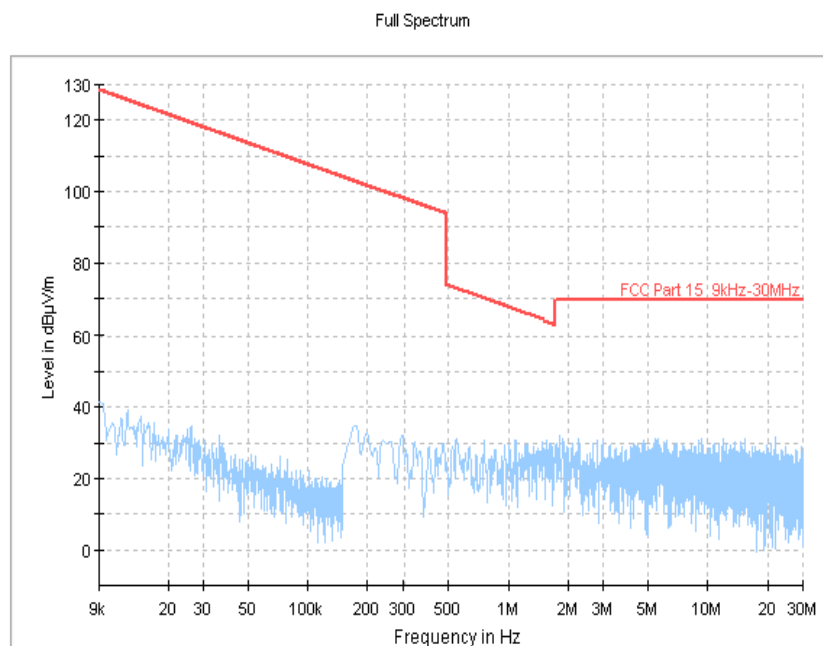
Fig.28 Radiated Spurious Emission (Ch19, 9 kHz-30 MHz)
