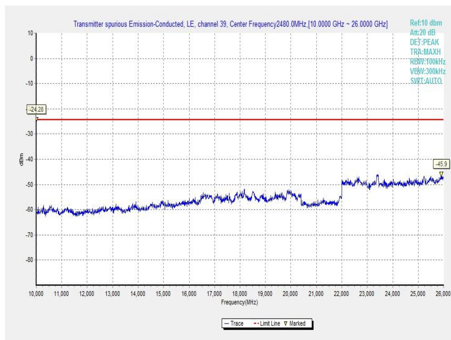
Fig.26 Conducted Spurious Emission (Ch39, 10 GHz-26 GHz)
