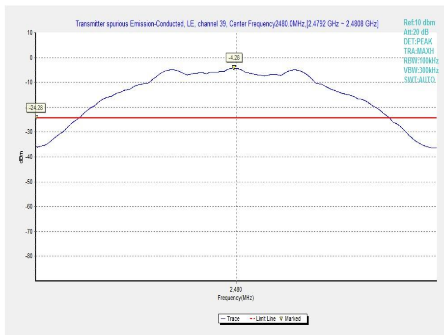
Fig.22 Conducted Spurious Emission (Ch39, Center Frequency)
