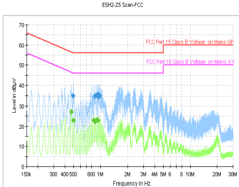
Fig.37 AC Powerline Conducted Emission (Traffic, AE1, 240V)
