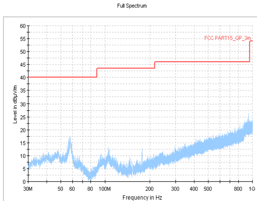
Fig.29 Radiated Spurious Emission (Ch19, 30 MHz-1 GHz)
