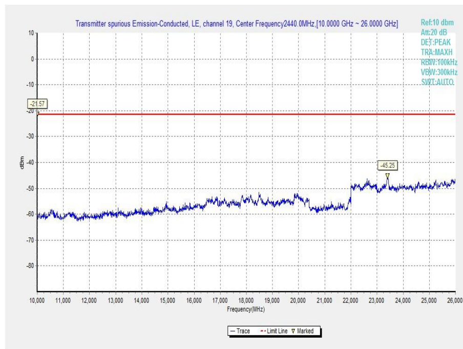
Fig.21 Conducted Spurious Emission (Ch19, 10 GHz-26 GHz)
