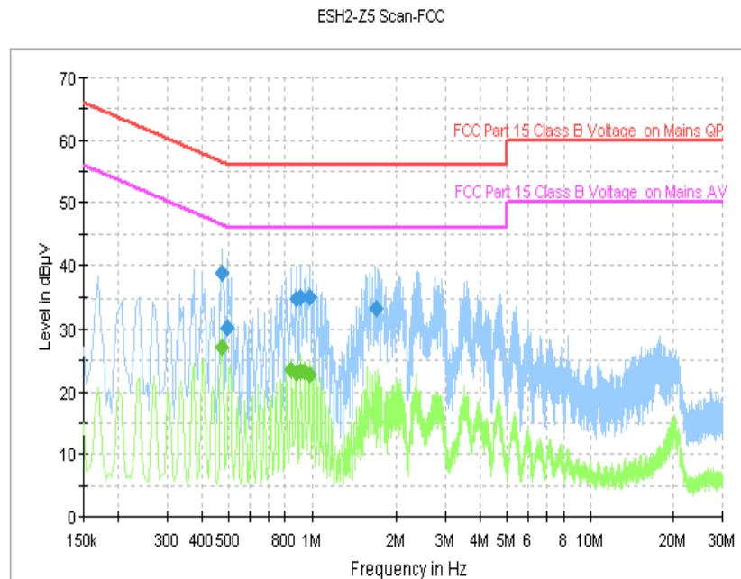
Fig.36 AC Power line Conducted Emission (Idle, AE1, 120V)
