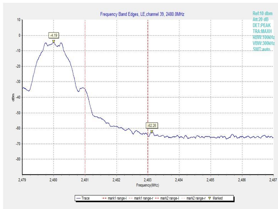
Fig.11 Band Edges (Ch 39)
