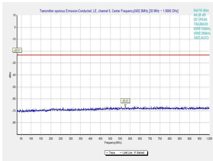
Fig.13 Conducted Spurious Emission (Ch0, 30 MHz-1 GHz)
