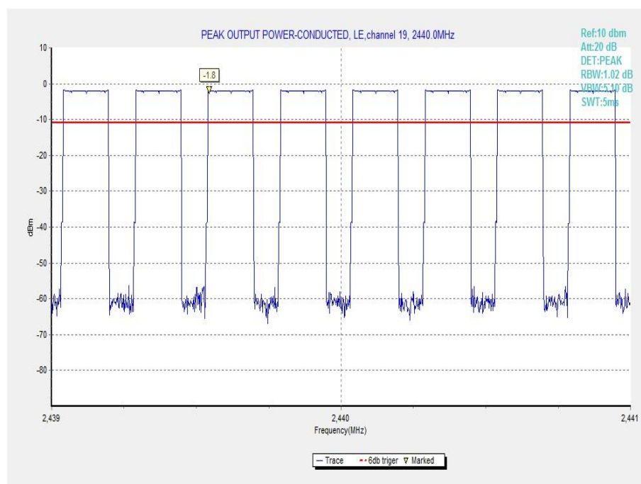
Fig.2 Maximum Peak Output Power(GFSK, Ch 19)
