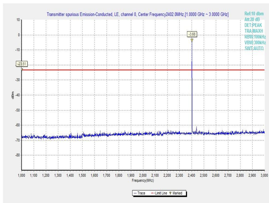
Fig.14 Conducted Spurious Emission (Ch0, 1 GHz-3 GHz)
