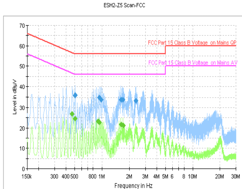
Fig.35 AC Powerline Conducted Emission (Traffic, AE1, 120V)
