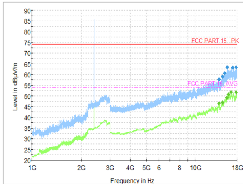
Fig.27 Radiated Spurious Emission (GFSK, Ch0, 1 GHz ~18 GHz)
