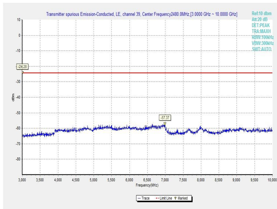
Fig.25 Conducted Spurious Emission (Ch39, 3 GHz-10 GHz)
