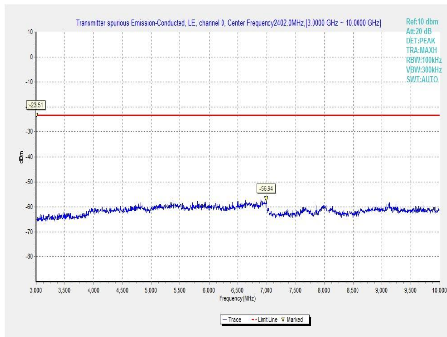
Fig.15 Conducted Spurious Emission (Ch0, 3 GHz-10 GHz)
