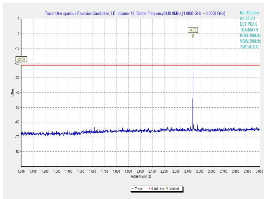
Fig.19 Conducted Spurious Emission (Ch19, 1 GHz-3 GHz)
