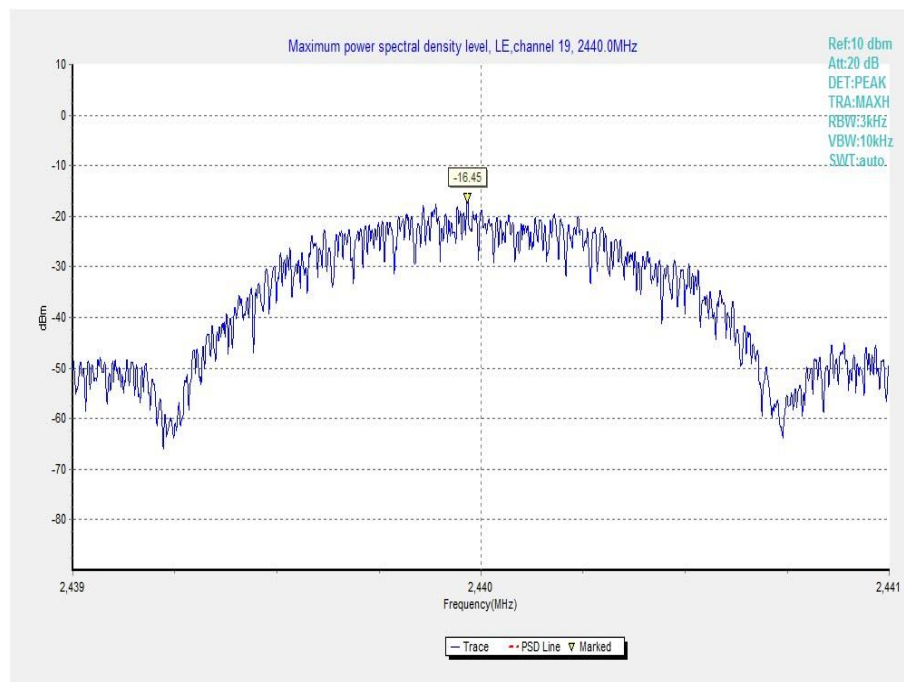
Fig.5 Power Spectral Density (Ch 19)
