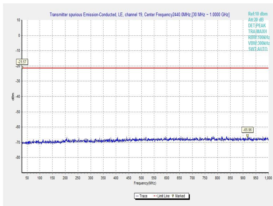
Fig.18 Conducted Spurious Emission (Ch19, 30 MHz-1 GHz)
