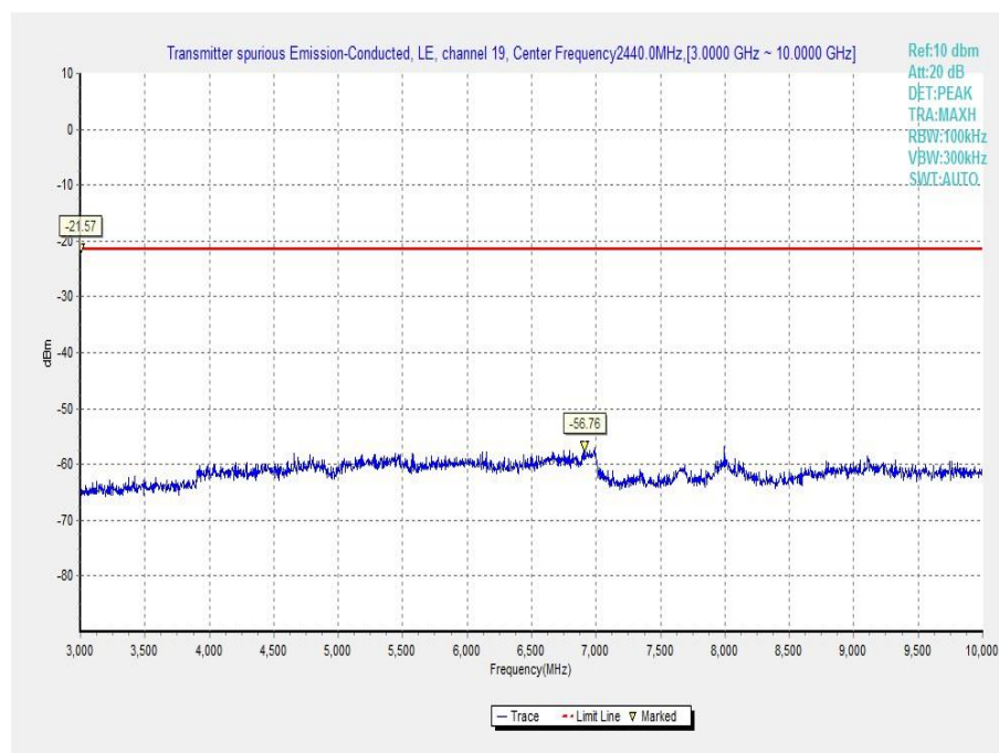
Fig.20 Conducted Spurious Emission (Ch19, 3 GHz-10 GHz)
