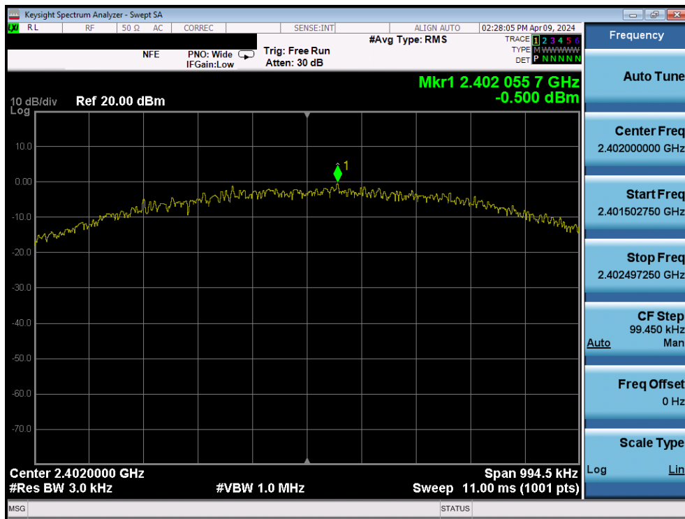
Plot 7-74. Power Spectral Density Plot (Bluetooth (LE), 1Mbps – Ch. 0) – Ant2
