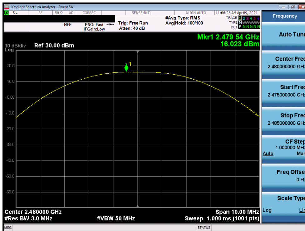
Plot 7-49. Peak Power Plot (Bluetooth (LE), 2Mbps – Ch. 39) – Ant2
