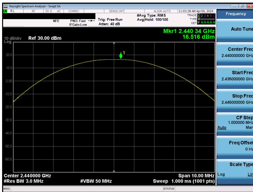
Plot 7-45. Peak Power Plot (Bluetooth (LE), 1Mbps – Ch. 19) – Ant2
