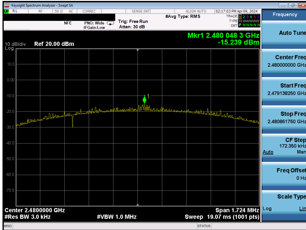
Plot 7-85. Power Spectral Density Plot (Bluetooth (LE), 2Mbps – Ch. 39) – Dual Ant1
