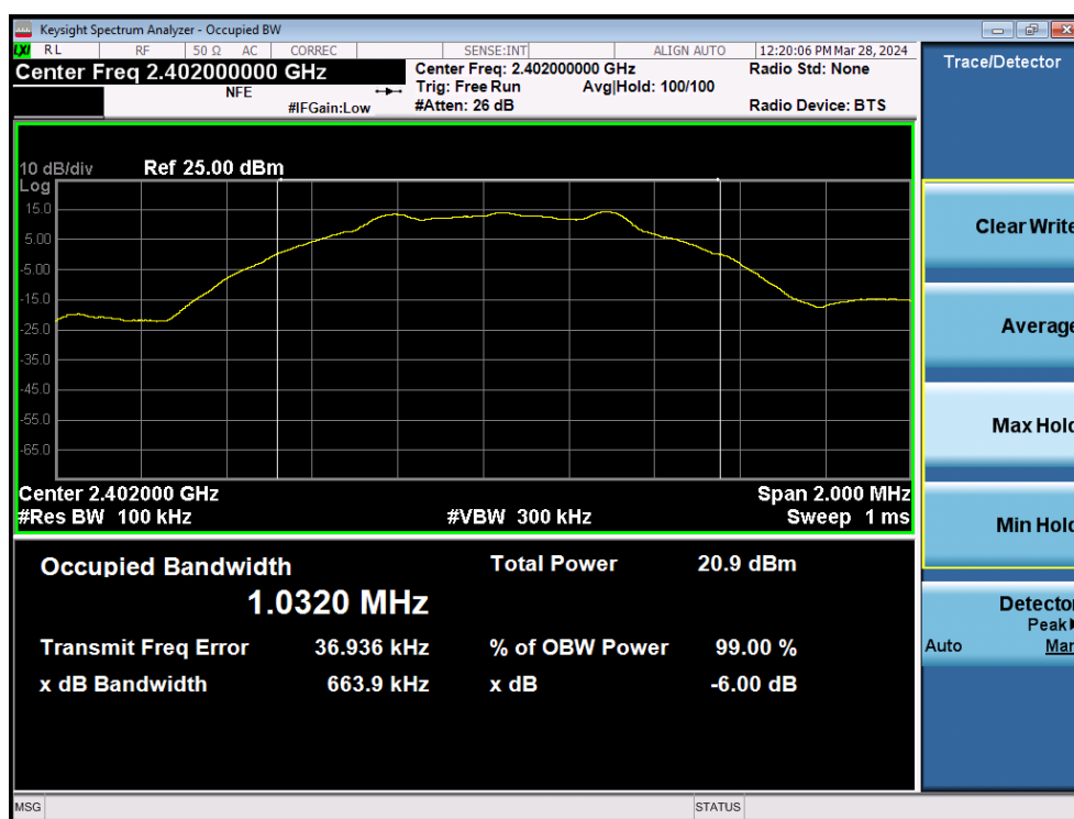
Plot 7-20. 6dB Bandwidth Plot (Bluetooth (LE), 1Mbps – Ch. 0 – Dual Ant1)
