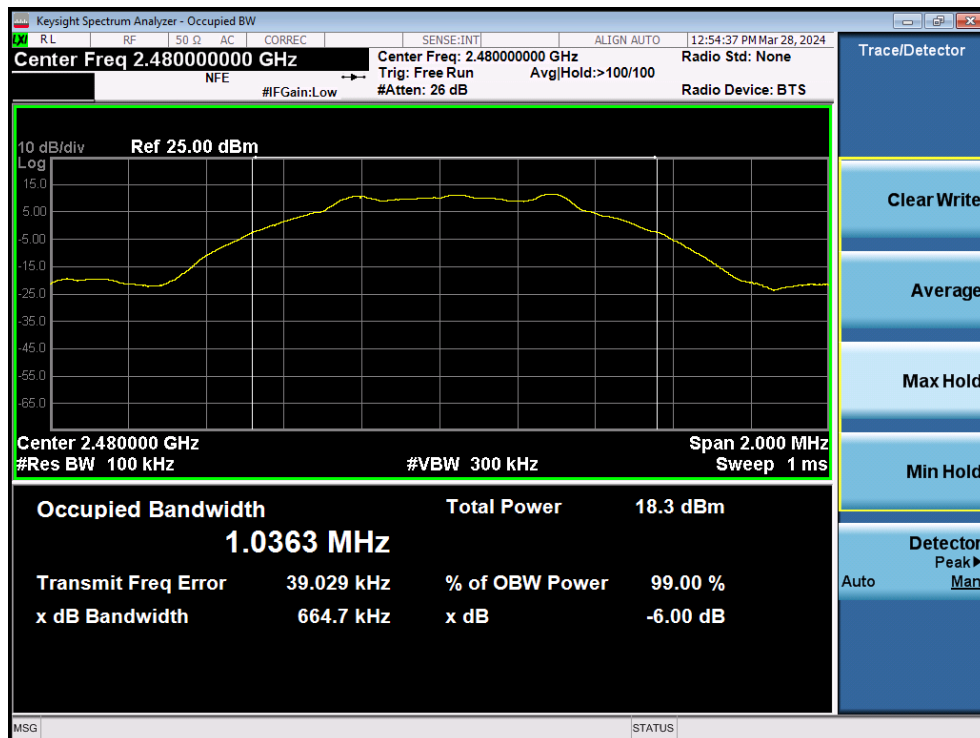
Plot 7-22. 6dB Bandwidth Plot (Bluetooth (LE), 1Mbps – Ch. 39 – Dual Ant1)
