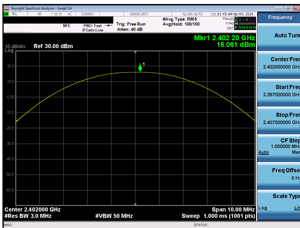
Plot 7-44. Peak Power Plot (Bluetooth (LE), 1Mbps – Ch. 0) – Ant2
