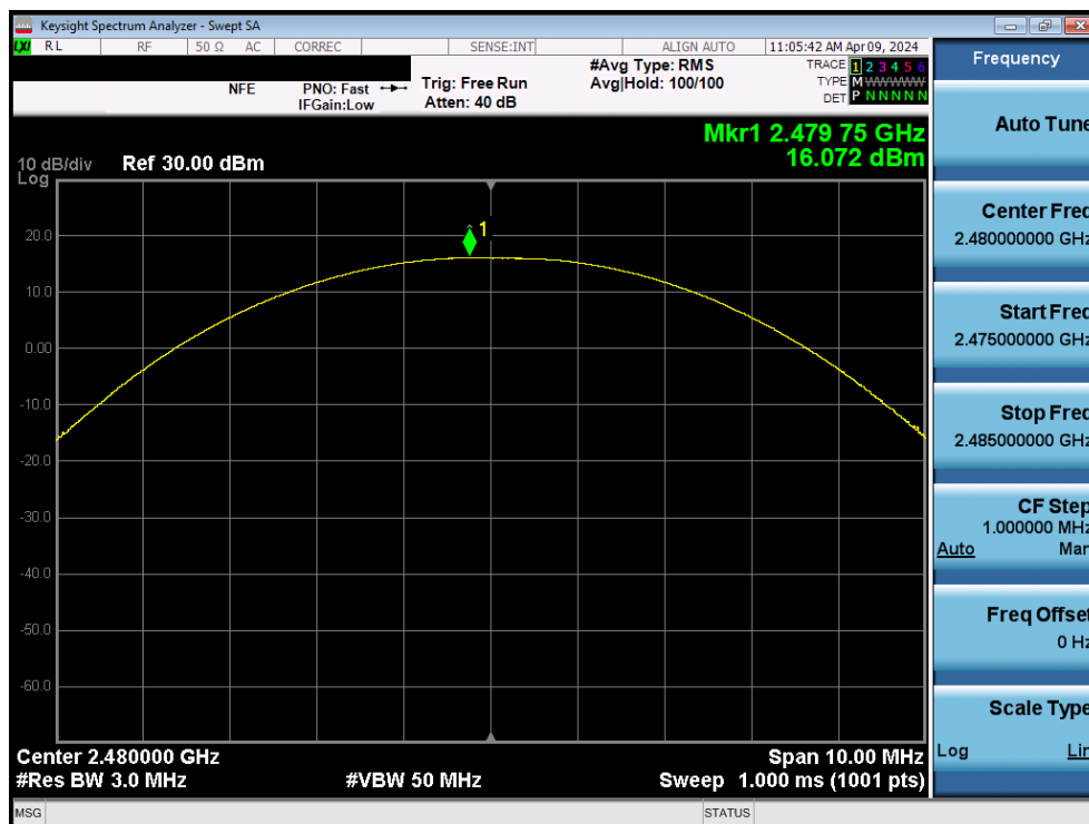
Plot 7-46. Peak Power Plot (Bluetooth (LE), 1Mbps – Ch. 39) – Ant2
