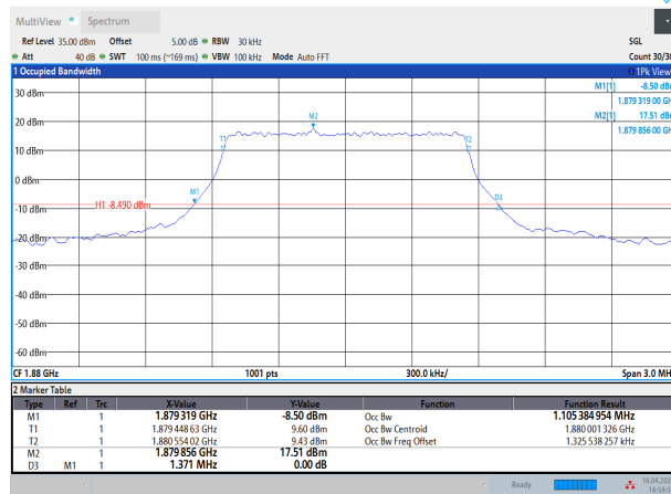
Band2-1.4MHz-QPSK-18900-6RB#0
