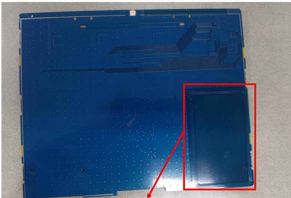
Receiving Antenna(NFC)
