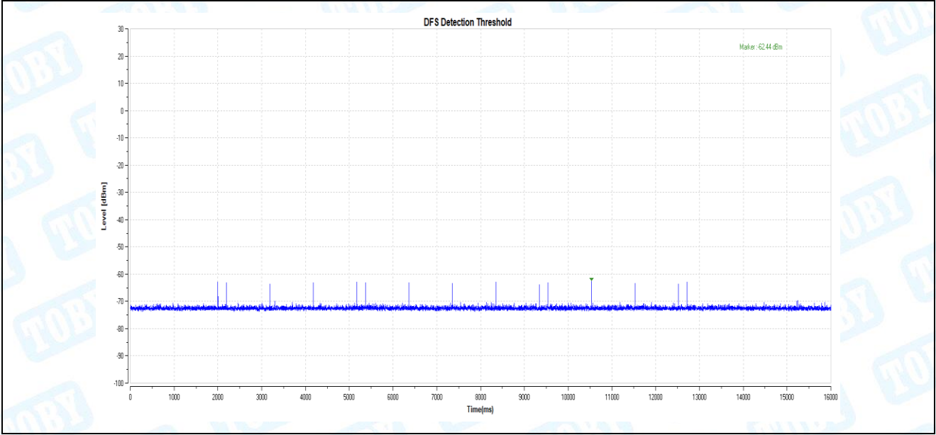
11AX160_5250_Type5
