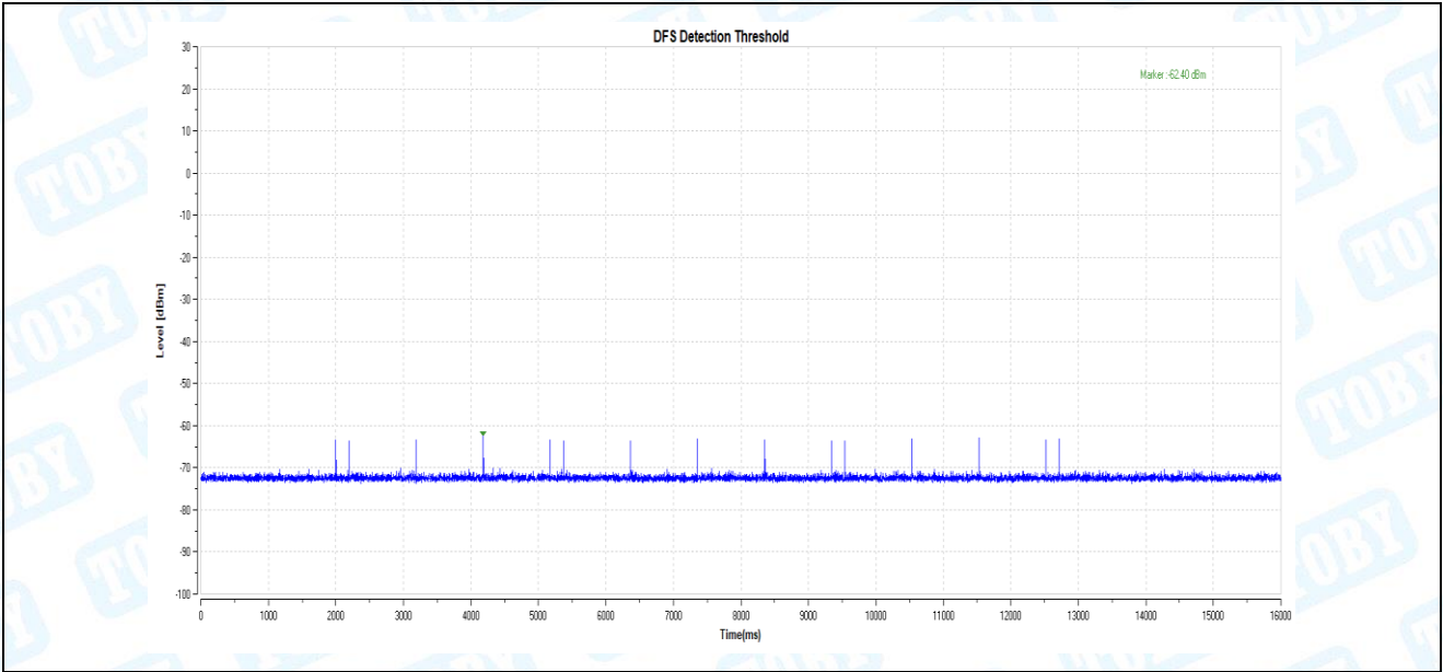
11AC80_5290_Type6
