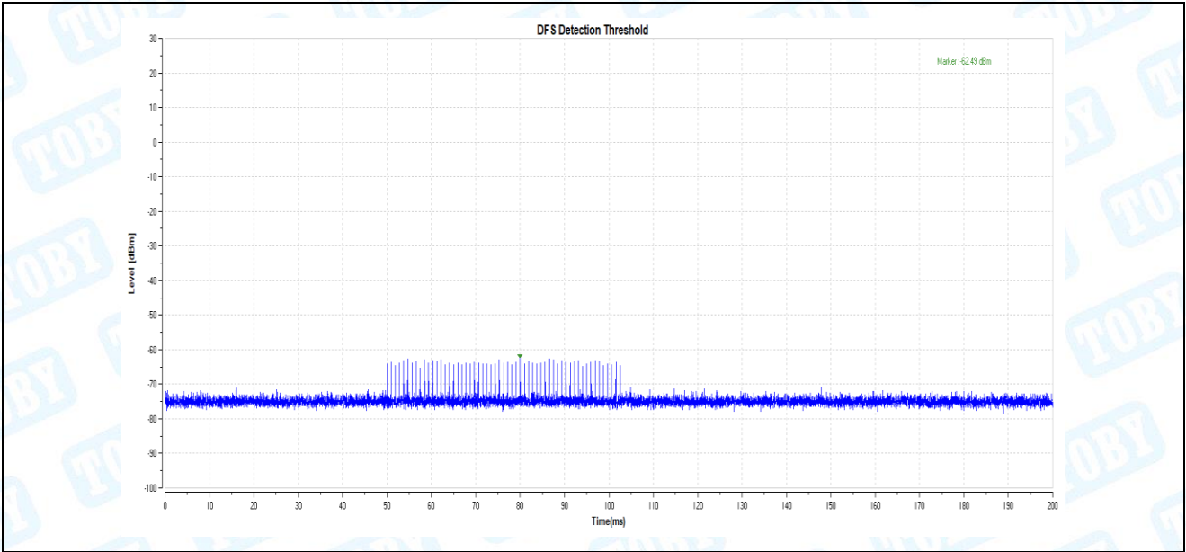
11AC80_5530_Type2
