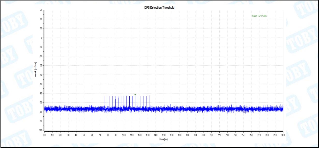
11AC80_5530_Type3
