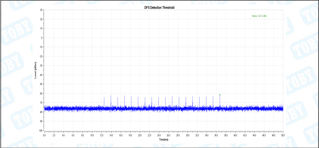
11AC80_5290_Type1
