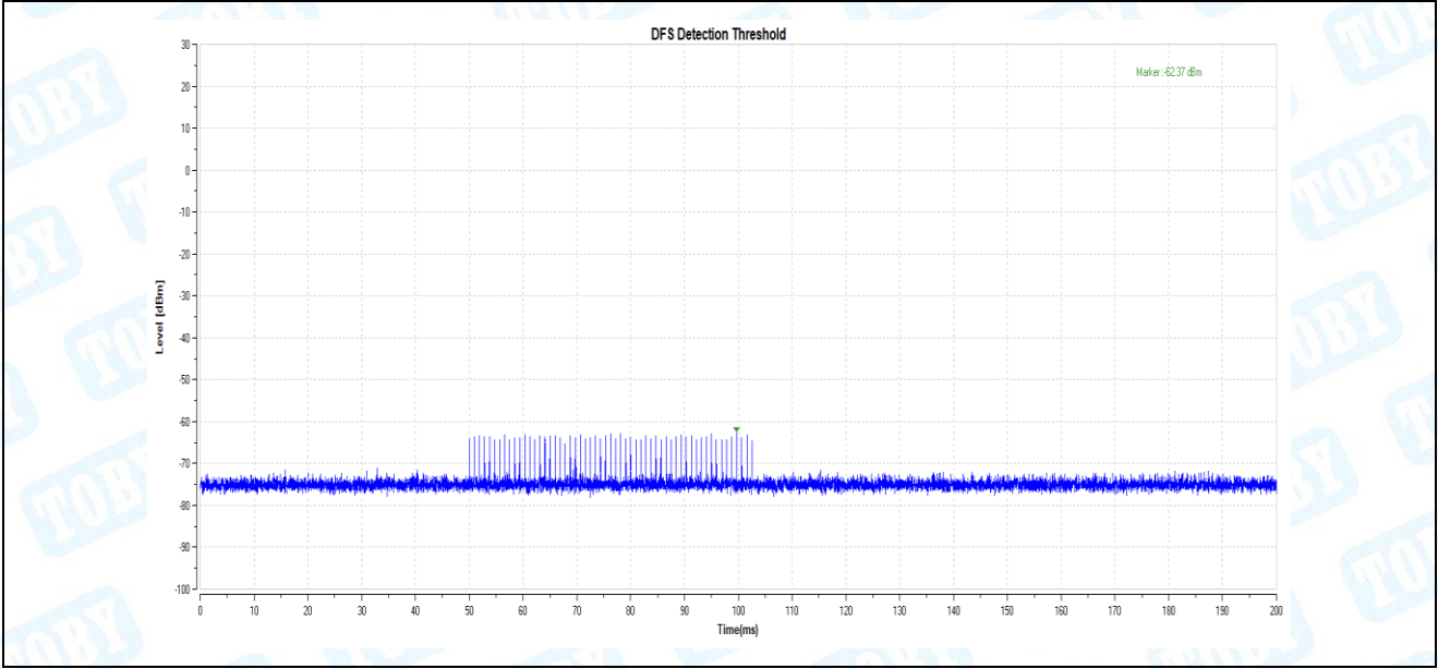
11AC80_5290_Type1
