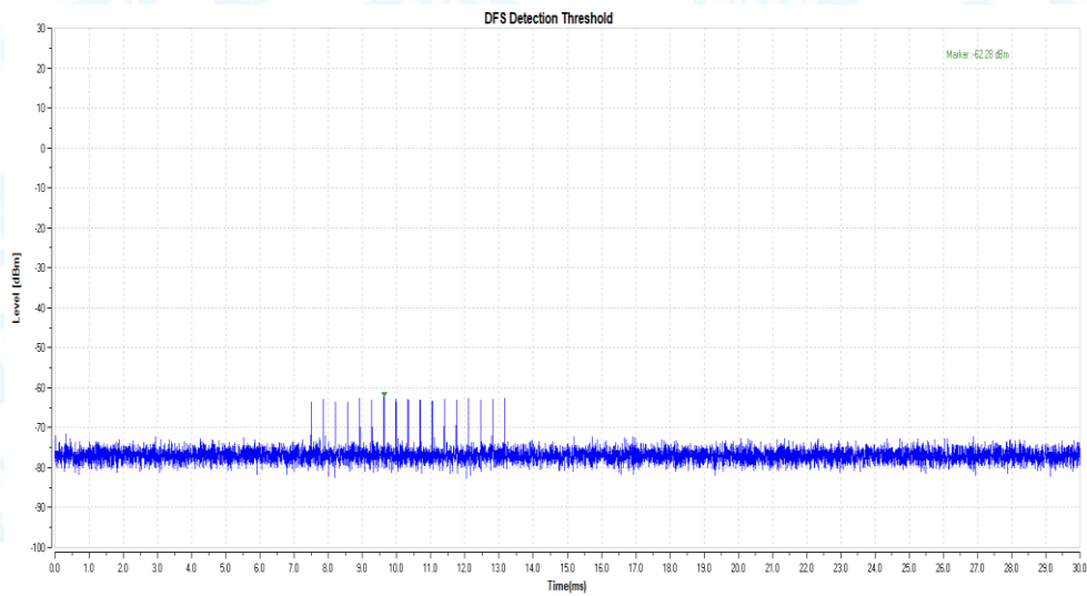
11AC80_5290_Type4
