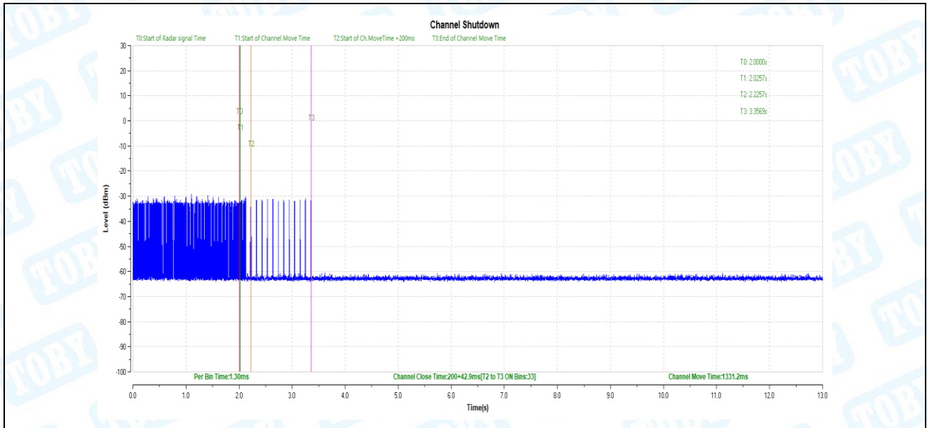
11AX160_5250
