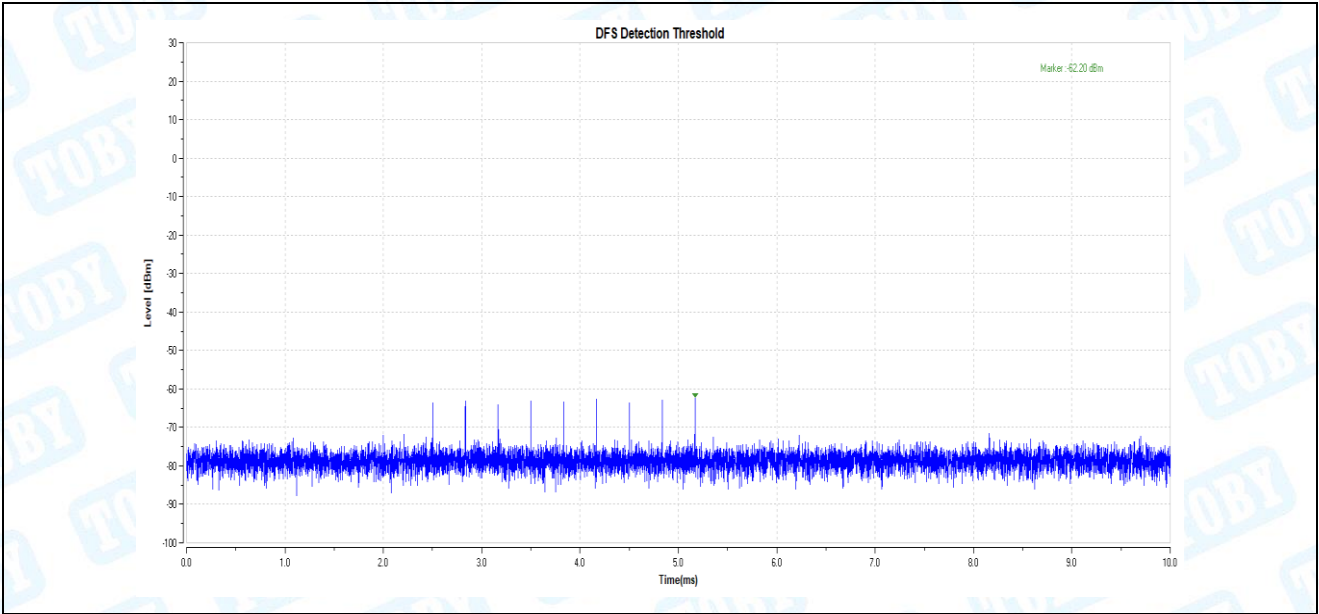
11AC80_5290_Type0
