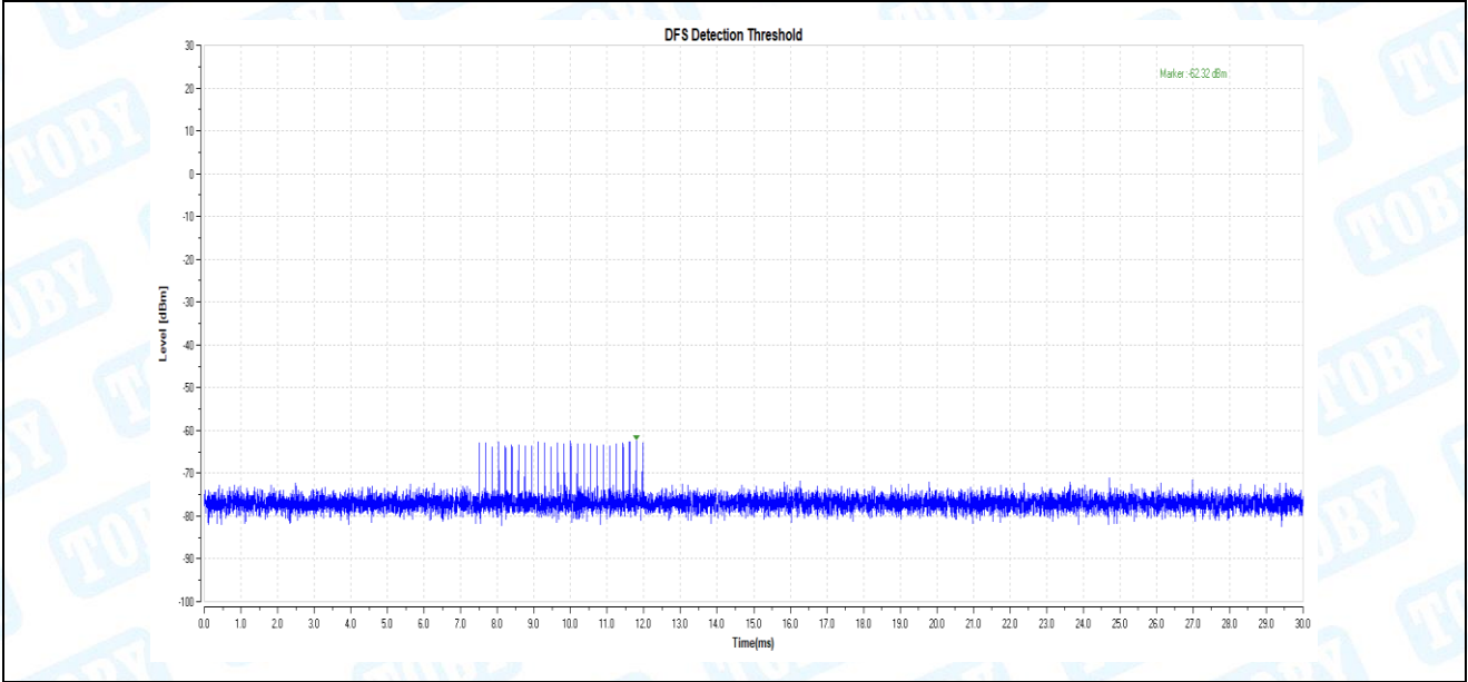
11AC80_5530_Type3
