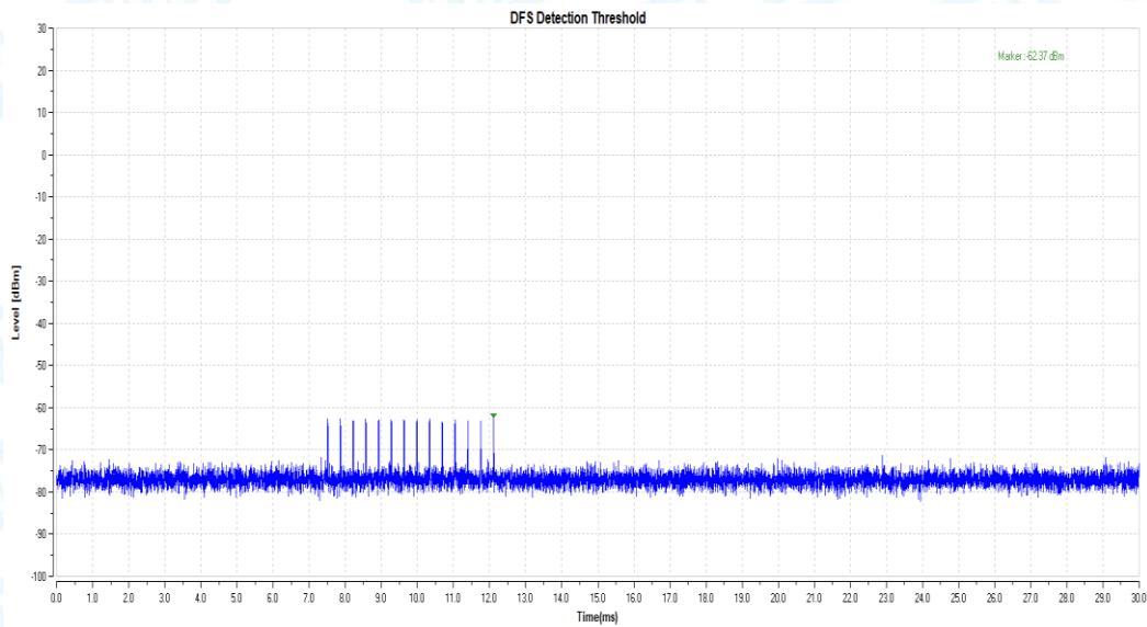
11AC80_5530_Type5
