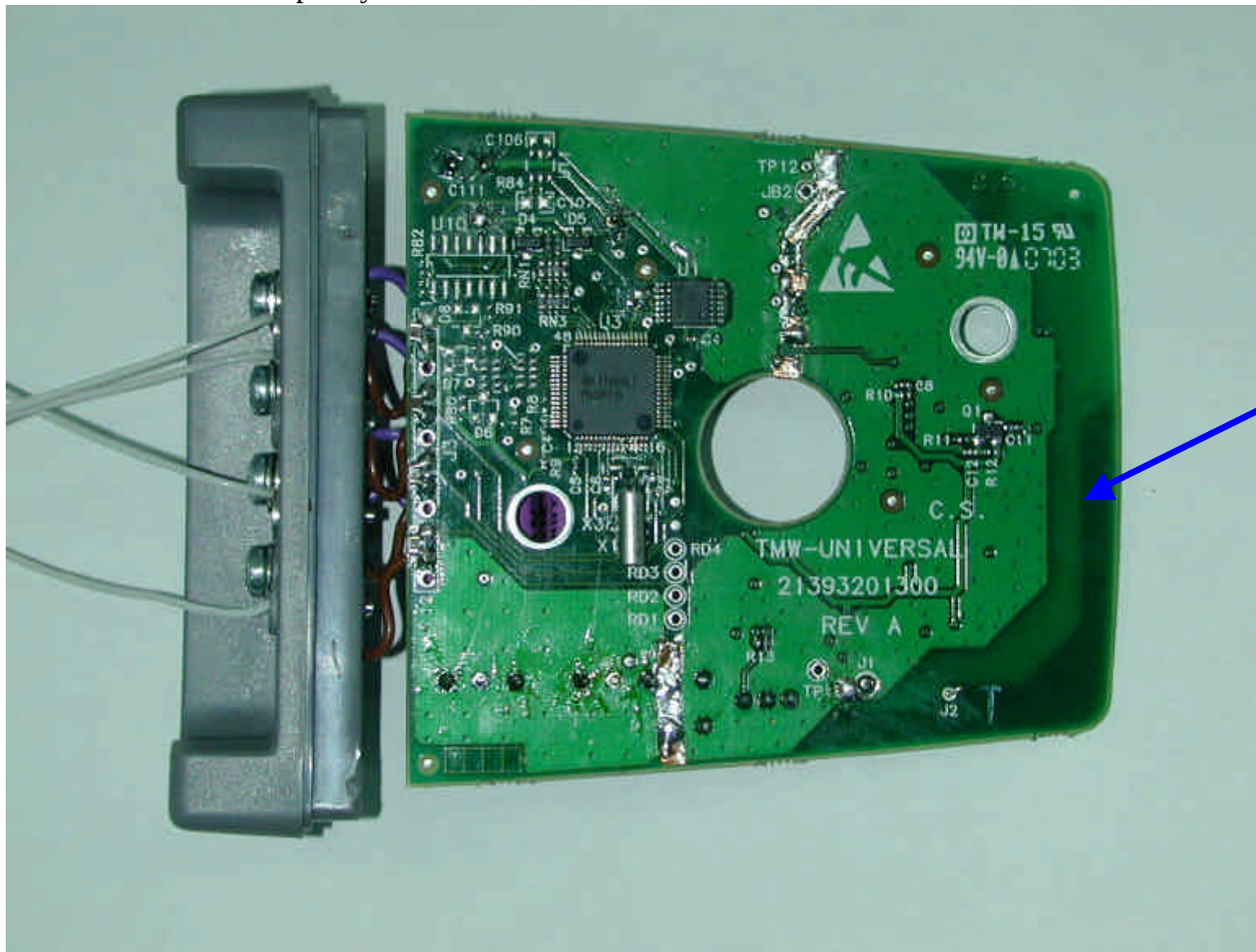
PCB side 1 without temporary antenna connector
