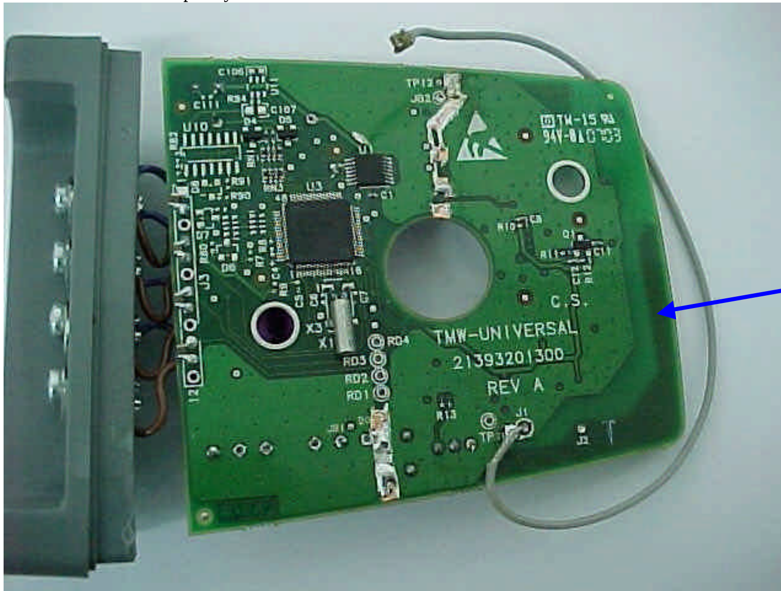
PCB first side with temporary antenna connector
