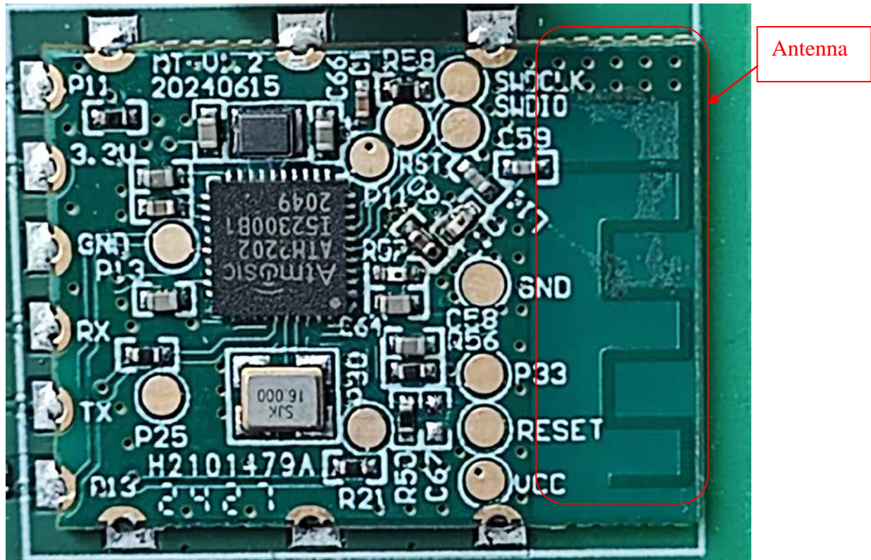
FIGURE 33 SWI331 WIRELESS (M/N: SWI331 WIRELESS-008) BOARD2-4
