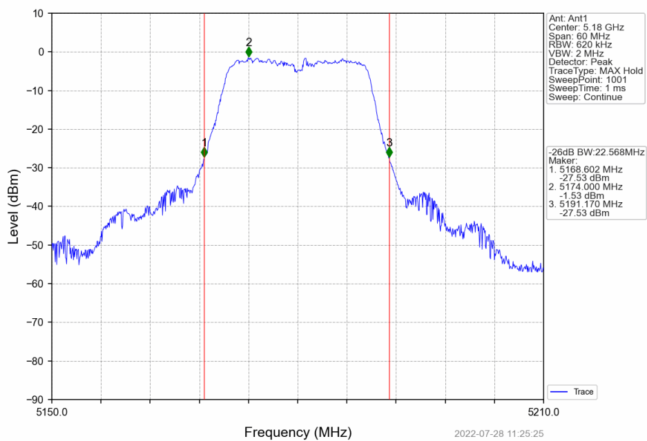
802.11ac(VHT20)_LCH_5180MHz_Ant1_NTN
