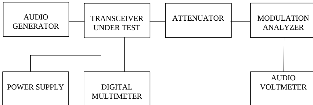
TEST SET-UP
