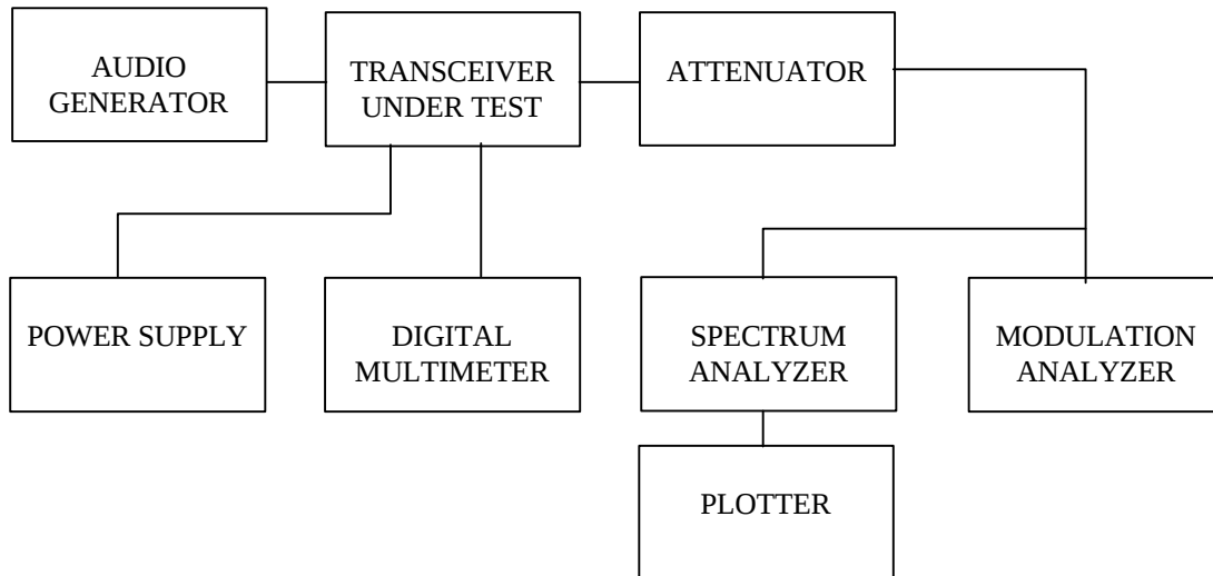
TEST SET-UP
