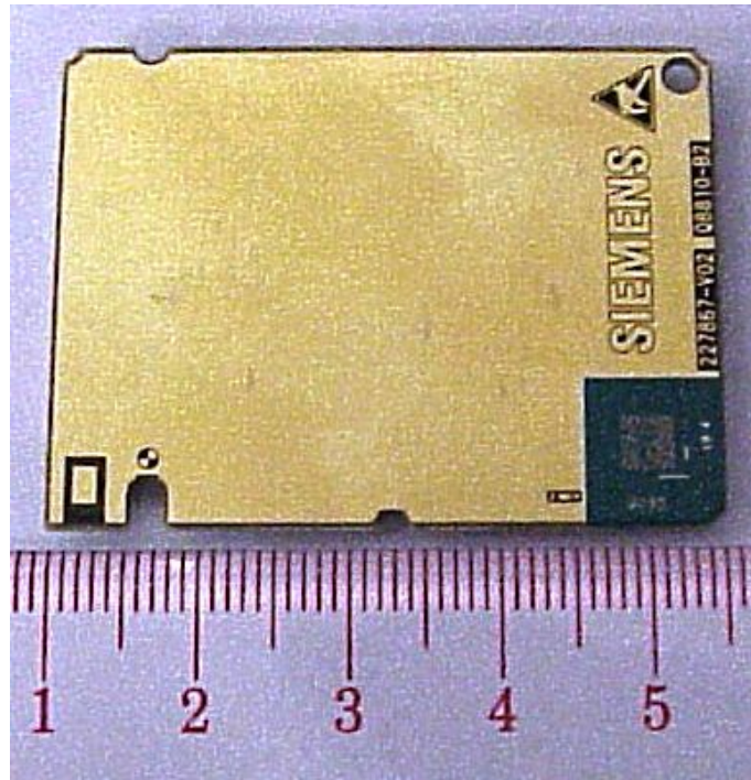
TC63 Top side
