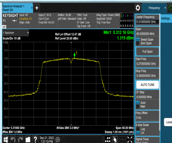
11N40SISO_Ant1_5310
