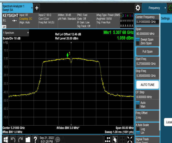
11AC40SISO_Ant1_5310
