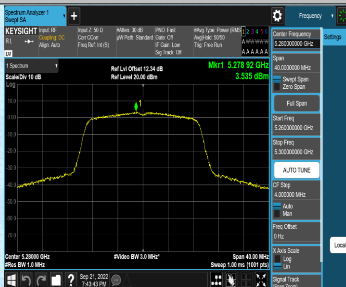
11AC20SISO_Ant1_5280
