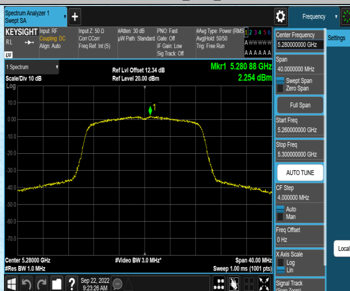
11AC20SISO_Ant2_5280
