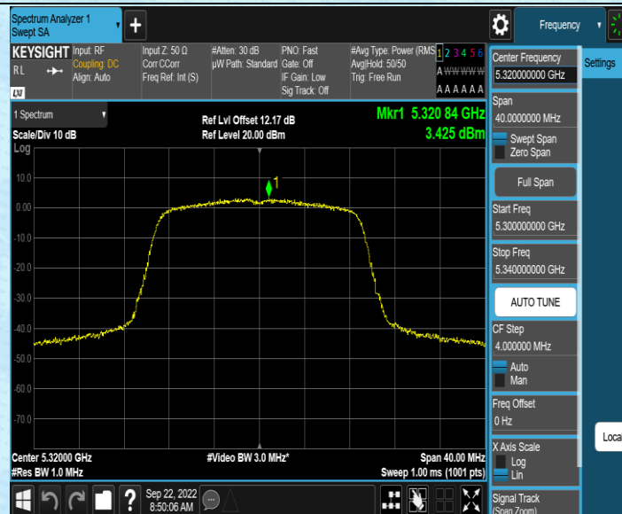
11N20SISO_Ant2_5320
