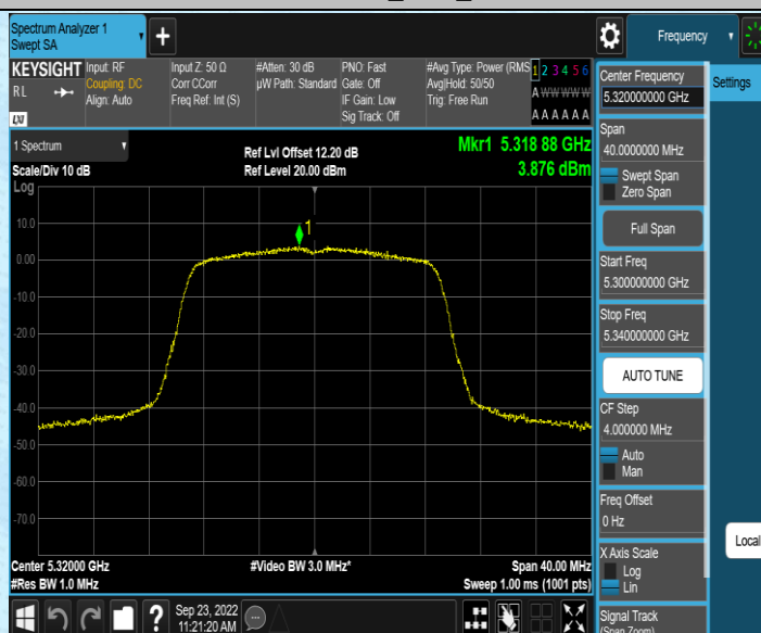
11N20SISO_Ant1_5320
