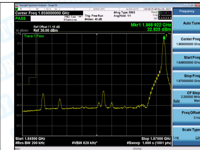
Band2_20MHz_16QAM_18700_1RB#99
