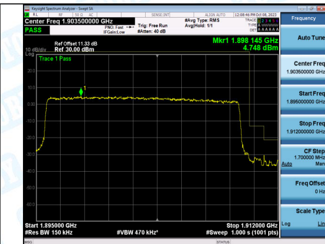
Band2_15MHz_QPSK_19125_75RB#0
