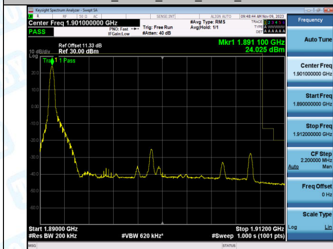
Band2_20MHz_QPSK_19100_1RB#0
