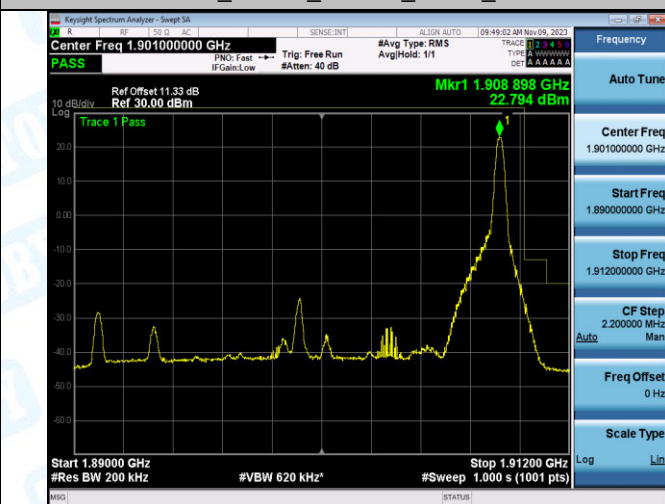
Band2_20MHz_16QAM_19100_1RB#99
