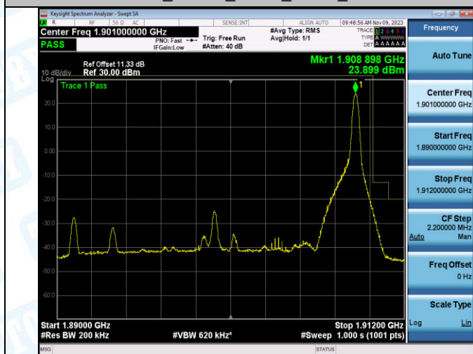
Band2_20MHz_QPSK_19100_1RB#99
