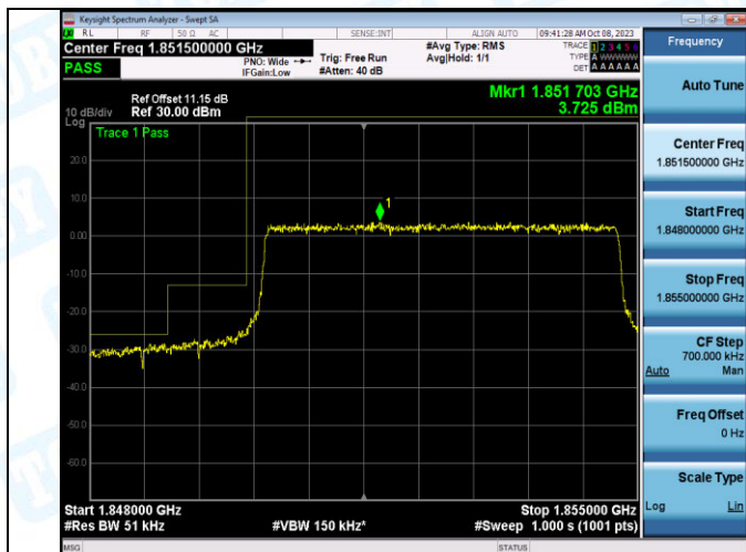
Band2_5MHz_QPSK_18625_25RB#0
