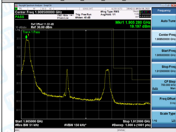
Band2_5MHz_QPSK_19175_1RB#0
