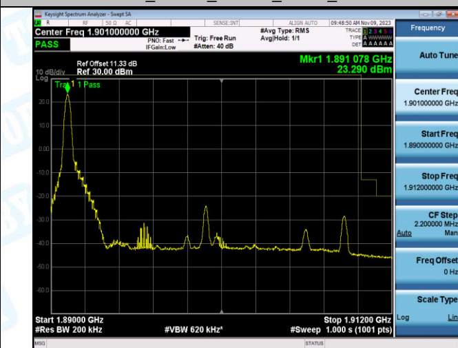
Band2_20MHz_16QAM_19100_1RB#0
