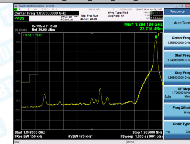
Band2_15MHz_16QAM_18675_1RB#74
