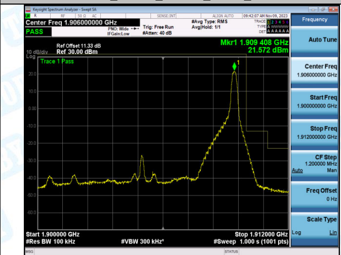
Band2_10MHz_16QAM_19150_1RB#49
