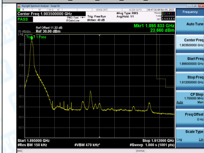
Band2_15MHz_QPSK_19125_1RB#0
