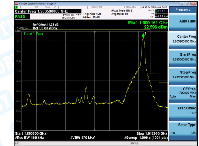
Band2_15MHz_16QAM_19125_1RB#74
