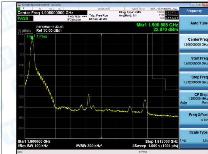
Band2_10MHz_QPSK_19150_1RB#0
