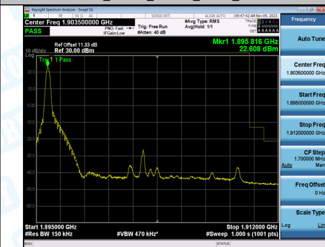
Band2_15MHz_16QAM_19125_1RB#0
