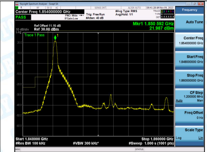
Band2_10MHz_16QAM_18650_1RB#0
