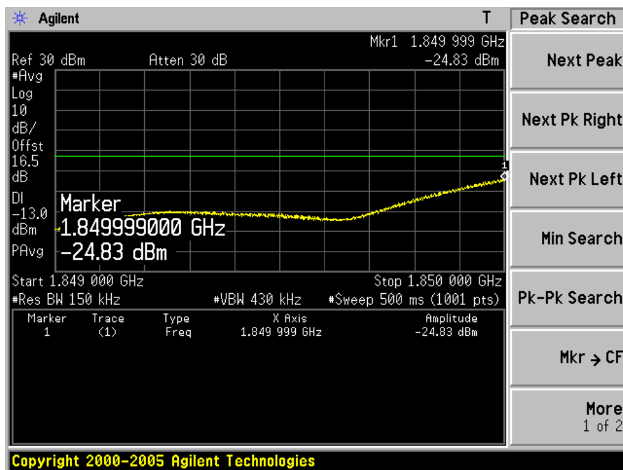
Figure Channel 26115 (1857.50MHz)
