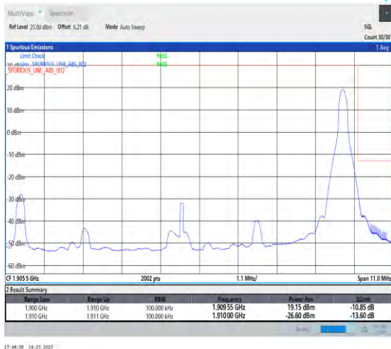
1-N2-PC3-15-10-H-2-DFT-PI2BPSK-Edge_1RB_Right-1@51-Ant3-1-seegraph-PASS-see graph
