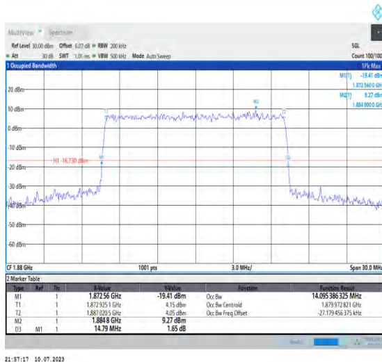
1-N2-PC3-15-15-M-9-CP-256QAM-Outer_Full-79@0- Ant3-14.095-14.790-≤15-PASS
