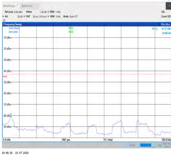
1-N2-PC3-15-20-H-1-DFT-PI2BPSK-Inner_1RB_Lef t-1@1-0.009-0.15-Ant3-0.02--81.97--43-PASS
