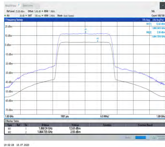
1-N2-PC3-15-20-L-2-CP-256QAM-Outter_Full-106@ 0-Ant3-9.70-100%-0.00-9.70-PASS-≤13
