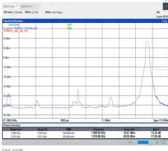
1-N2-PC3-15-10-H-5-CP-QPSK-Edge_1RB_Right-1@51-Ant3-1-seegraph-PASS-see graph
