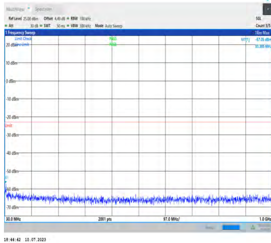
1-N2-PC3-15-20-M-1-DFT-PI2BPSK-Inner_1RB_Lef t-1@1-30-1000-Ant3-33.40--57.05--23-PASS
