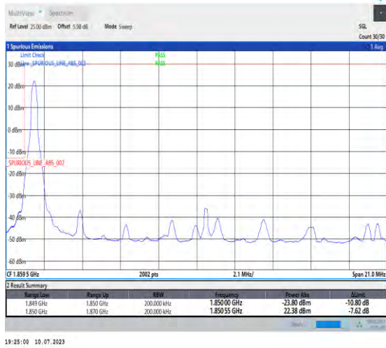
1-N2-PC3-15-20-L-1-DFT-PI2BPSK-Edge_1RB_Left-1@0-Ant3-1-seegraph-PASS-see graph
