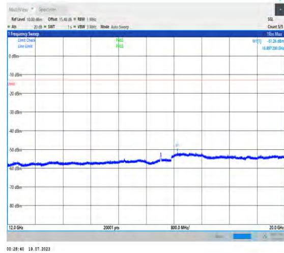
1-N2-PC3-15-20-H-1-DFT-PI2BPSK-Inner_1RB_Left- t-1@1-12000-20000-Ant3-16897.20--51.26--13-PASS
