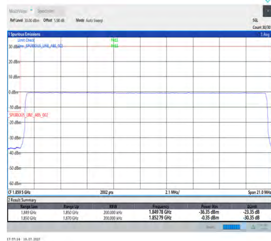
1-N2-PC3-15-20-L-6-CP-QPSK-Outer_Full-106@0-Ant3-1-seegraph-PASS-see graph
