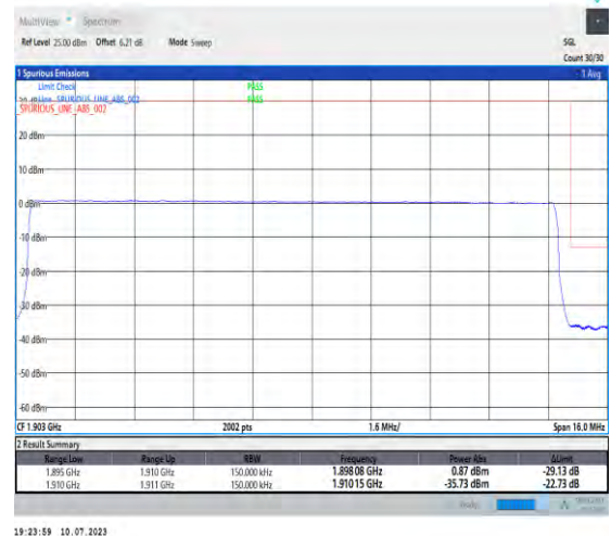
1-N2-PC3-15-15-H-6-CP-QPSK-Outer_Full-79@0-Ant3-1-seegraph-PASS-see graph
