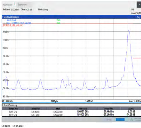
1-N2-PC3-15-15-H-2-DFT-PI2BPSK-Edge_1RB_Right-1@78-Ant3-1-seegraph-PASS-see graph
