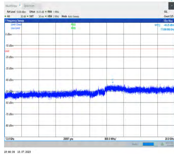
1-N2-PC3-15-20-L-1-DFT-PI2BPSK-Inner_1RB_Left- 1@1-12000-20000-Ant3-17088.00--43.25--13-PASS
