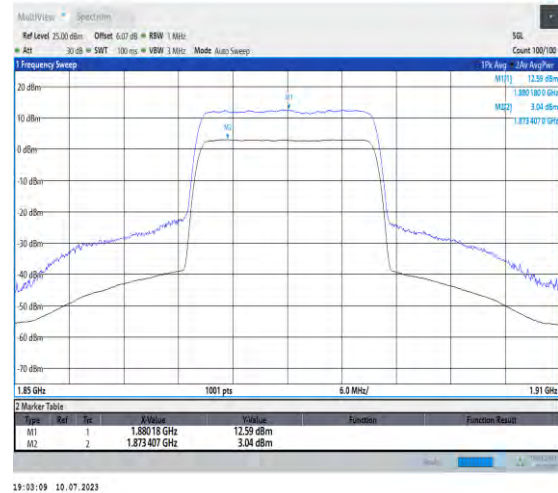
1-N2-PC3-15-20-M-2-CP-256QAM-Outter_Full-106 @0-Ant3-9.55-100%-0.00-9.55-PASS-≤13
