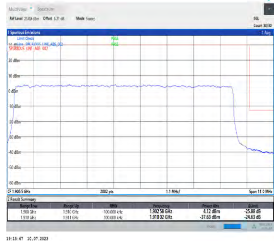
1-N2-PC3-15-10-H-3-DFT-PI2BPSK-Outer_Full-50@0-Ant3-1-seegraph-PASS-see graph
