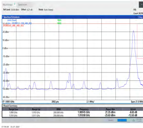
1-N2-PC3-15-20-H-2-DFT-PI2BPSK-Edge_1RB_Right-1@105-Ant3-1-seegraph-PASS-see graph
