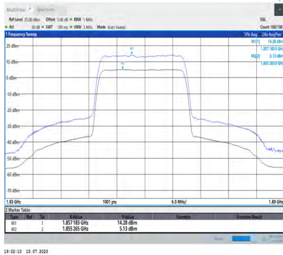
1-N2-PC3-15-20-L-1-DFT-256QAM-Outter_Full-100@ 0-Ant3-9.15-100%-0.00-9.15-PASS-≤13
