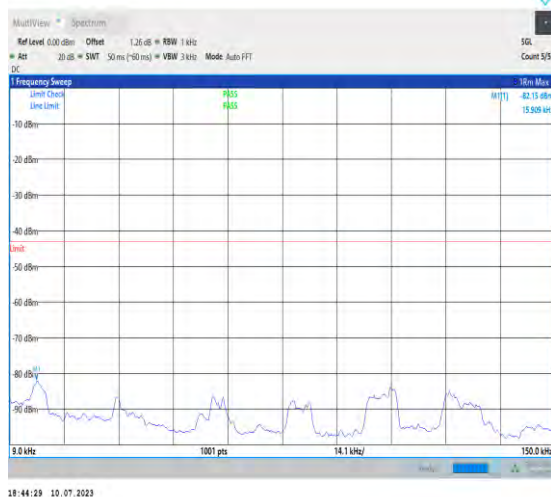
1-N2-PC3-15-20-M-1-DFT-PI2BPSK-Inner_1RB_Lef t-1@1-0.009-0.15-Ant3-0.02--82.15--43-PASS
