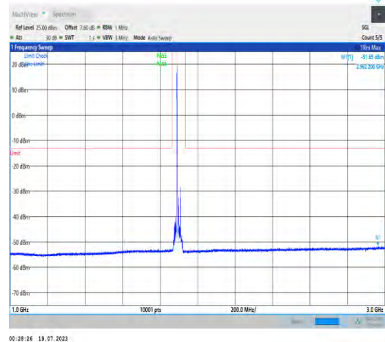
1-N2-PC3-15-20-H-1-DFT-PI2BPSK-Inner_1RB_Left -1@1-1000-3000-Ant3-2962.2--51.65--13-PASS
