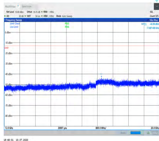
1-N2-PC3-15-20-M-1-DFT-PI2BPSK-Inner_1RB_Left- 1@1-12000-20000-Ant3-17007.60--43.38--13-PASS
