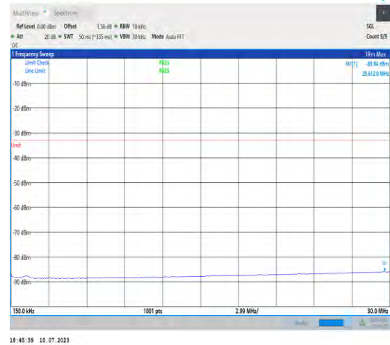
1-N2-PC3-15-20-H-1-DFT-PI2BPSK-Inner_1RB_Left- 1@1-0.15-30-Ant3-29.61--85.94--33-PASS
