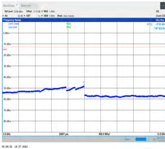
1-N2-PC3-15-20-H-1-DFT-PI2BPSK-Inner_1RB_Left- t-1@1-3000-12000-Ant3-7487.85--47.82--13-PASS
