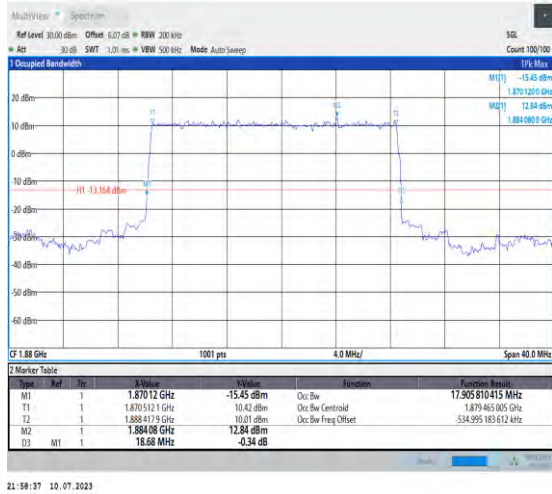
1-N2-PC3-15-20-M-2-DFT-PI2BPSK-Outter_Full-100 @0-Ant3-17.906-18.680-≤20-PASS
