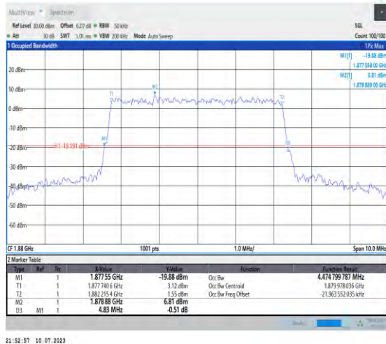
1-N2-PC3-15-5-M-9-CP-256QAM-Outer_Full-25@0- Ant3-4.475-4.830-≤5-PASS
