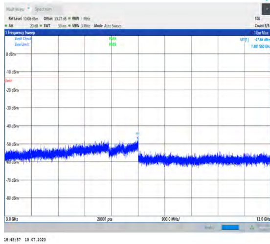
1-N2-PC3-15-20-H-1-DFT-PI2BPSK-Inner_1RB_Left- t-1@1-3000-12000-Ant3-7481.55--47.65--13-PASS
