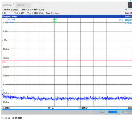
1-N2-PC3-15-20-L-1-DFT-PI2BPSK-Inner_1RB_Left -1@1-30-1000-Ant3-30.97--59.66--23-PASS
