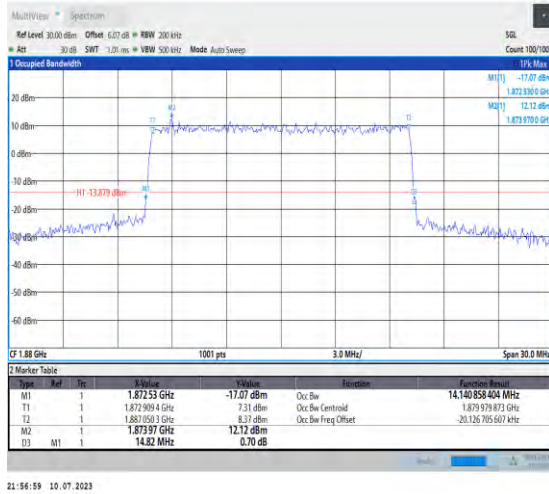
1-N2-PC3-15-15-M-7-CP-16QAM-Outer_Full-79@0- Ant3-14.141-14.820-≤15-PASS
