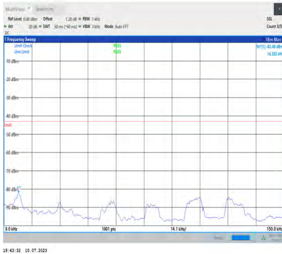
1-N2-PC3-15-20-L-1-DFT-PI2BPSK-Inner_1RB_Left -1@1-0.009-0.15-Ant3-0.02--82.48--43-PASS
