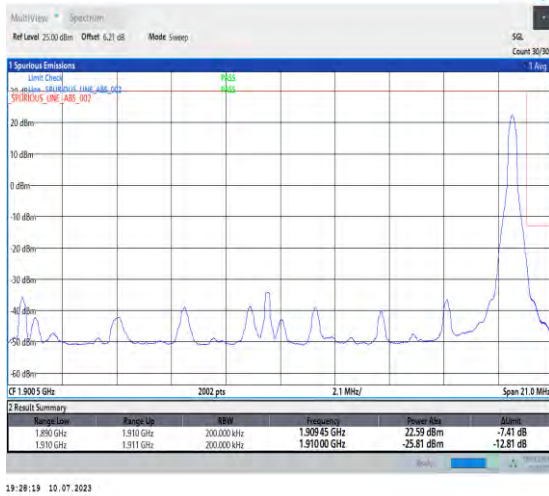
1-N2-PC3-15-20-H-2-DFT-PI2BPSK-Edge_1RB_Right-1@105-Ant3-1-seegraph-PASS-see graph
