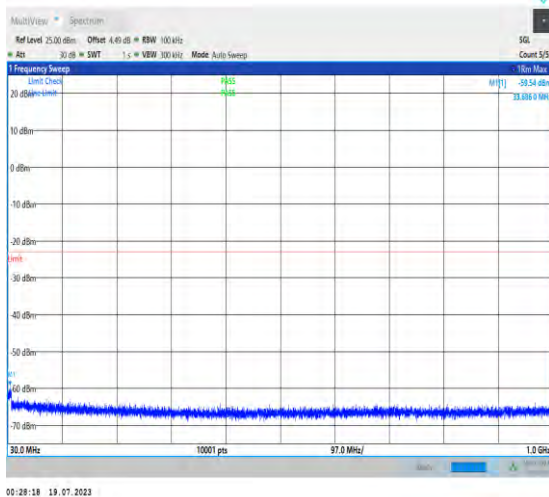
1-N2-PC3-15-20-H-1-DFT-PI2BPSK-Inner_1RB_Left -1@1-30-1000-Ant3-33.686--59.54--23-PASS
