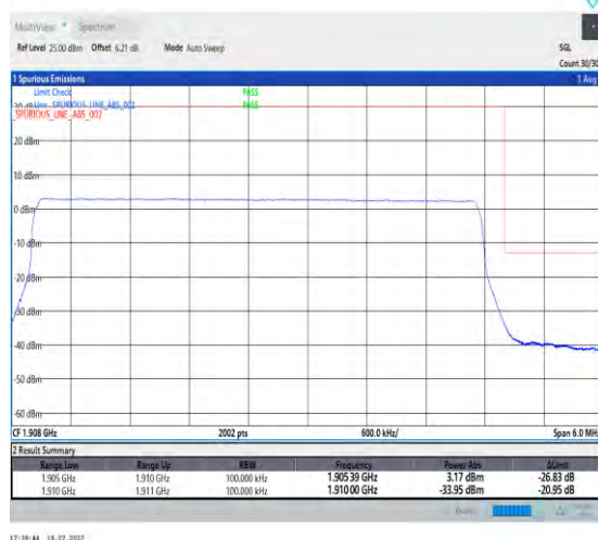
1-N2-PC3-15-5-H-6-CP-QPSK-Outer_Full-25@0-Ant3-1-seegraph-PASS-see graph
