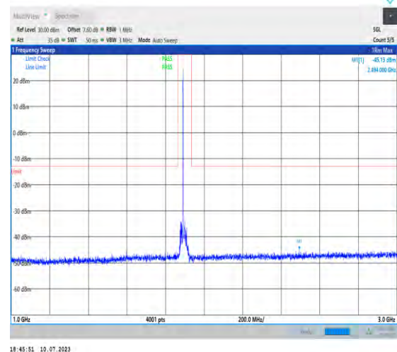
1-N2-PC3-15-20-H-1-DFT-PI2BPSK-Inner_1RB_Left- 1@1-1000-3000-Ant3-2494.00--45.13--13-PASS
