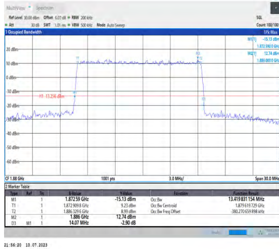
1-N2-PC3-15-15-M-3-DFT-16QAM-Outer_Full-75@0-Ant3-13.42-14.070-≤15-PASS
