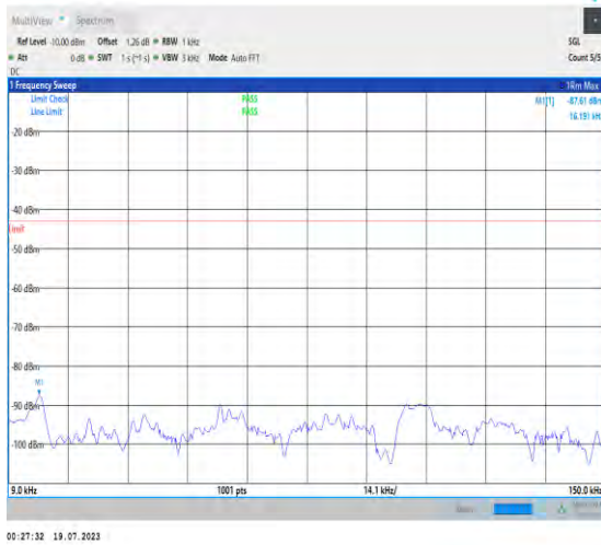
1-N2-PC3-15-20-H-1-DFT-PI2BPSK-Inner_1RB_Left -1@1-0.009-0.15-Ant3-16.191--87.61--43-PASS
