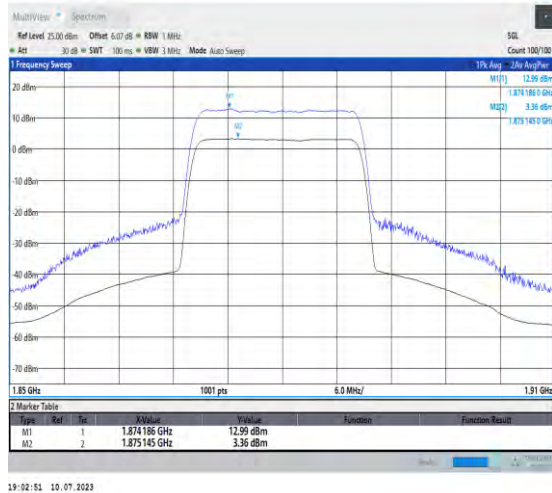
1-N2-PC3-15-20-M-1-DFT-256QAM-Outter_Full-100 @0-Ant3-9.63-100%-0.00-9.63-PASS-≤13
