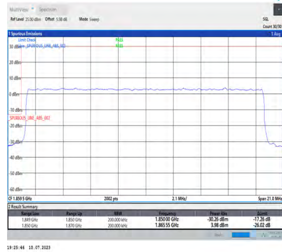
1-N2-PC3-15-20-L-3-DFT-PI2BPSK-Outer_Full-100@0-Ant3-1-seegraph-PASS-see graph
