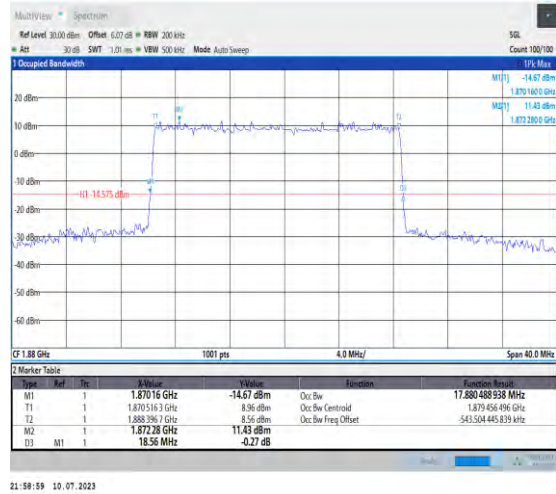
1-N2-PC3-15-20-M-3-DFT-16QAM-Outter_Full-100@ 0-Ant3-17.88-18.560-≤20-PASS
