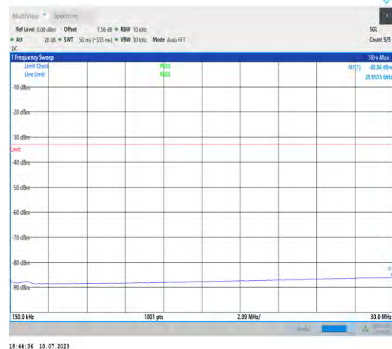
1-N2-PC3-15-20-M-1-DFT-PI2BPSK-Inner_1RB_Left- 1@1-0.15-30-Ant3-29.91--85.94--33-PASS
