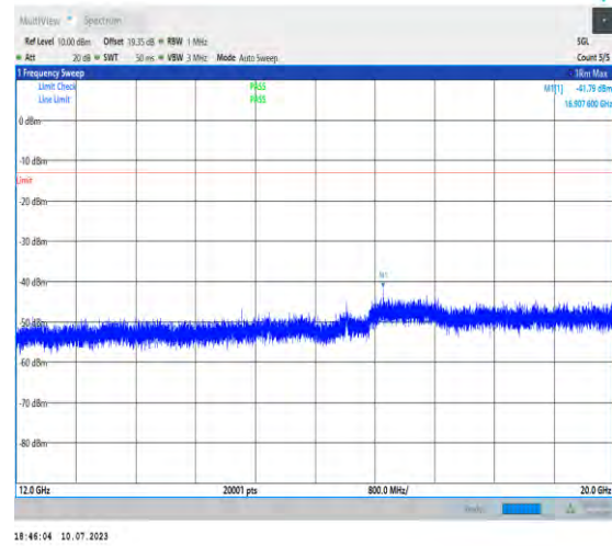
1-N2-PC3-15-20-H-1-DFT-PI2BPSK-Inner_1RB_Left- t-1@1-12000-20000-Ant3-16907.60--41.79--13-PASS
