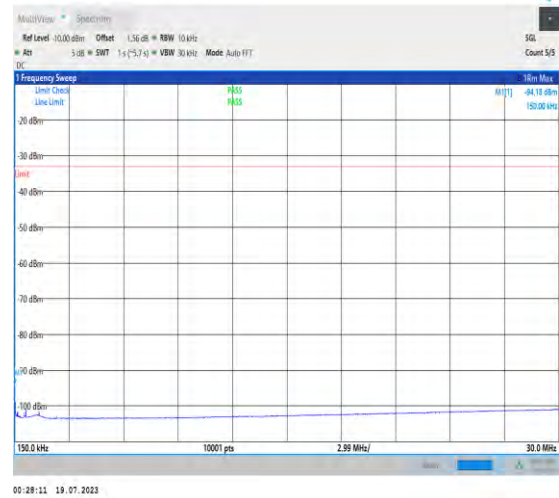
1-N2-PC3-15-20-H-1-DFT-PI2BPSK-Inner_1RB_Left -1@1-0.15-30-Ant3-150--94.18--33-PASS
