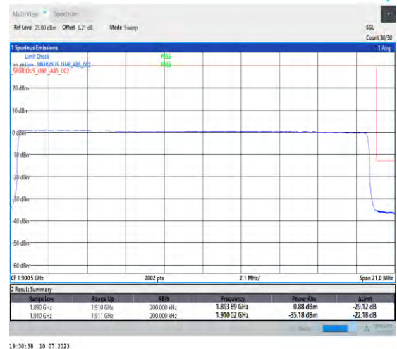
1-N2-PC3-15-20-H-6-CP-QPSK-Outer_Full-106@0-Ant3-1-seegraph-PASS-see graph
