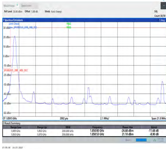
1-N2-PC3-15-20-L-1-DFT-PI2BPSK-Edge_1RB_Left-1@0-Ant3-1-seegraph-PASS-see graph
