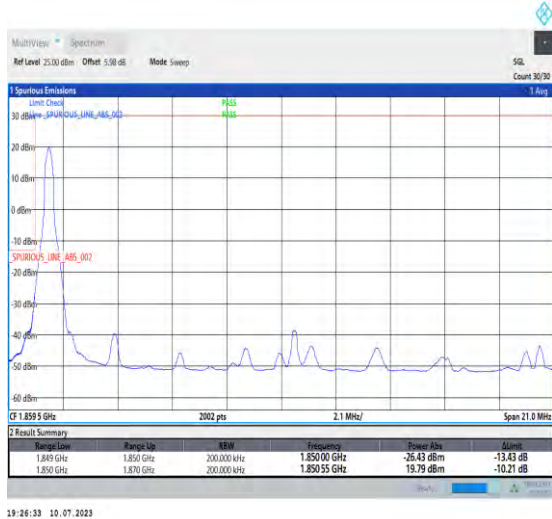
1-N2-PC3-15-20-L-4-CP-QPSK-Edge_1RB_Left-1@0-Ant3-1-seegraph-PASS-see graph
