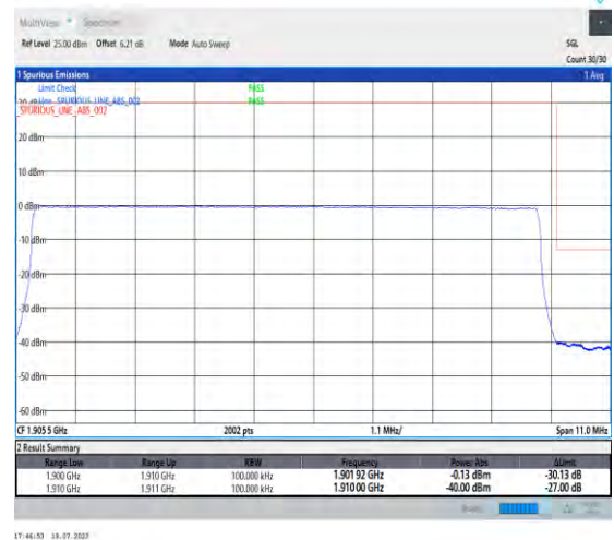
1-N2-PC3-15-10-H-6-CP-QPSK-Outer_Full-52@0-Ant3-1-seegraph-PASS-see graph
