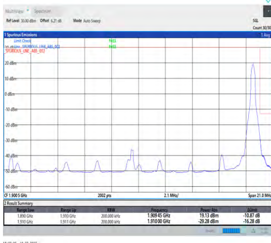
1-N2-PC3-15-20-H-5-CP-QPSK-Edge_1RB_Right-1@105-Ant3-1-seegraph-PASS-see graph
