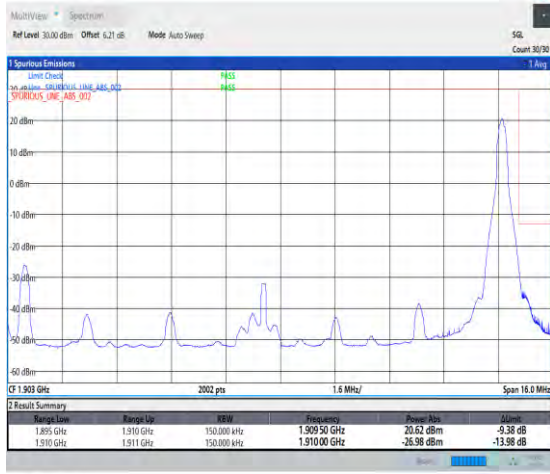
1-N2-PC3-15-15-H-2-DFT-PI2BPSK-Edge_1RB_Right-1@78-Ant3-1-seegraph-PASS-see graph
