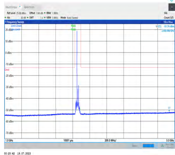
1-N2-PC3-15-20-L-1-DFT-PI2BPSK-Inner_1RB_Left -1@1-1000-3000-Ant3-2935--51.74--13-PASS
