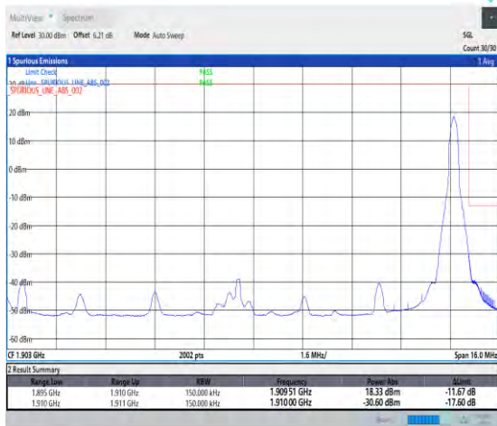
1-N2-PC3-15-15-H-5-CP-QPSK-Edge_1RB_Right-1@78-Ant3-1-seegraph-PASS-see graph
