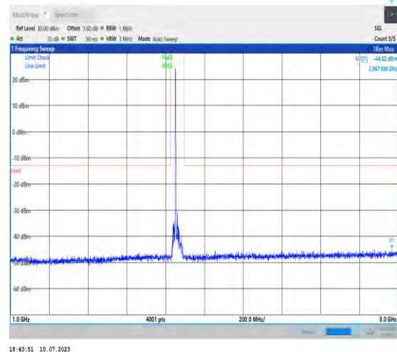
1-N2-PC3-15-20-L-1-DFT-PI2BPSK-Inner_1RB_Left- 1@1-1000-3000-Ant3-2967.50--44.82--13-PASS
