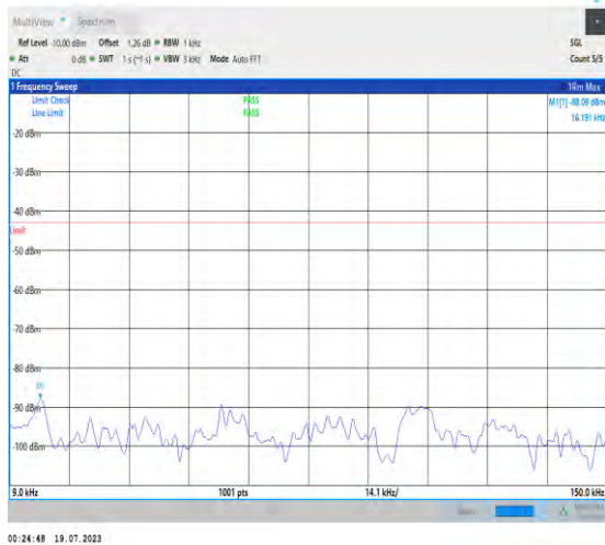
1-N2-PC3-15-20-L-1-DFT-PI2BPSK-Inner_1RB_Left -1@1-0.009-0.15-Ant3-16.191--88.09--43-PASS
