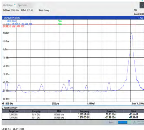
1-N2-PC3-15-15-H-5-CP-QPSK-Edge_1RB_Right-1@78-Ant3-1-seegraph-PASS-see graph
