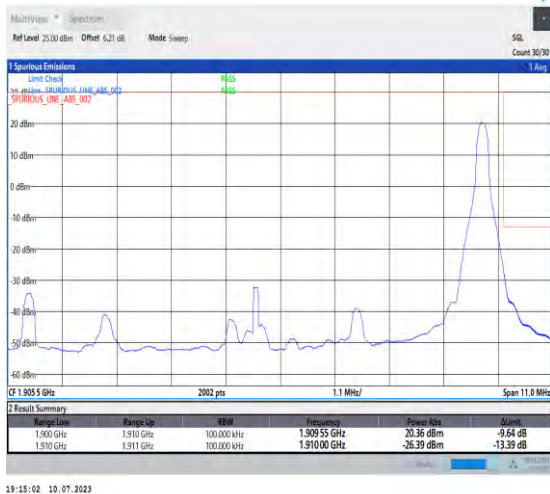
1-N2-PC3-15-10-H-2-DFT-PI2BPSK-Edge_1RB_Right-1@51-Ant3-1-seegraph-PASS-see graph
