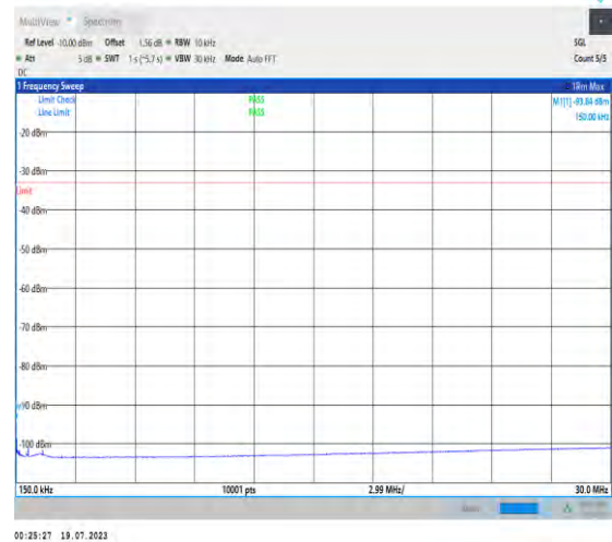
1-N2-PC3-15-20-L-1-DFT-PI2BPSK-Inner_1RB_Left -1@1-0.15-30-Ant3-150--93.84--33-PASS
