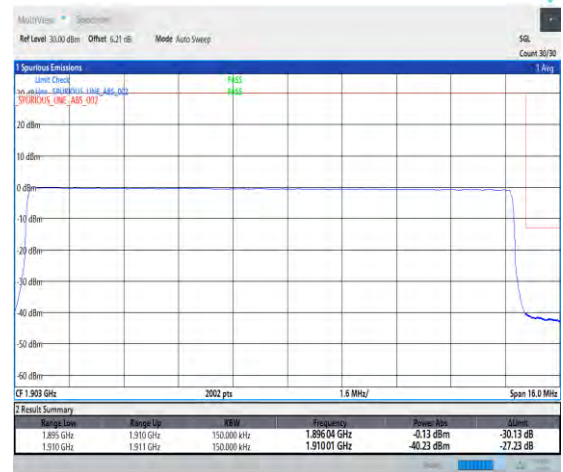
1-N2-PC3-15-15-H-6-CP-QPSK-Outer_Full-79@0-Ant3-1-seegraph-PASS-see graph
