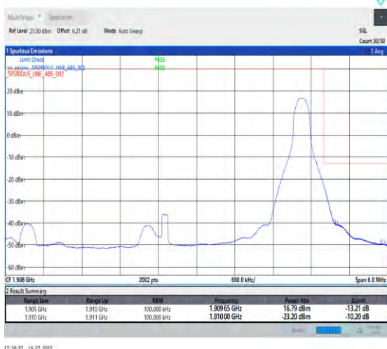
1-N2-PC3-15-5-H-5-CP-QPSK-Edge_1RB_Right-1@24-Ant3-1-seegraph-PASS-see graph
