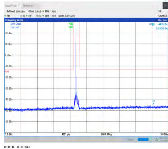
1-N2-PC3-15-20-M-1-DFT-PI2BPSK-Inner_1RB_Left- 1@1-1000-3000-Ant3-2818.00--44.83--13-PASS
