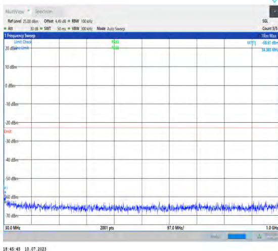
1-N2-PC3-15-20-H-1-DFT-PI2BPSK-Inner_1RB_Lef t-1@1-30-1000-Ant3-34.37--58.61--23-PASS
