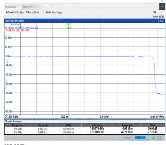
1-N2-PC3-15-20-H-6-CP-QPSK-Outer_Full-106@0-Ant3-1-seegraph-PASS-see graph
