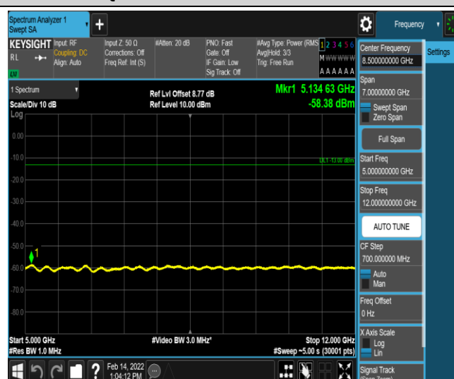
Band2-1.4MHz-QPSK-18607-1-0-Low-5000-12000--58.38-PASS
