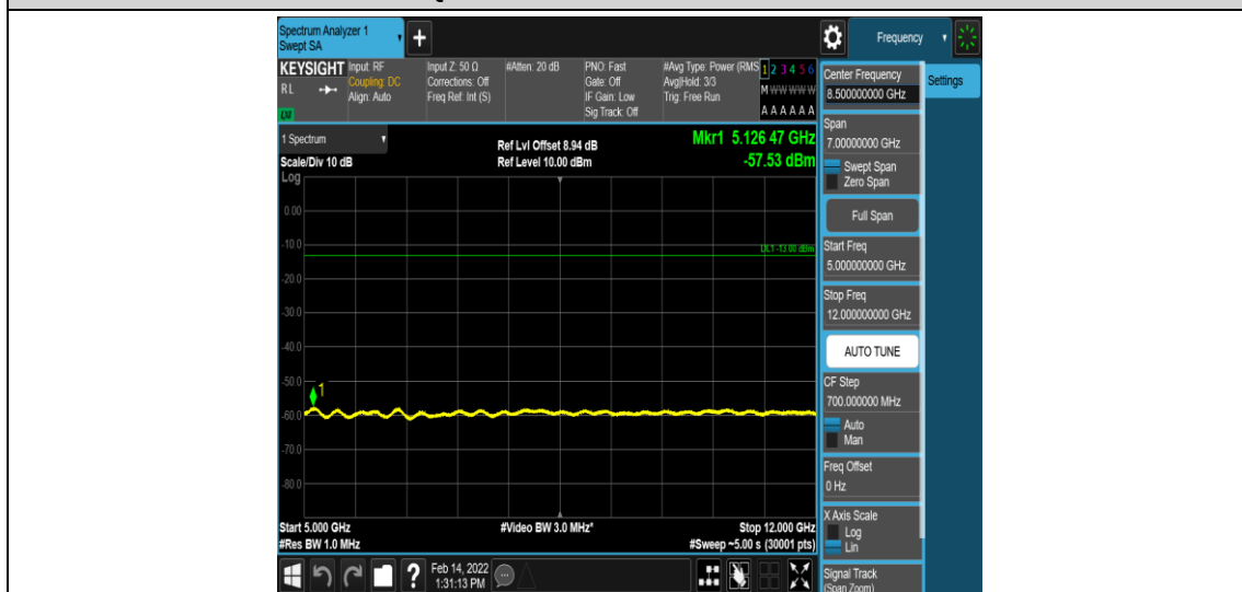
Band2-1.4MHz-QPSK-19193-6-0-Low-5000-12000--57.53-PASS
