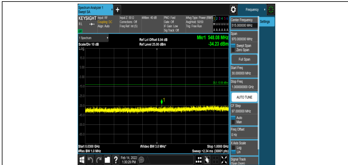
Band2-1.4MHz-QPSK-19193-6-0-Low-30-1000--34.23-PASS
