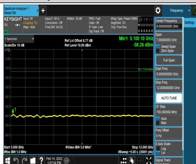
Band2-1.4MHz-QPSK-18607-6-0-Low-5000-12000--58.26-PASS
