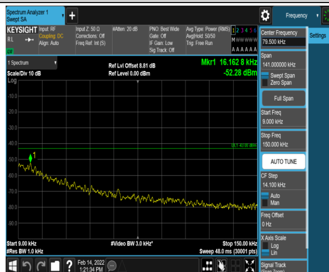
Band2-1.4MHz-QPSK-18900-1-0-Low-0.009-0.15--52.28-PASS
