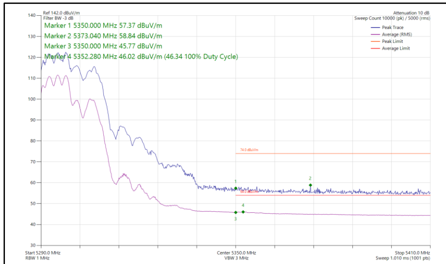
Figure 58 - 802.11ax HE20, RU 106-53, CDD, Core 0 - Core 1 - 5300 MHz Band Edge Frequency 5350 MHz
