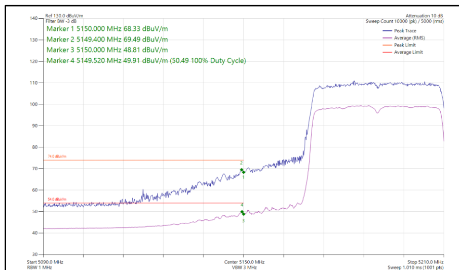
Figure 91 - 802.11ax HE40, SU, SISO, Core 0 - 5190 MHz Band Edge Frequency 5150 MHz
