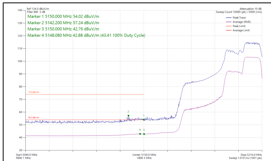
Figure 110 - 802.11ax HE40, RU 106-56, SISO, Core 1 - 5190 MHz Band Edge Frequency 5150 MHz
