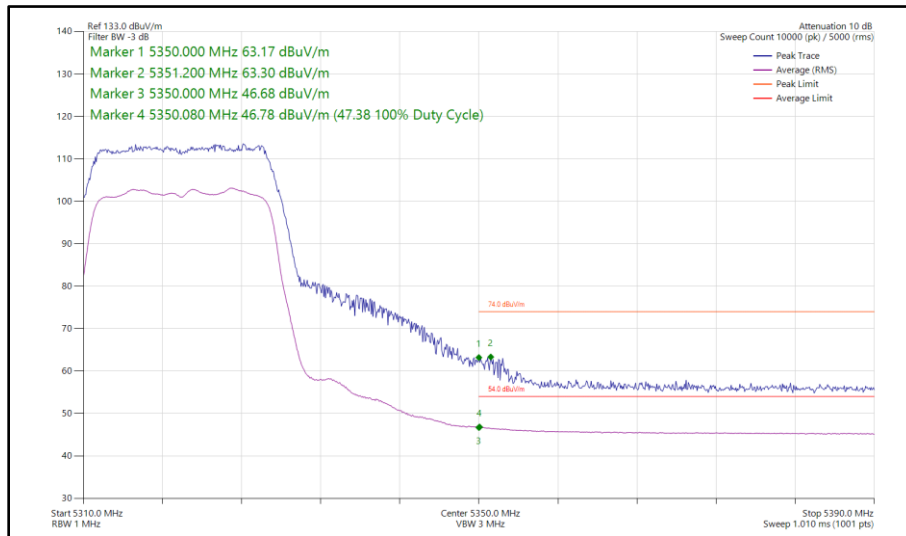
Figure 72 - 802.11n HT20, SDM, Core 0-1 - 5320 MHz Band Edge Frequency 5350 MHz
