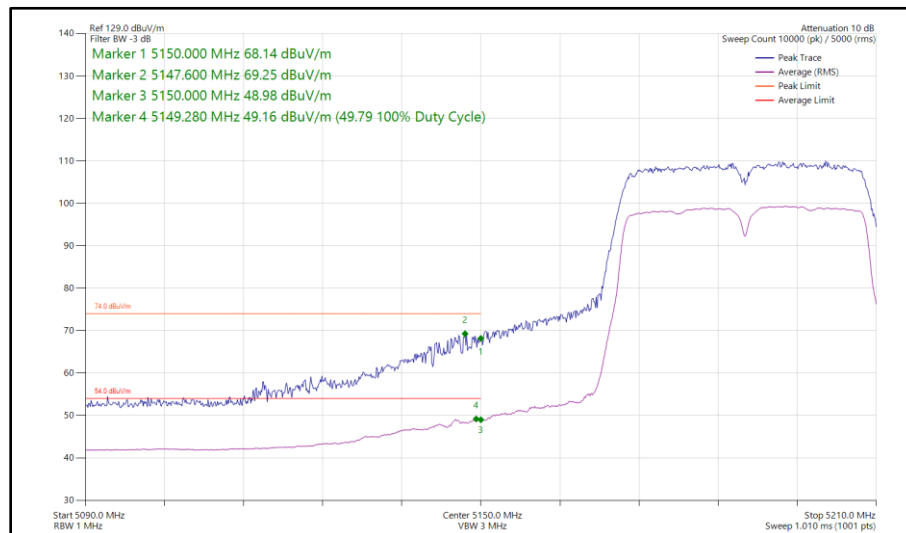
Figure 107 - 802.11n HT40, SISO, Core 1 - 5190 MHz Band Edge Frequency 5150 MHz
