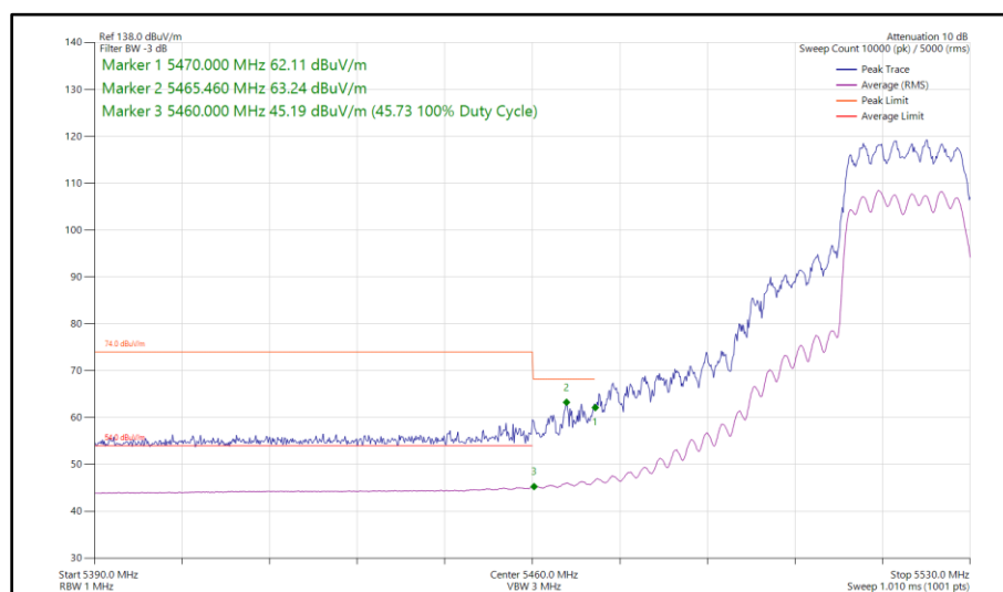
Figure 65 - 802.11ax HE20, SU, CDD, Core 0 - Core 1 - 5520 MHz Band Edge Frequency 5460 MHz
