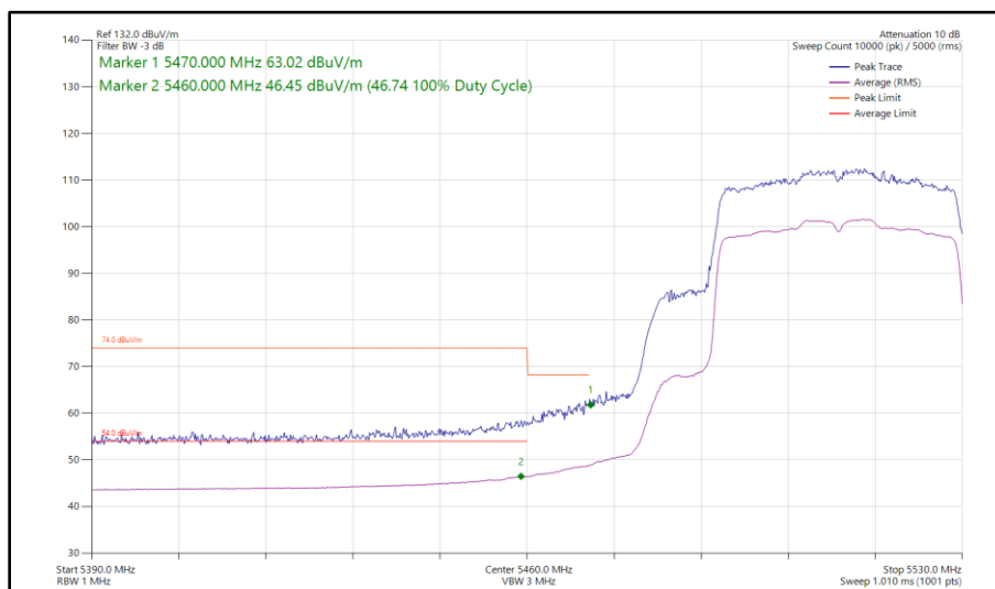
Figure 121 - 802.11ax HE40, SU, SISO, Core 1 - 5510 MHz Band Edge Frequency 5460 MHz
