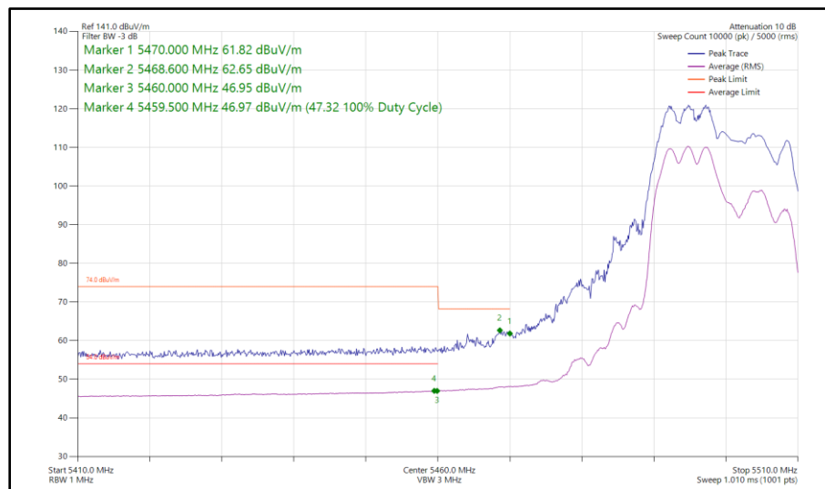
Figure 64 - 802.11ax HE20, RU 106-53, CDD, Core 0 - Core 1 - 5500 MHz Band Edge Frequency 5460 MHz
