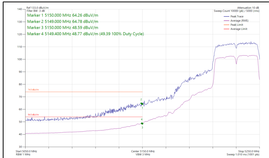
Figure 108 - 802.11n HT40, SISO, Core 1 - 5230 MHz Band Edge Frequency 5150 MHz
