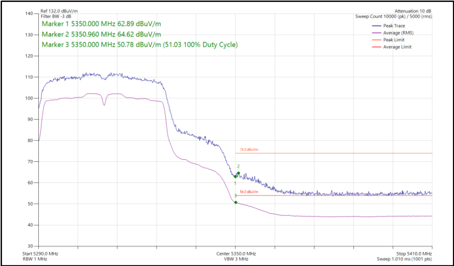
Figure 114 - 802.11n HT40, SISO, Core 1 - 5310 MHz Band Edge Frequency 5350 MHz
