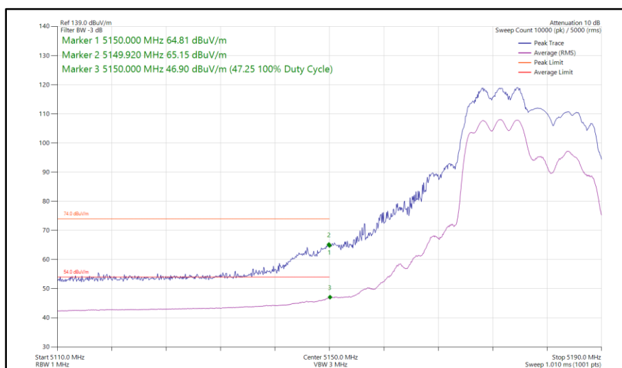
Figure 69 - 802.11ax HE20, RU 106-53, SDM, Core 0 - Core 1 - 5180 MHz Band Edge Frequency 5150 MHz
