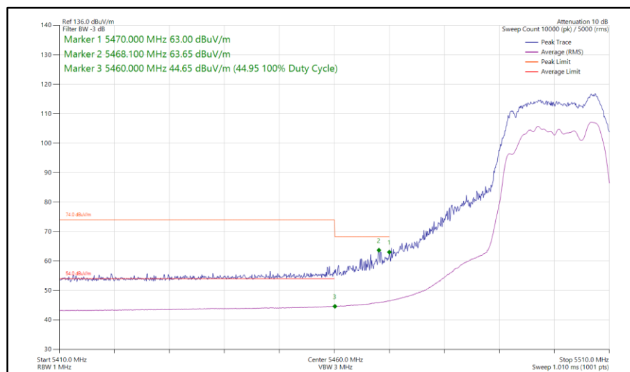
Figure 87 - 802.11ac VHT20, TxBF, Core 0 - Core 1 - 5500 MHz Band Edge Frequency 5460 MHz
