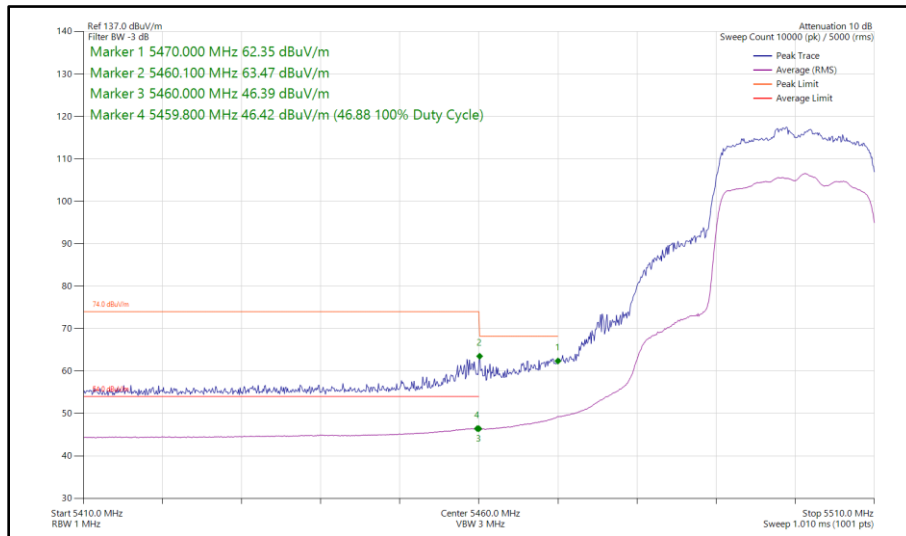
Figure 78 - 802.11ax HE20, SU, SDM, Core 0 - Core 1 - 5500 MHz Band Edge Frequency 5460 MHz
