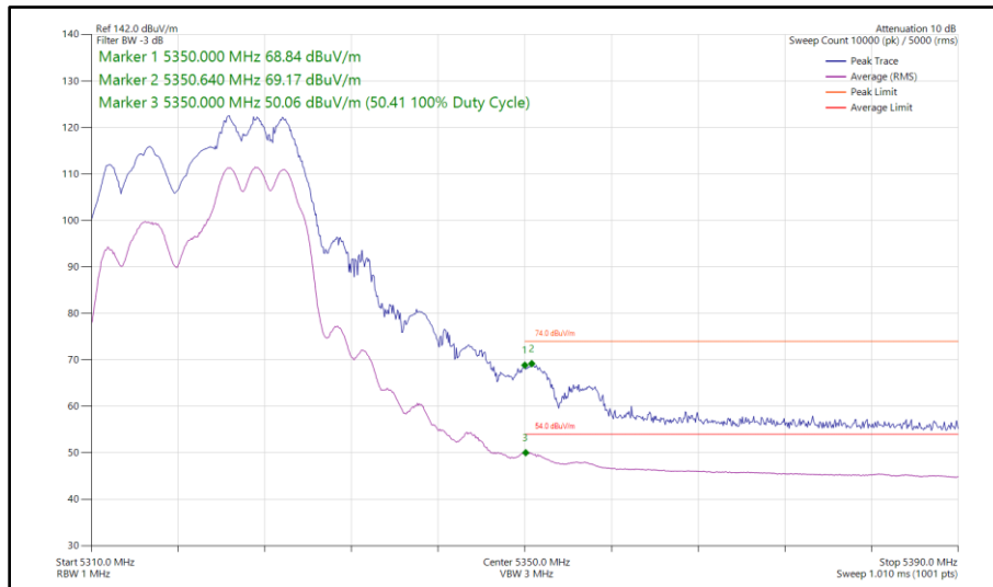
Figure 76 - 802.11ax HE20, RU 106-54, SDM, Core 0 - Core 1 - 5320 MHz Band Edge Frequency 5350 MHz
