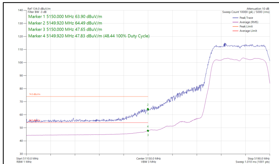
Figure 67 - 802.11n HT20, SDM, Core 0-1 - 5180 MHz Band Edge Frequency 5150 MHz
