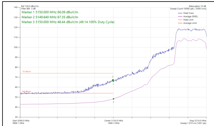
Figure 70 - 802.11ax HE20, SU, SDM, Core 0 - Core 1 - 5200 MHz Band Edge Frequency 5150 MHz
