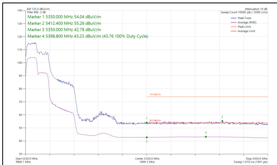
Figure 116 - 802.11ax HE40, RU 106-53, SISO, Core 1 - 5270 MHz Band Edge Frequency 5350 MHz
