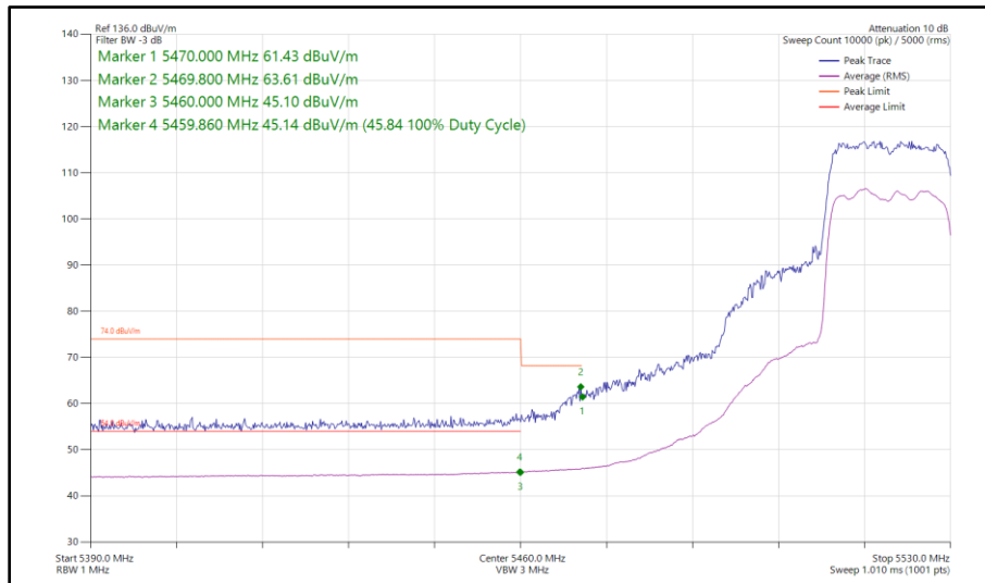
Figure 80 - 802.11ax HE20, SU, SDM, Core 0 - Core 1 - 5520 MHz Band Edge Frequency 5460 MHz
