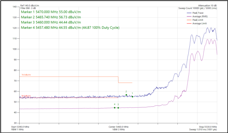
Figure 66 - 802.11ax HE20, RU 106-54, CDD, Core 0 - Core 1 - 5520 MHz Band Edge Frequency 5460 MHz
