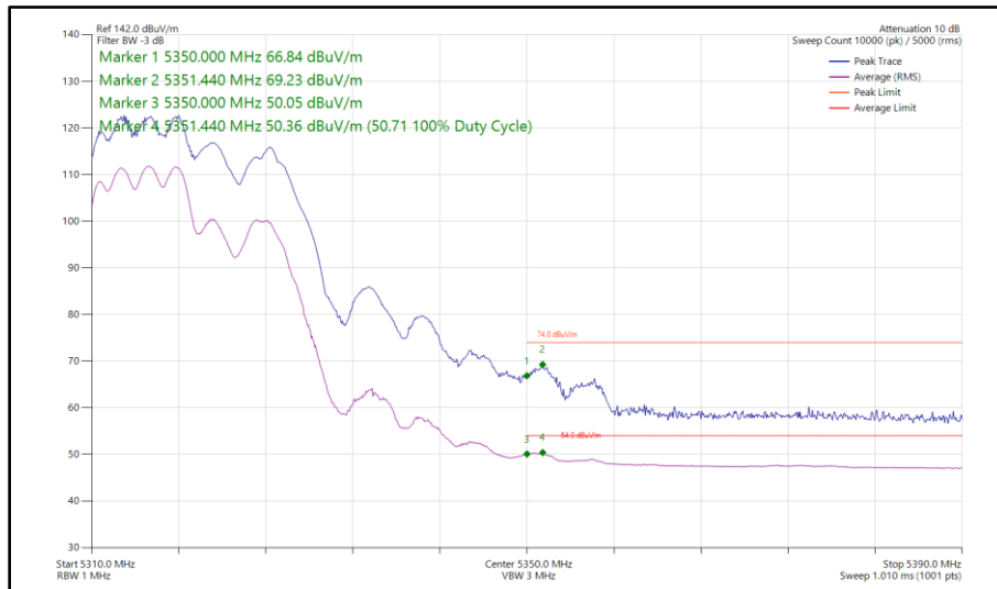
Figure 60 - 802.11ax HE20, RU 106-53, CDD, Core 0 - Core 1 - 5320 MHz Band Edge Frequency 5350 MHz
