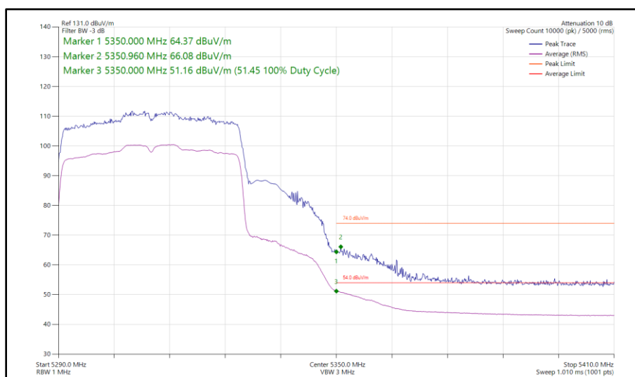
Figure 117 - 802.11ax HE40, SU, SISO, Core 1 - 5310 MHz Band Edge Frequency 5350 MHz
