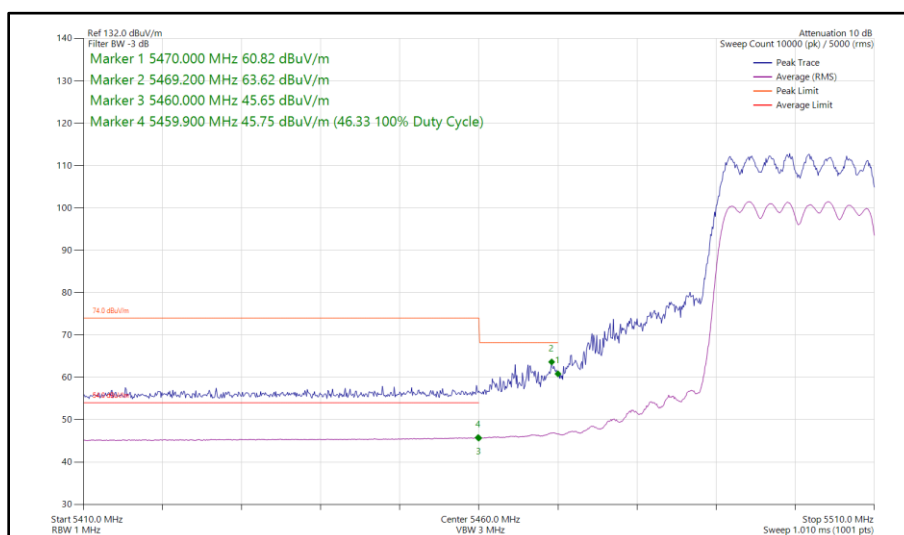
Figure 63 - 802.11ax HE20, SU, CDD, Core 0 - Core 1 - 5500 MHz Band Edge Frequency 5460 MHz
