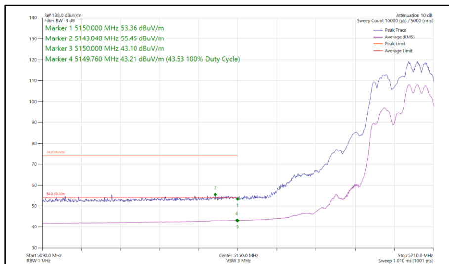
Figure 71 - 802.11ax HE20, RU 106-54, SDM, Core 0 - Core 1 - 5200 MHz Band Edge Frequency 5150 MHz
