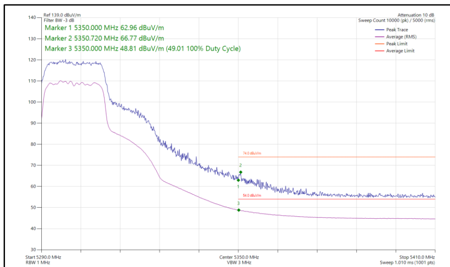
Figure 85 - 802.11ac VHT20, TxBF, Core 0 - Core 1 - 5300 MHz Band Edge Frequency 5350 MHz
