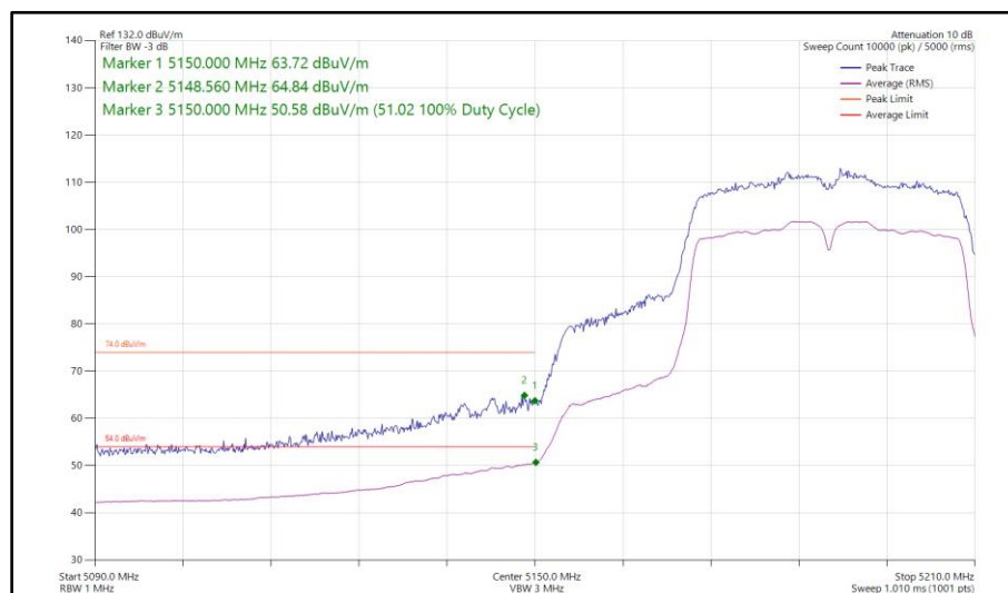
Figure 89 - 802.11n HT40, SISO, Core 0 - 5190 MHz Band Edge Frequency 5150 MHz
