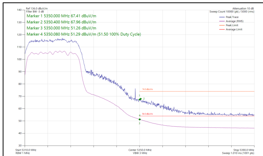
Figure 86 - 802.11ac VHT20, TxBF, Core 0 - Core 1 - 5320 MHz Band Edge Frequency 5350 MHz
