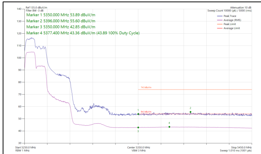
Figure 98 - 802.11ax HE40, RU 106-53, SISO, Core 0 - 5270 MHz Band Edge Frequency 5350 MHz
