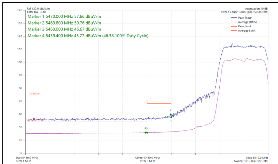
Figure 77 - 802.11n HT20, SDM, Core 0-1 - 5500 MHz Band Edge Frequency 5460 MHz
