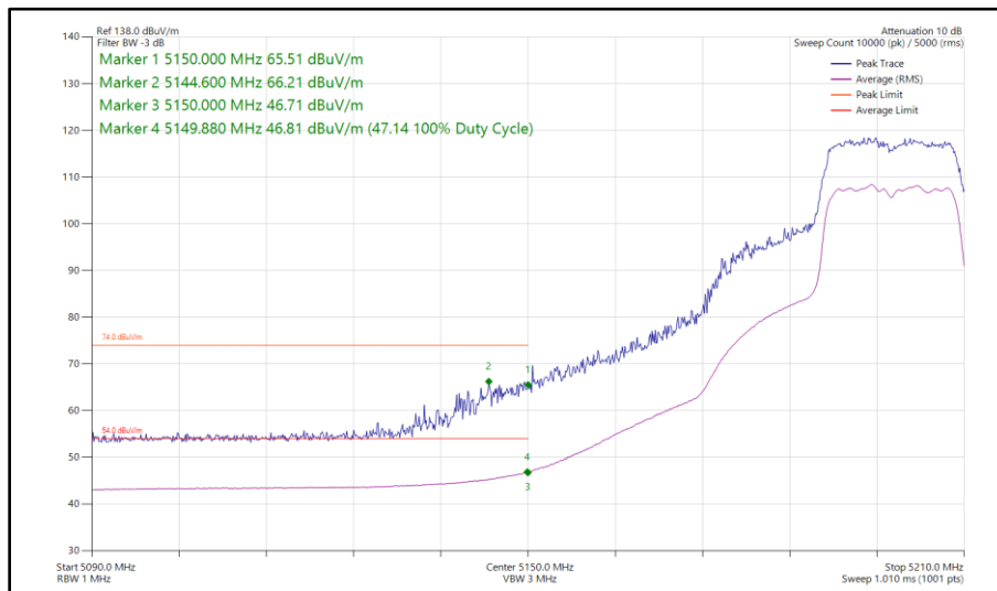
Figure 84 - 802.11ac VHT20, TxBF, Core 0 - Core 1 - 5200 MHz Band Edge Frequency 5150 MHz
