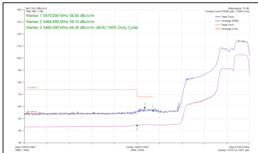
Figure 104 - 802.11ax HE40, RU 106-56, SISO, Core 0 - 5510 MHz Band Edge Frequency 5460 MHz
