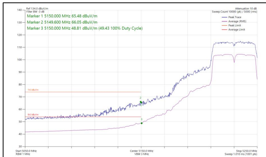
Figure 90 - 802.11n HT40, SISO, Core 0 - 5230 MHz Band Edge Frequency 5150 MHz
