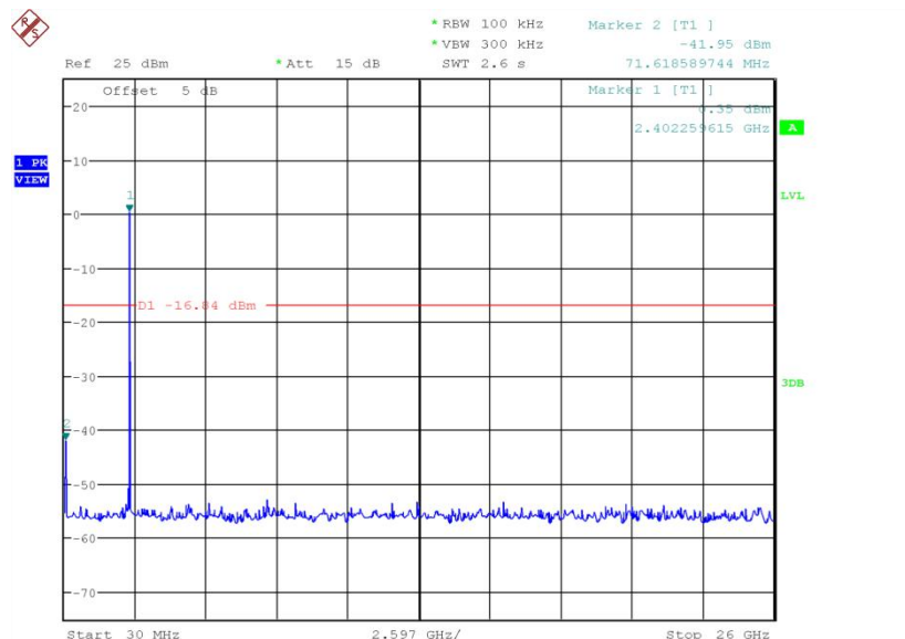
Fig 33. Conducted Spurious Emission (802.11b, Ch1)
