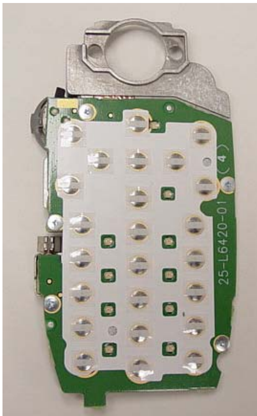
Keyboard & Main Shield
