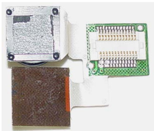
Front & Back Camera Module
