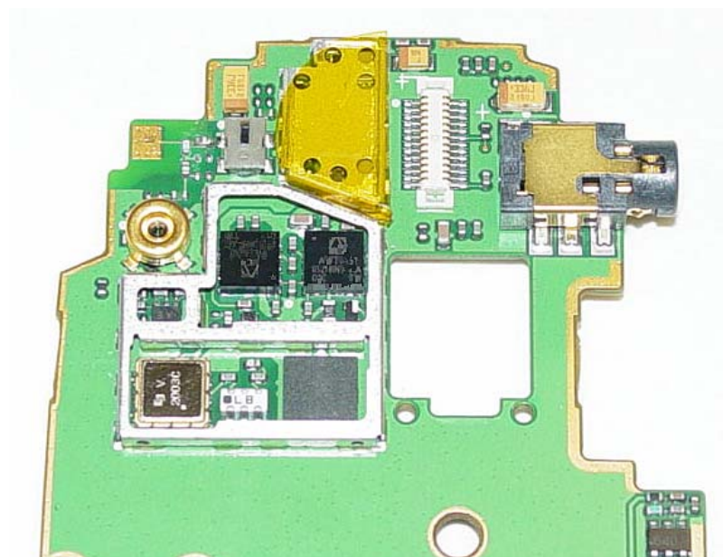
Main PCB_B without Shield &amp; Camera
