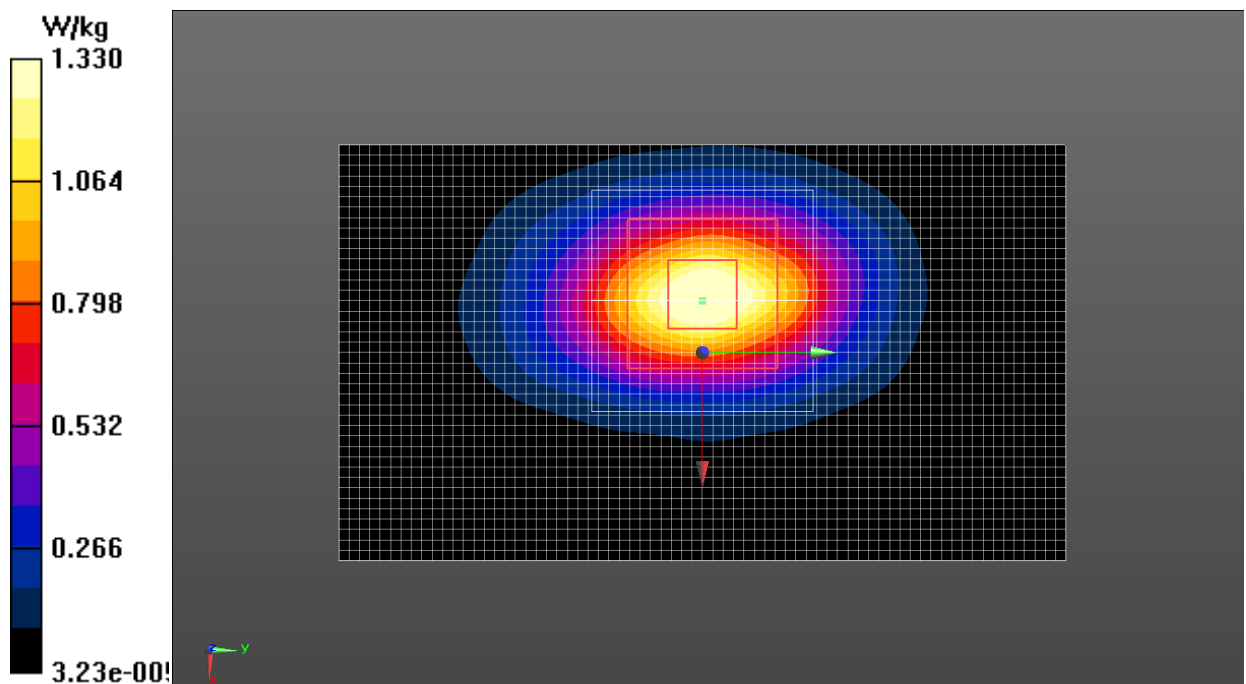
Fig.4 GSM 1900 MHz
