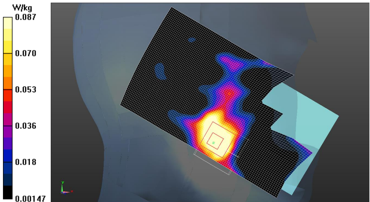
Fig.11 LTE Band 2
