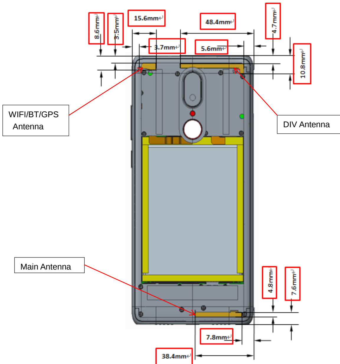
Picture 12.1 Antenna Locations (Back View)
