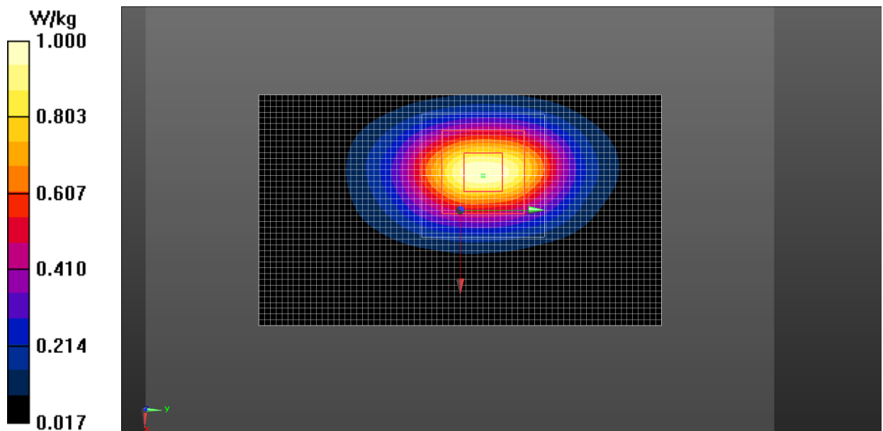
Fig.10 WCDMA 1700
