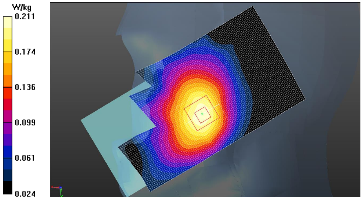
Fig.1 GSM 850MHz
