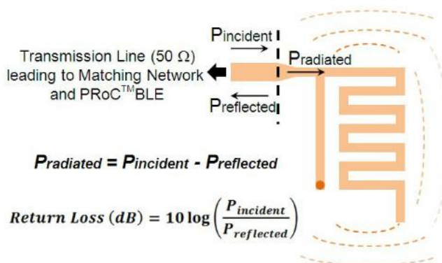
Figure 7. Return Loss
