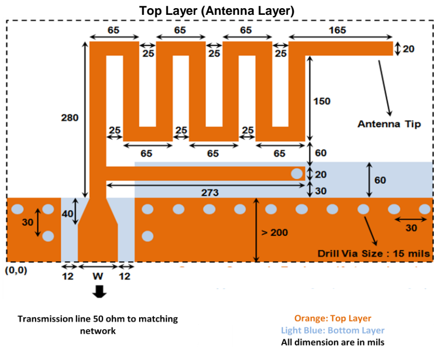
Figure 10. MIFA Layout
