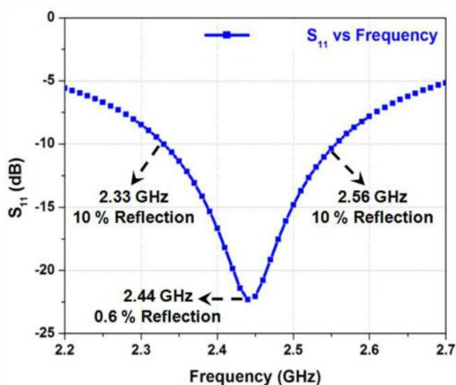
Figure 8. Bandwidth
