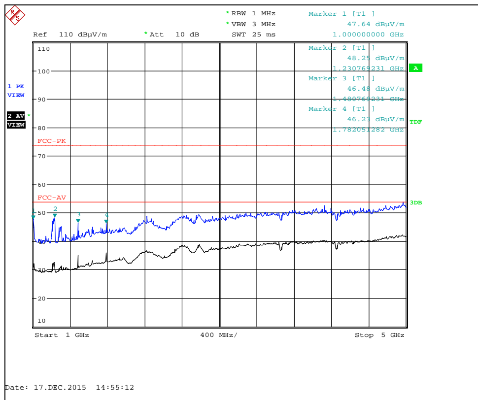
802.11b 1 Mbps Channel 1 : 1 GHz to 5 GHz
