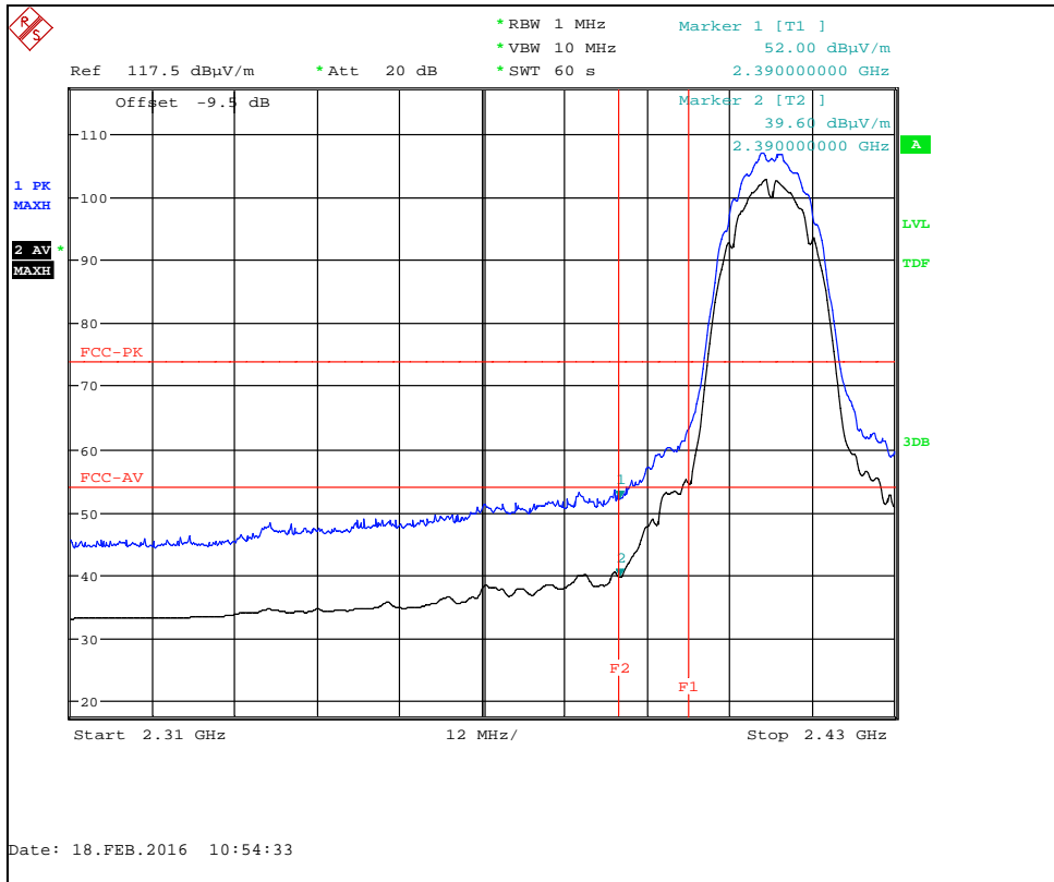
802.11b 1 Mbps Channel 1 : Lower Band Edge
