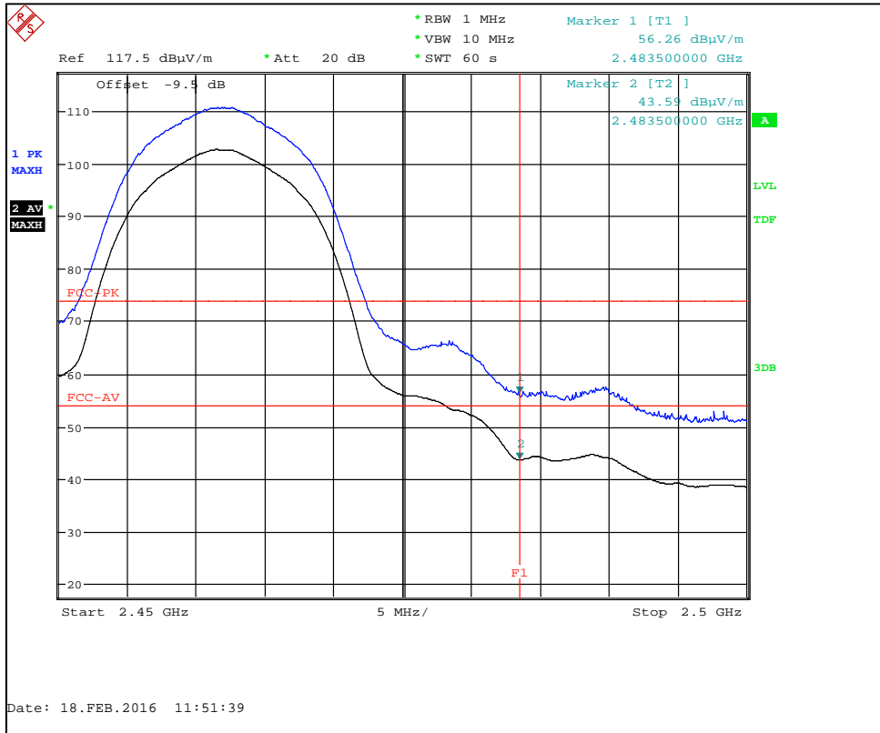
802.11b 11 Mbps Channel 11 : Upper Band Edge
