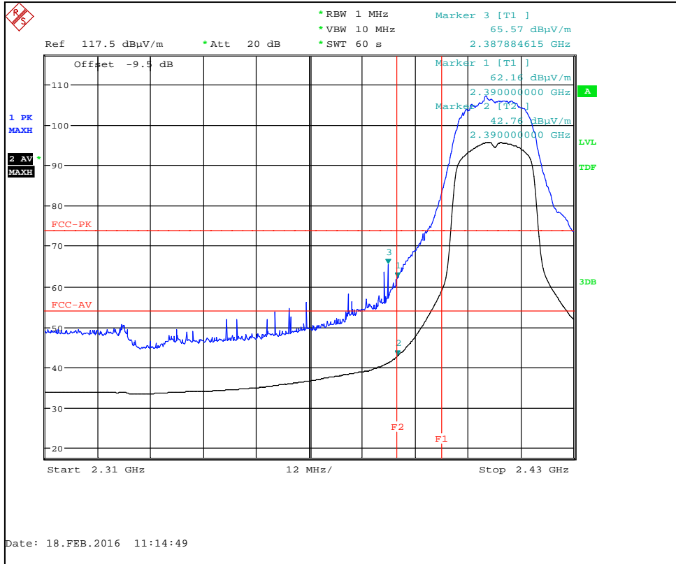
802.11n MCS0 Channel 1 : Lower Band Edge
