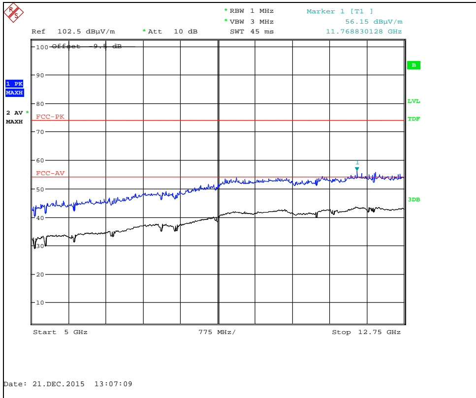
802.11n MCS0 Channel 6 : 5 GHz to 12.75 GHz
