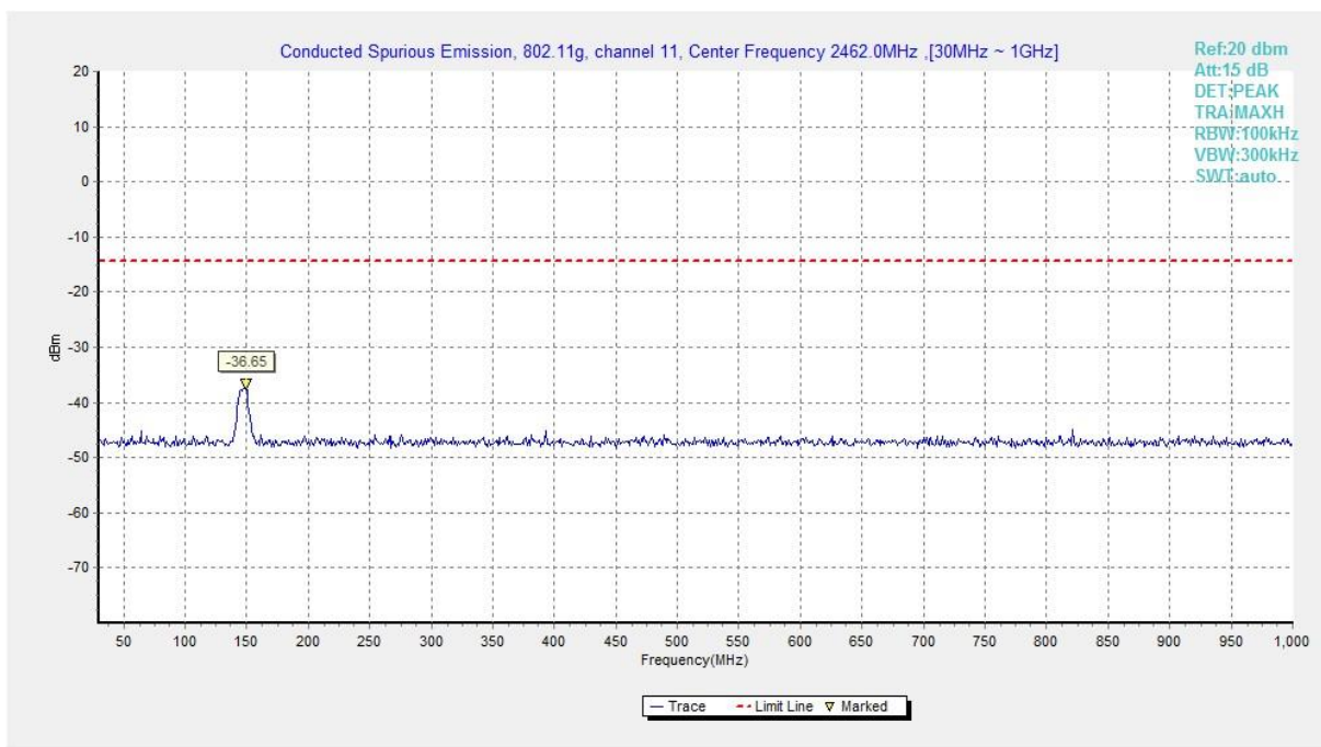
Fig.B.6.1.42 Transmitter Spurious Emission - Conducted (802.11g, Ch11, 30 MHz-1 GHz)
