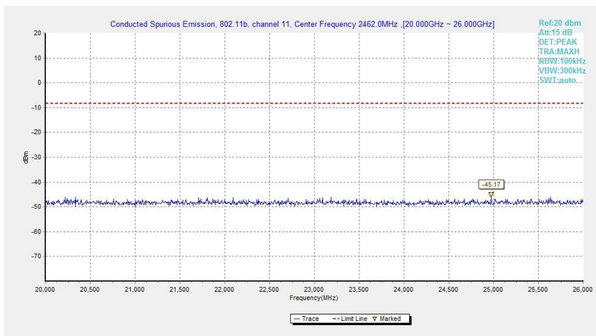
Fig.B.6.1.24 Transmitter Spurious Emission - Conducted (802.11b, Ch11, 20 GHz-26 GHz)
