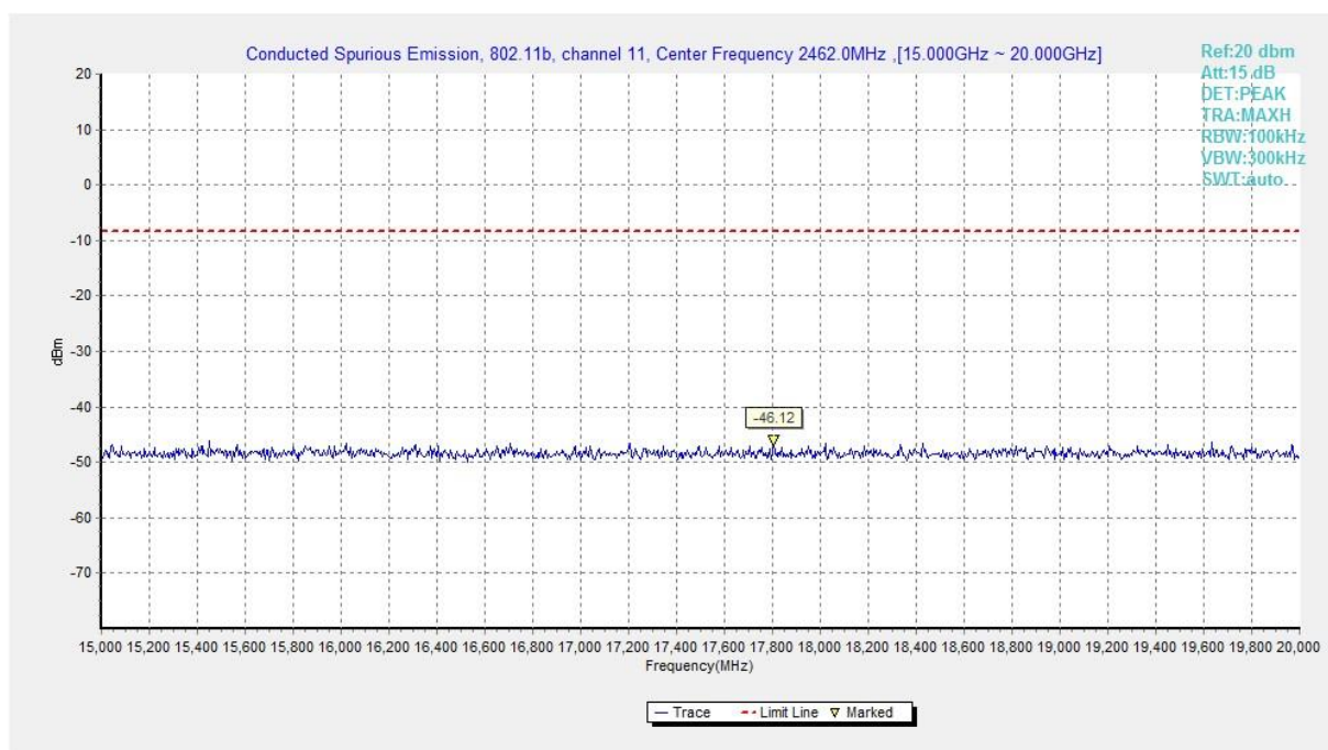
Fig.B.6.1.23 Transmitter Spurious Emission - Conducted (802.11b, Ch11, 15 GHz-20 GHz)
