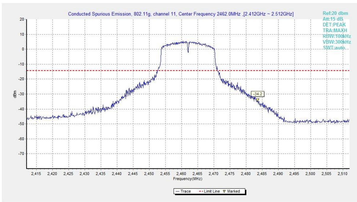
Fig.B.6.1.41 Transmitter Spurious Emission - Conducted (802.11g, Ch11, Center Frequency)
