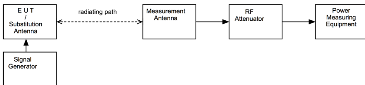
Figure vii Test Setup
