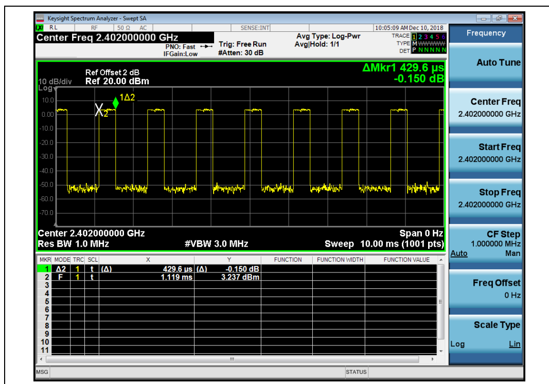
(3DH1_2402M, 8-DQPSK)
