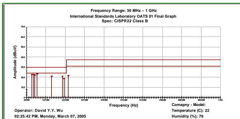
Graph 3.2.2 Open Field Radiated Emissions (Vertical)
