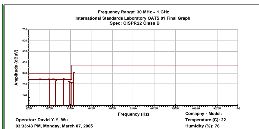
Graph 3.3.1 Open Field Radiated Emissions (Horizontal)
