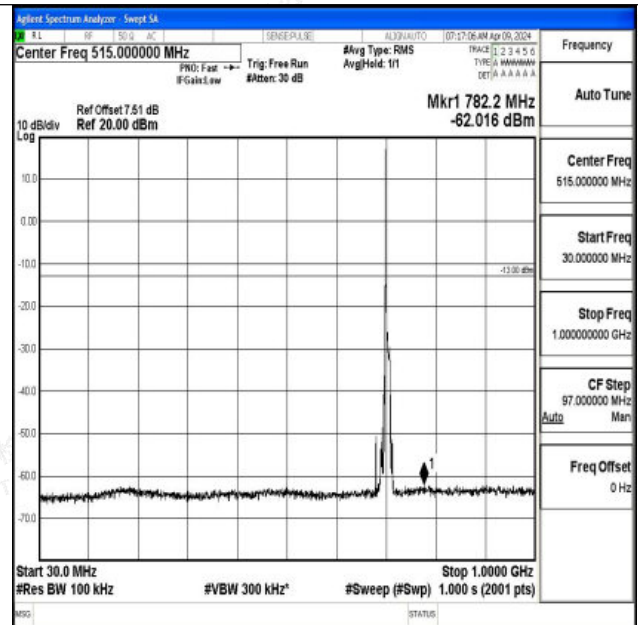
Band12_10MHz_16QAM_23130_1RB#0_30~1000_30~100
