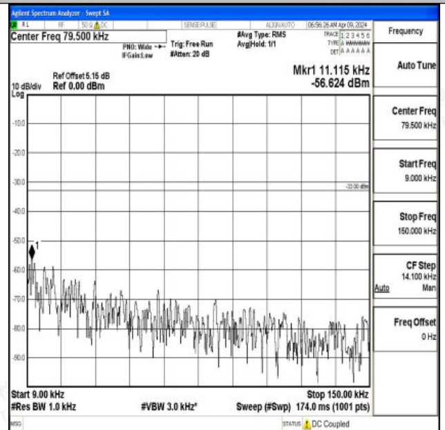
Band12_5MHz_16QAM_23095_1RB#0_0.009~0.15_0.009~0.15
