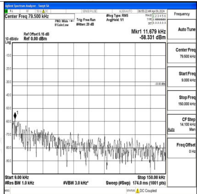
Band12_5MHz_16QAM_23035_1RB#0_0.009~0.15_0.009 ~0.15
