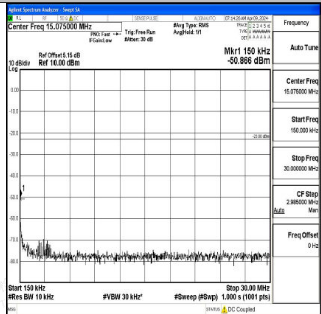
Band12_10MHz_QPSK_23060_1RB#0_0.15~30_0.15~30
