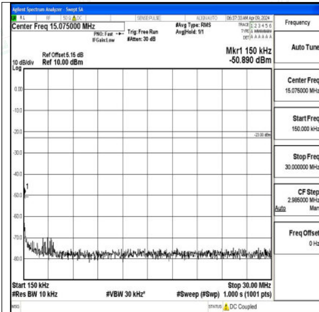
Band12_3MHz_16QAM_23165_1RB#0_0.15~30_0.15~30
