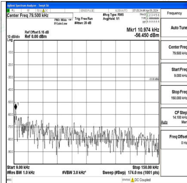
Band12_10MHz_QPSK_23095_1RB#0_0.009~0.15_0.009 ~0.15
