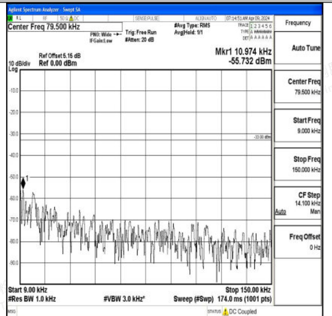
Band12_10MHz_16QAM_23060_1RB#0_0.009~0.15_0.009~0.15
