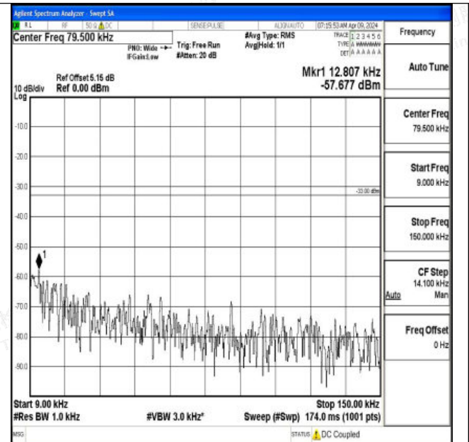
Band12_10MHz_16QAM_23095_1RB#0_0.009~0.15_0.009 ~0.15
