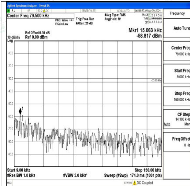
Band12_5MHz_QPSK_23155_1RB#0_0.009~0.15_0.009~0.15
