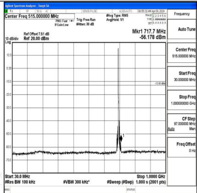
Band12_5MHz_16QAM_23035_1RB#0_30~1000_30~1000
