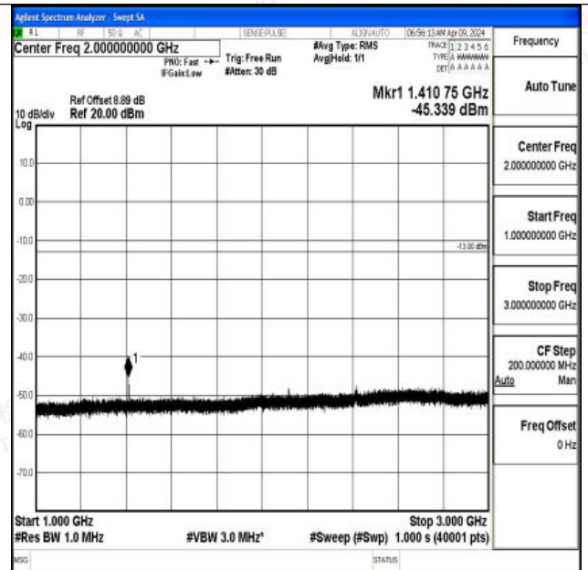
Band12_5MHz_QPSK_23095_1RB#0_1000~3000_1000~3000
