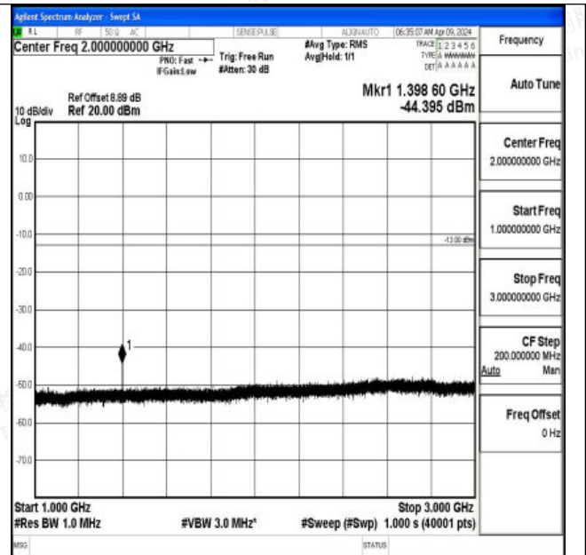
Band12_3MHz_QPSK_23025_1RB#0_1000~3000_1000~3000
