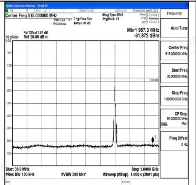
Band12_10MHz_16QAM_23095_1RB#0_30~1000_30~100 0
