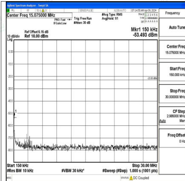
Band12_10MHz_16QAM_23060_1RB#0_0.15~30_0.15~3
