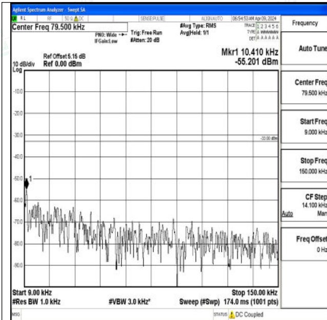
Band12_5MHz_QPSK_23035_1RB#0_0.009~0.15_0.009~0.15
