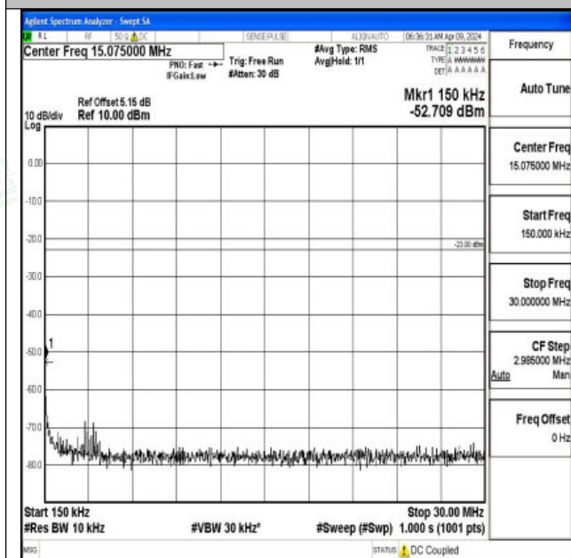
Band12_3MHz_16QAM_23095_1RB#0_0.15~30_0.15~30
