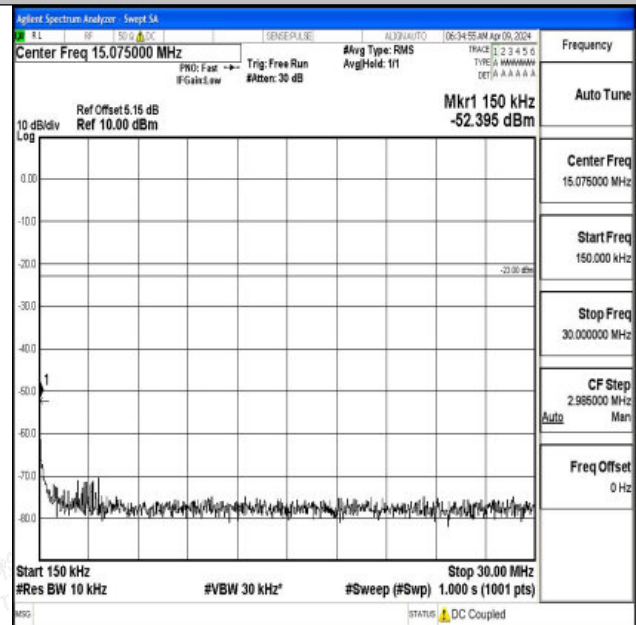
Band12_3MHz_QPSK_23025_1RB#0_0.15~30_0.15~30
