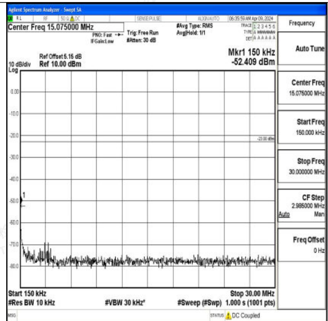
Band12_3MHz_QPSK_23095_1RB#0_0.15~30_0.15~30
