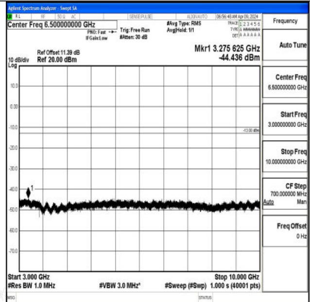
Band12_5MHz_16QAM_23095_1RB#0_3000~10000_3000 ~10000
