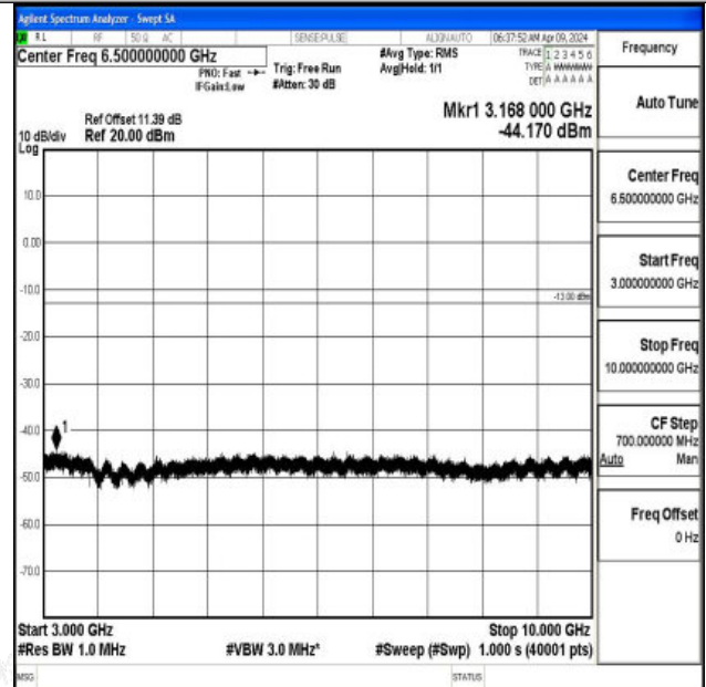
Band12_3MHz_16QAM_23165_1RB#0_3000~10000_3000~10000
