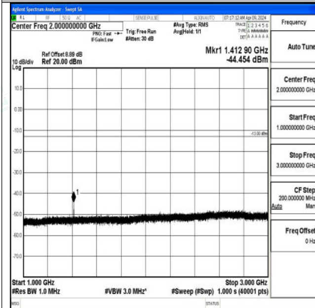
Band12_10MHz_16QAM_23130_1RB#0_1000~3000_100
