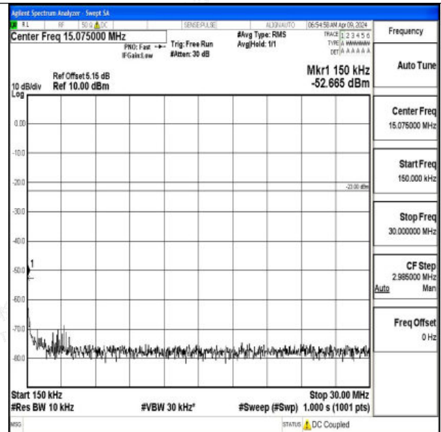
Band12_5MHz_QPSK_23035_1RB#0_0.15~30_0.15~30
