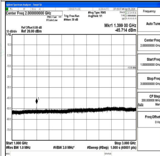
Band12_10MHz_16QAM_23060_1RB#0_1000~3000_100
