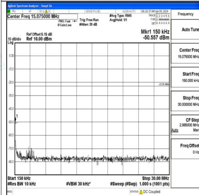
Band12_1.4MHz_16QAM_23173_1RB#0_0.15~30_0.15~3 0
