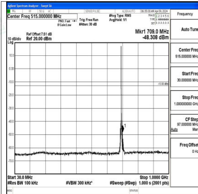
Band12_3MHz_QPSK_23025_1RB#0_30~1000_30~1000
