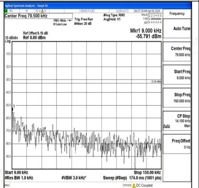
Band12_3MHz_16QAM_23165_1RB#0_0.009~0.15_0.009~0.15
