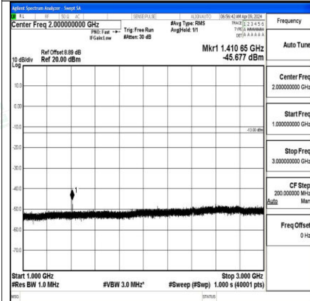
Band12_5MHz_16QAM_23095_1RB#0_1000~3000_1000 ~3000
