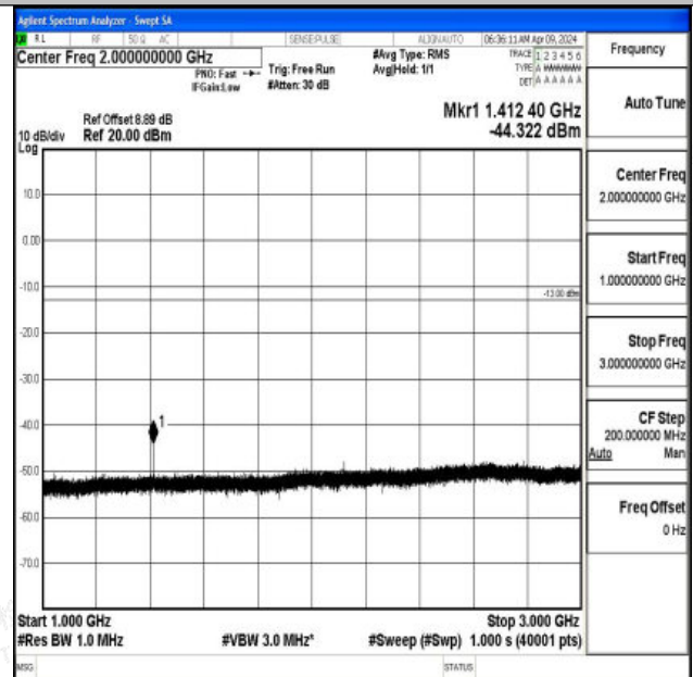
Band12_3MHz_QPSK_23095_1RB#0_1000~3000_1000~3000
