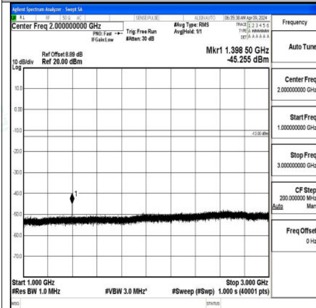
Band12_3MHz_16QAM_23025_1RB#0_1000~3000_1000~3000
