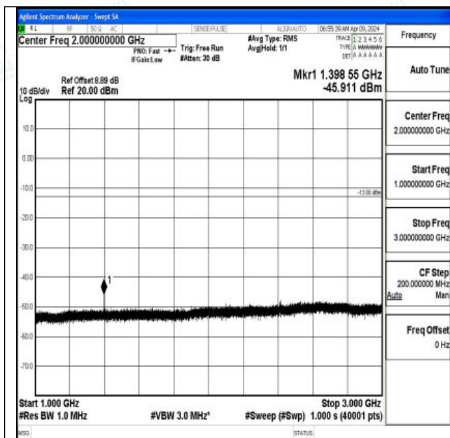
Band12_5MHz_16QAM_23035_1RB#0_1000~3000_1000 ~3000
