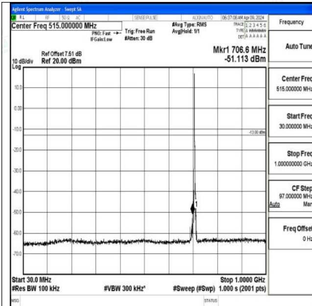
Band12_3MHz_QPSK_23165_1RB#0_30~1000_30~1000
