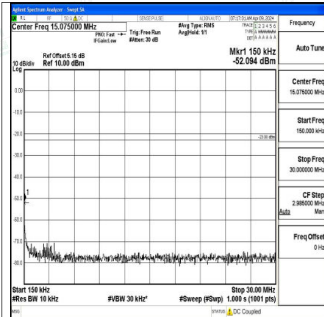
Band12_10MHz_16QAM_23130_1RB#0_0.15~30_0.15~3
