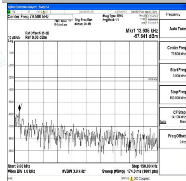
Band12_5MHz_QPSK_23095_1RB#0_0.009~0.15_0.009~0.15
