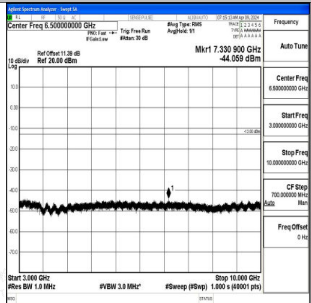
Band12_10MHz_16QAM_23060_1RB#0_3000~10000_300
