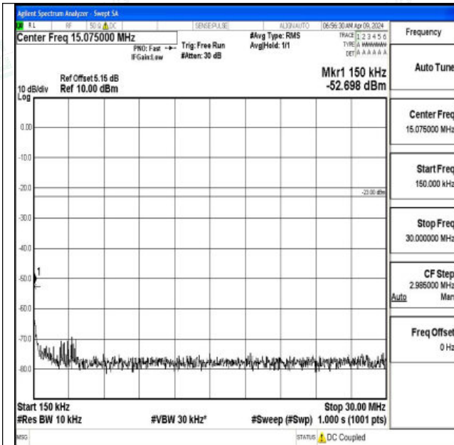
Band12_5MHz_16QAM_23095_1RB#0_0.15~30_0.15~30
