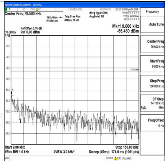
Band12_1.4MHz_16QAM_23173_1RB#0_0.009~0.15_0.00 9~0.15
