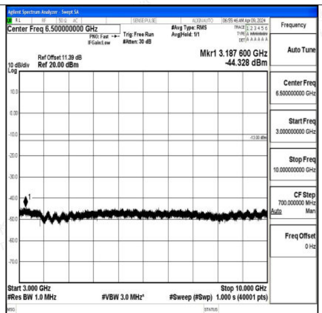
Band12_5MHz_16QAM_23035_1RB#0_3000~10000_3000 ~10000
