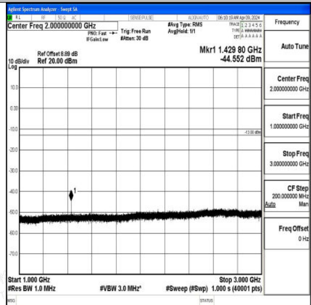
Band12_1.4MHz_QPSK_23173_1RB#0_1000~3000_1000~3000 3000
