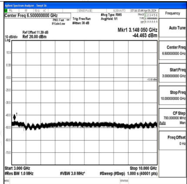
Band12_10MHz_16QAM_23095_1RB#0_3000~10000_300 0~10000
