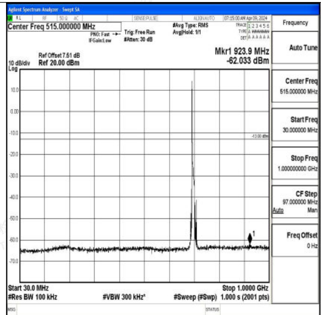
Band12_10MHz_16QAM_23060_1RB#0_30~1000_30~100
