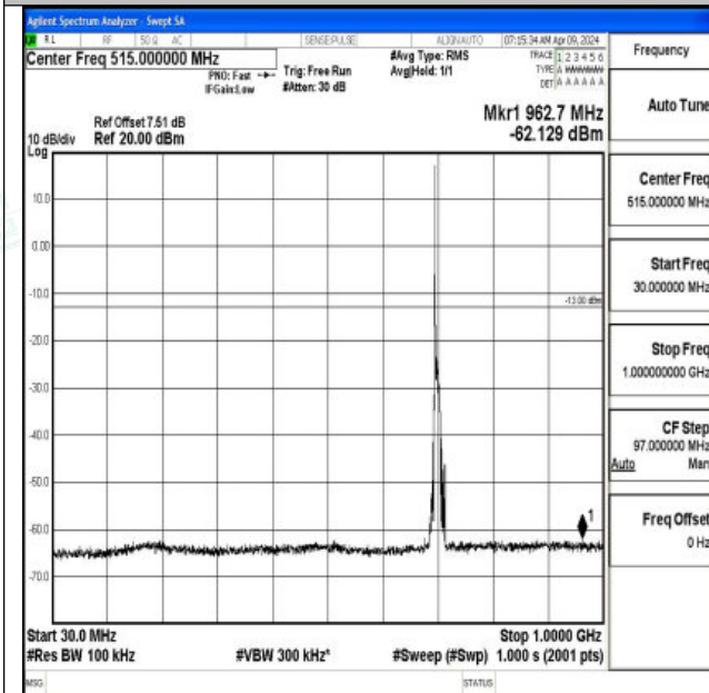
Band12_10MHz_QPSK_23095_1RB#0_30~1000_30~100 0
