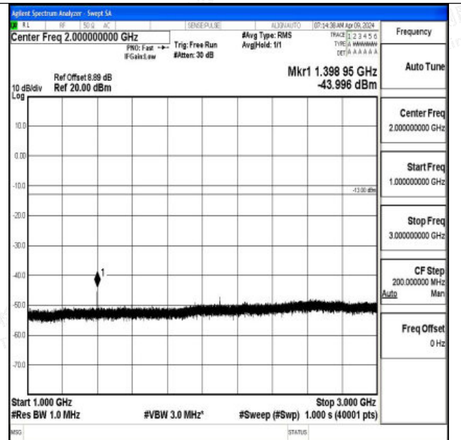
Band12_10MHz_QPSK_23060_1RB#0_1000~3000_1000~3000
