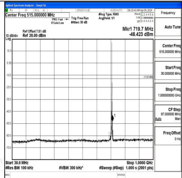
Band12_1.4MHz_16QAM_23173_1RB#0_30~1000_30~10 00
