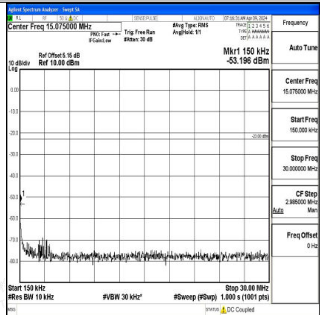
Band12_10MHz_QPSK_23130_1RB#0_0.15~30_0.15~30
