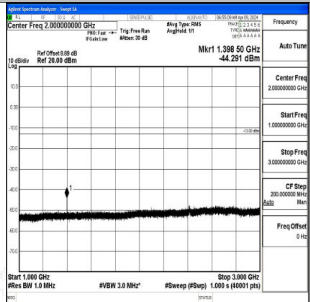
Band12_5MHz_QPSK_23035_1RB#0_1000~3000_1000~3000
