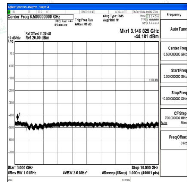
Band12_3MHz_QPSK_23095_1RB#0_3000~10000_3000 ~10000
