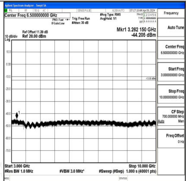
Band12_10MHz_16QAM_23130_1RB#0_3000~10000_300
