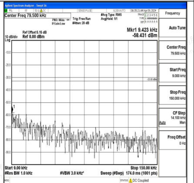
Band12_3MHz_16QAM_23025_1RB#0_0.009~0.15_0.009~0.15
