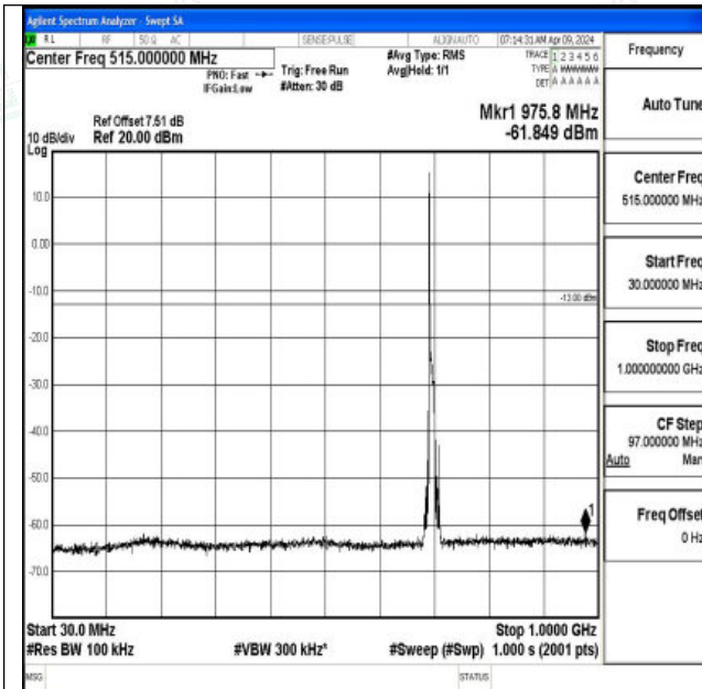
Band12_10MHz_QPSK_23060_1RB#0_30~1000_30~100
