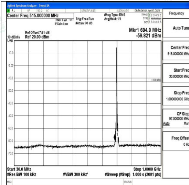
Band12_5MHz_QPSK_23095_1RB#0_30~1000_30~1000
