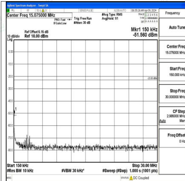
Band12_3MHz_16QAM_23025_1RB#0_0.15~30_0.15~30
