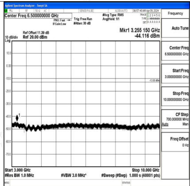
Band12_5MHz_16QAM_23155_1RB#0_3000~10000_3000 ~10000
