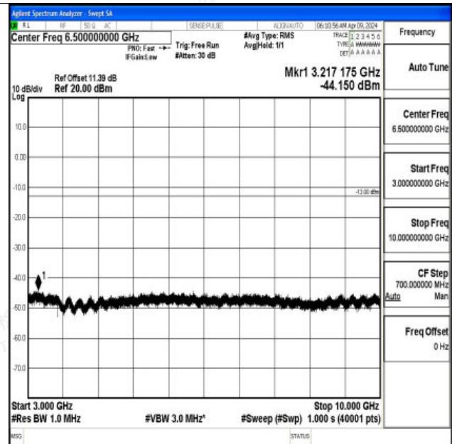
Band12_1.4MHz_16QAM_23173_1RB#0_3000~10000_300 0~10000
