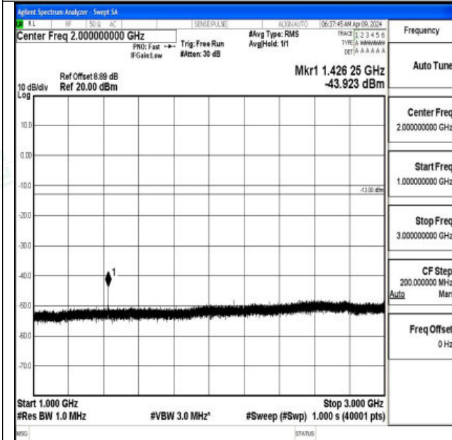
Band12_3MHz_16QAM_23165_1RB#0_1000~3000_1000~3000
