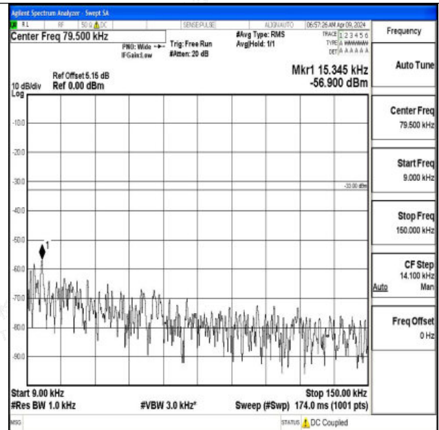
Band12_5MHz_16QAM_23155_1RB#0_0.009~0.15_0.009 ~0.15
