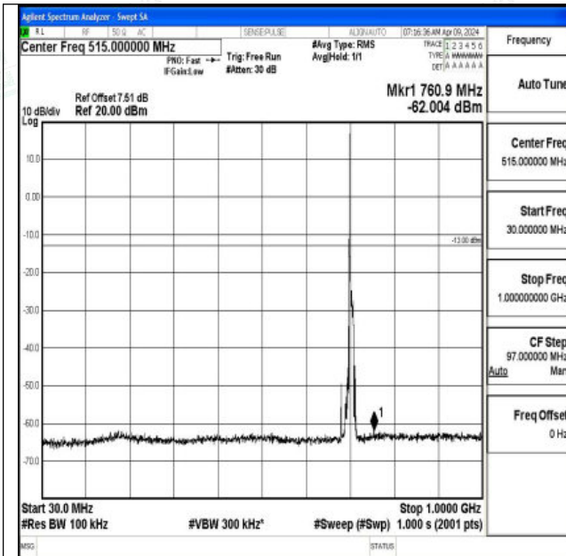
Band12_10MHz_QPSK_23130_1RB#0_30~1000_30~100
