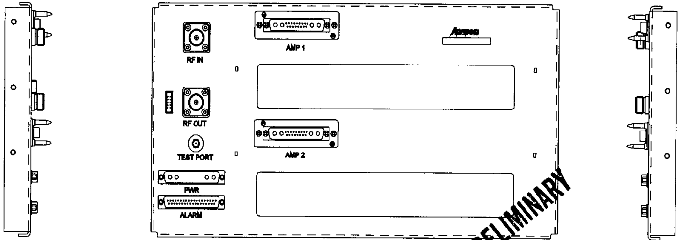
Figure 1-6 BAS Backplane
