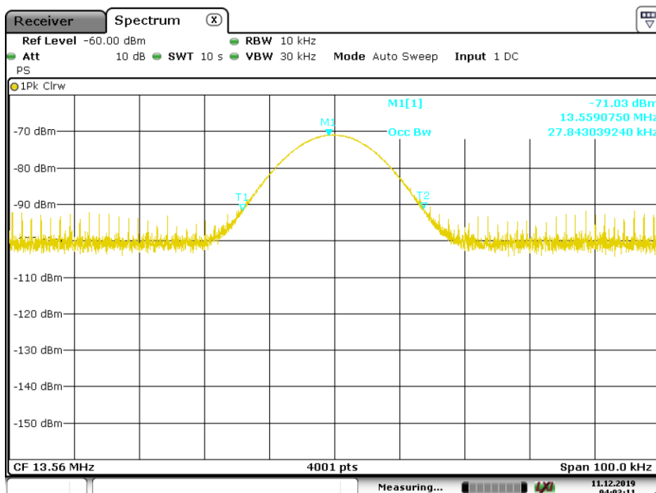
Figure: 99% Bandwidth
