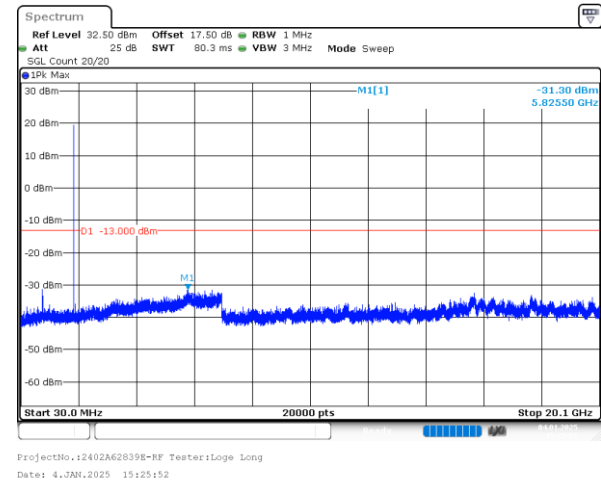
3MHz_High_QPSK_1@0(30MHz~20.1GHz)
