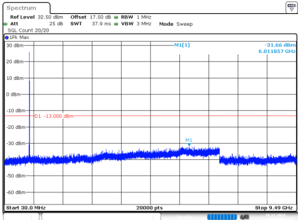
5MHz_Middle_QPSK_1@0(30MHz~9.49GHz)
