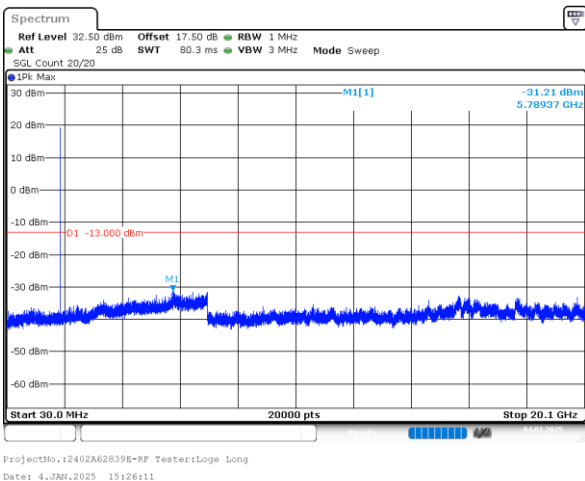
3MHz_Middle_QPSK_1@0(30MHz~20.1GHz)
