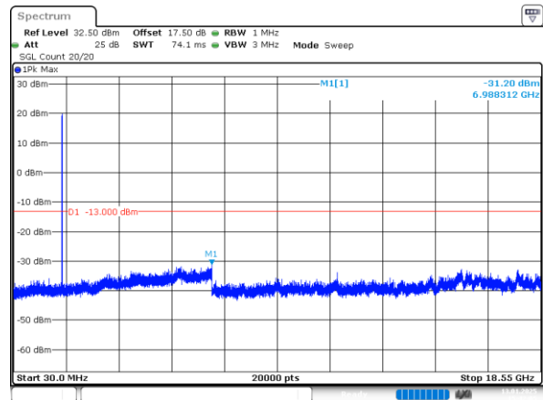
5MHz_Middle_QPSK_1@0(30MHz~18.55GHz)
