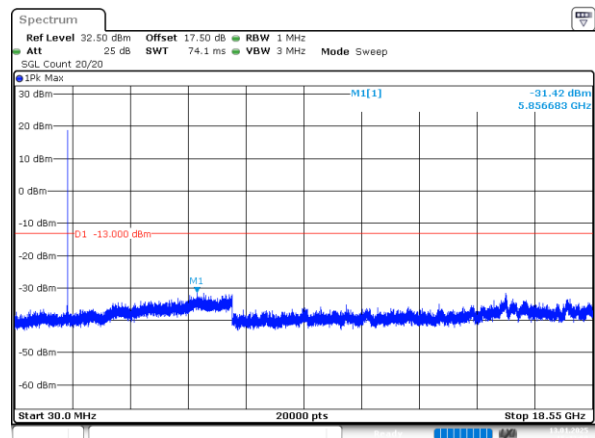
10MHz_Low_QPSK_1@0(30MHz~18.55GHz)
