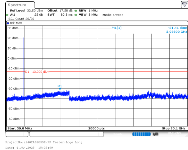
3MHz_Low_QPSK_1@0(30MHz~20.1GHz)
