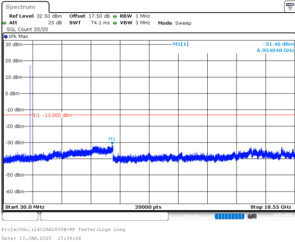
1.4MHz_High_QPSK_1@0(30MHz~18.55GHz)
