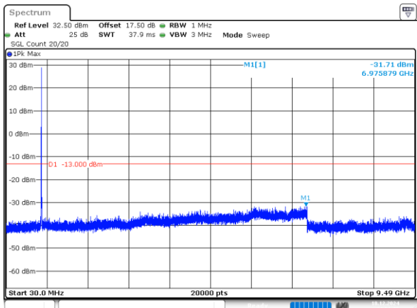
10MHz_High_QPSK_1@0(30MHz~9.49GHz)
