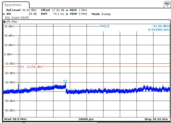
20MHz_Low_QPSK_1@0(30MHz~18.55GHz)
