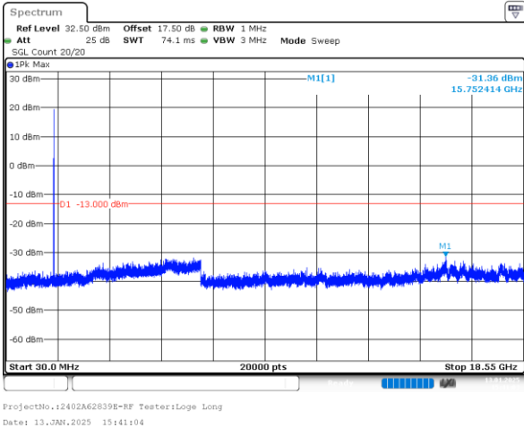
3MHz_Middle_QPSK_1@0(30MHz~18.55GHz)
