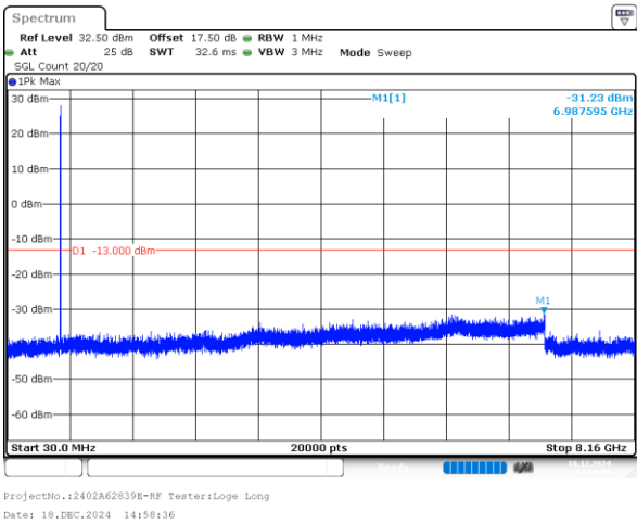
3MHz_Middle_QPSK_1@0(30MHz~8.16GHz)
