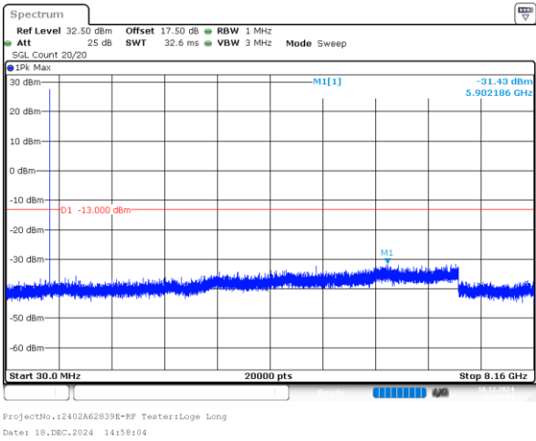
1.4MHz_High_QPSK_1@0(30MHz~8.16GHz)
