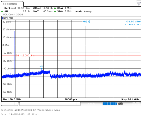
1.4MHz_High_QPSK_1@0(30MHz~20.1GHz)
