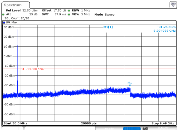
10MHz_Low_QPSK_1@0(30MHz~9.49GHz)
