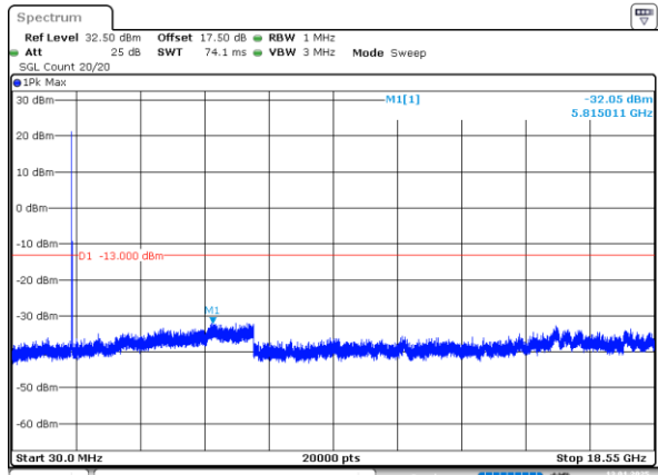
20MHz_High_QPSK_1@0(30MHz~18.55GHz)
