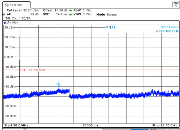
15MHz_Middle_QPSK_1@0(30MHz~18.55GHz)
