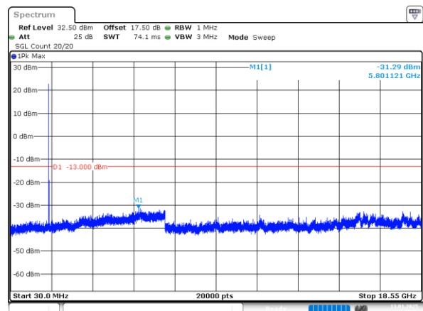
10MHz_High_QPSK_1@0(30MHz~18.55GHz)
