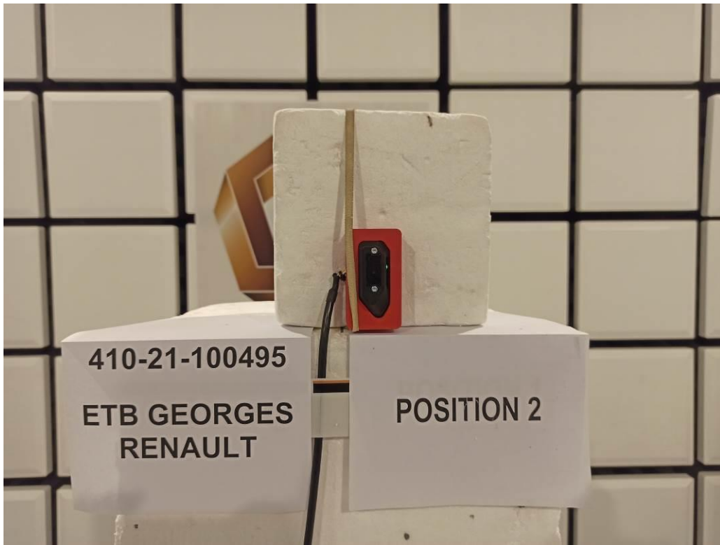
TEST SETUP PHOTO(S) - MAXIMUM PEAK OUTPUT POWER OF UWB DEVICE / POSITION 2
