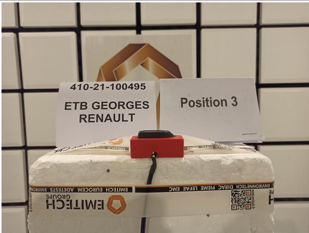
TEST SETUP PHOTO(S) - MAXIMUM PEAK OUTPUT POWER OF UWB DEVICE / POSITION 3
