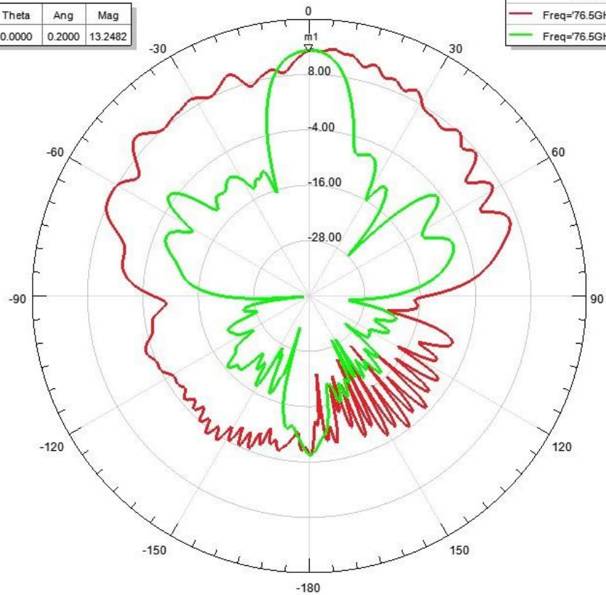
FR552 antenna pattern
